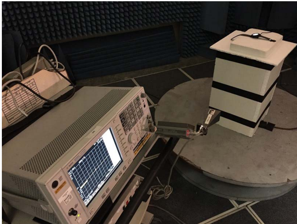
Radiated Emissions to 25 GHz
