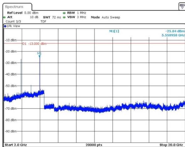
Band2-1.4MHz-QPSK-18607-1RB#0-Range3:2000~20000MHz
