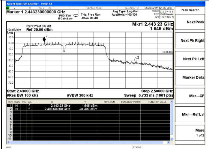
802.11n(HT40)-High channel
