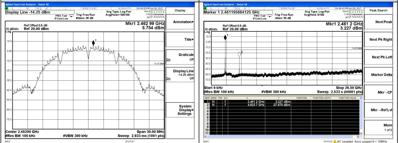
802.11b High channel Reference
