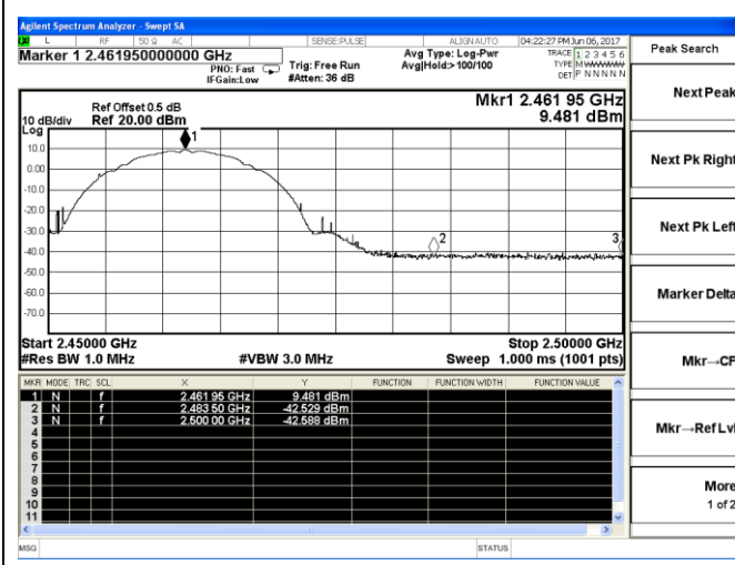
802.11b High channel(Peak)
