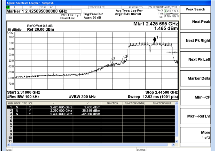
802.11n(HT40)- Low channel
