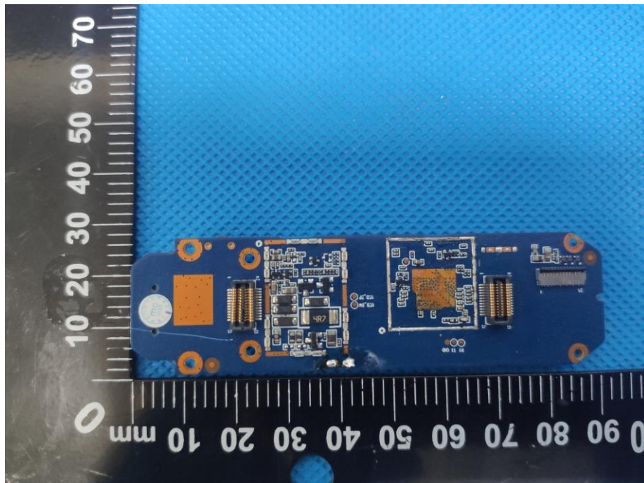
EUT Housing and Board View 22
