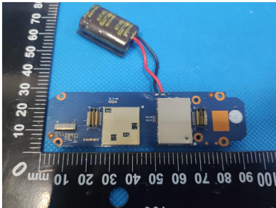
EUT Housing and Board View 19
