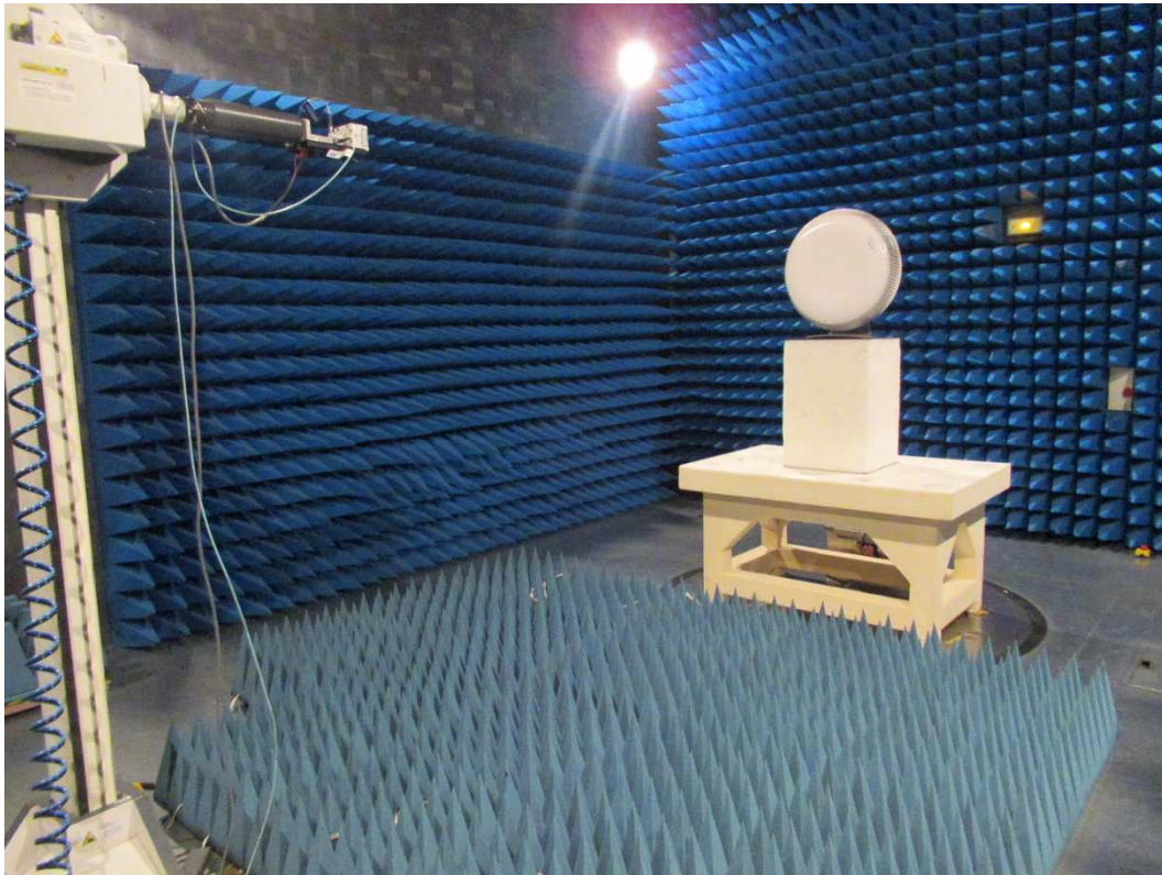
Test Setup Photo – Occupied Bandwidth and Frequency stability
