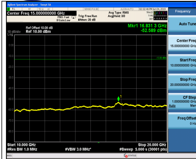
10GHz-20GHz
