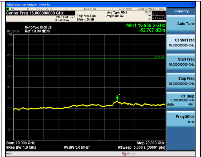
10GHz-20GHz
