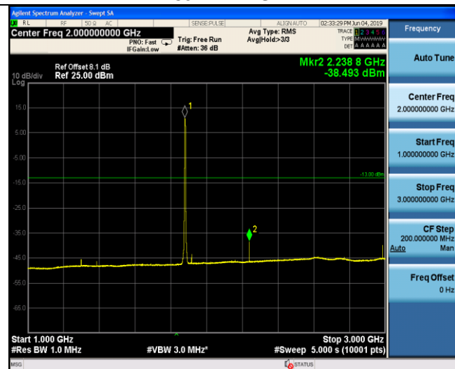
1GHz-3GHz
