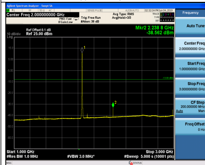
1GHz-3GHz
