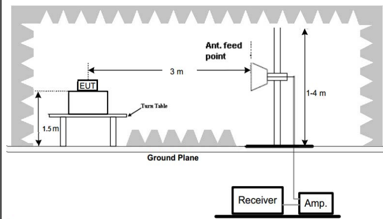
Above 1GHz
