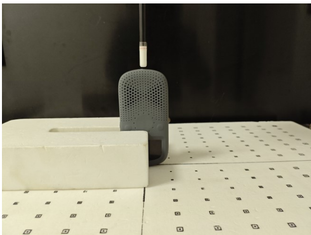
Bottom Side, Test Separation 2 mm
