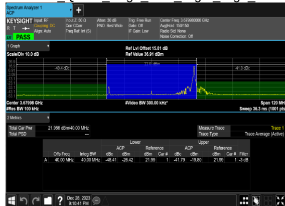
N48(40M)_DFT-s- OFDM QPSK Edge 1RB Right High CH
