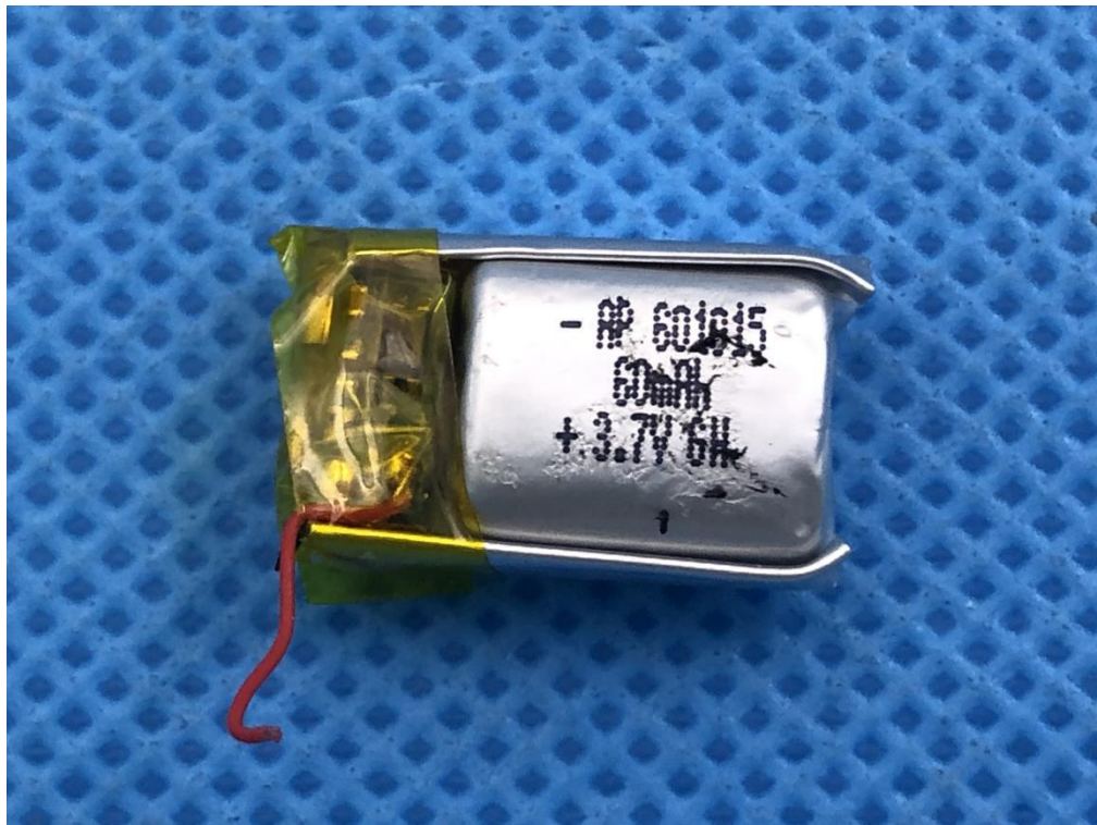
BATTERY VIEW OF EUT (FIGURE 1) left earphone
