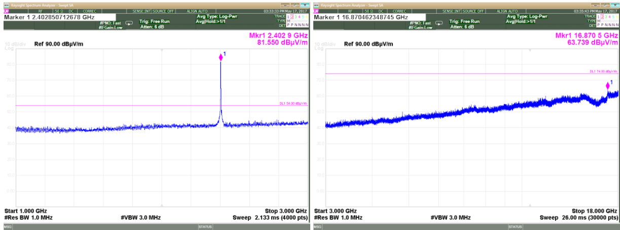
Plot 3.2.10: Radiated Emissions test, Horizontal Polarization, Tx Modulated, Field strength of harmonics, Fc -2402, 1GHz -18GHz
