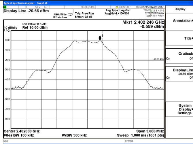
2401 – 2403 MHz
