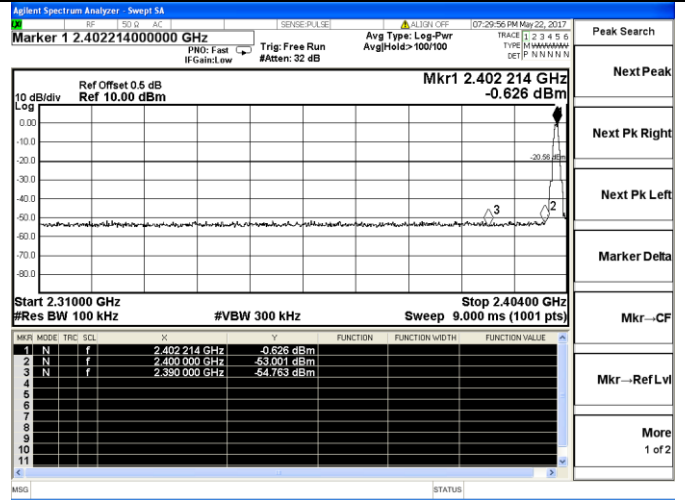
Channel 0 / 2402 MHz
