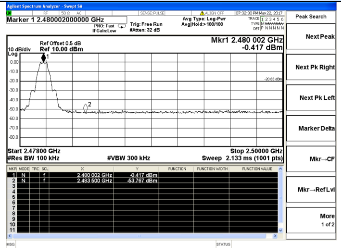
Channel 39 / 2480 MHz
