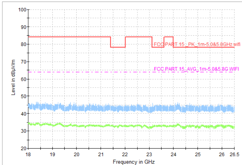
Fig. 90 Transmitter Spurious Emission (All channel, 18GHz~26.5GHz)
