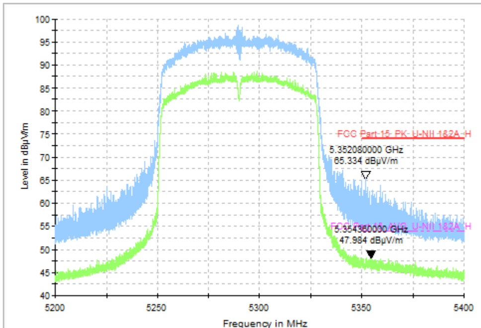
Fig. 62 Band Edges (802.11ac-VHT80, CH58 5290MHz)
