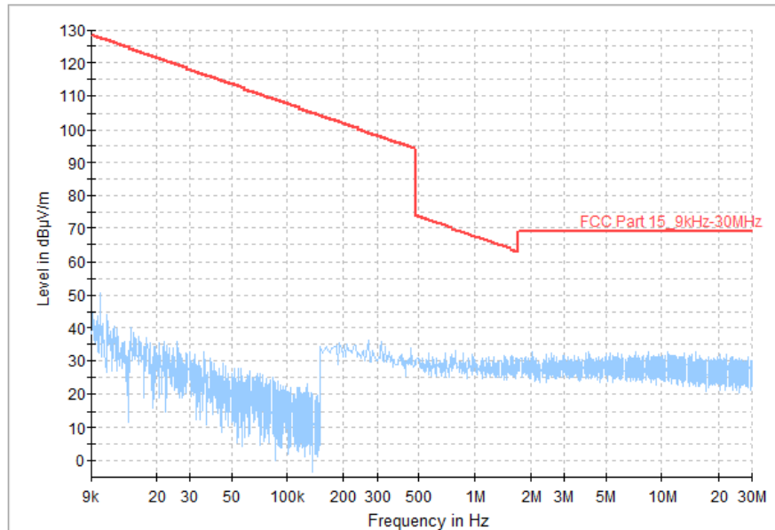
Fig. 48 Radiated Spurious Emission (All Channels, 9kHz ~ 30MHz)
