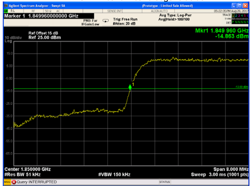
WCDMA band II band edge-left side
