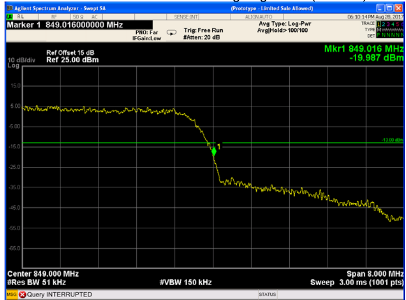
WCDMA band V band edge-right side (HSUPA)
