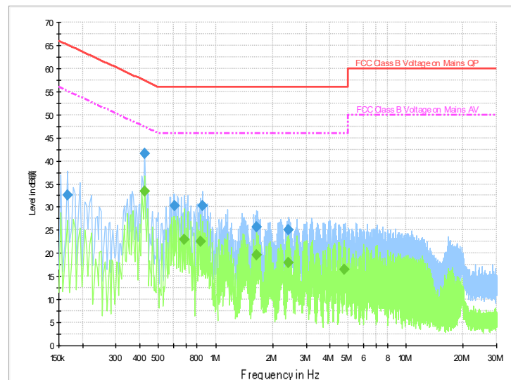
Fig.A.8.1 AC Powerline Conducted Emission-802.11b
