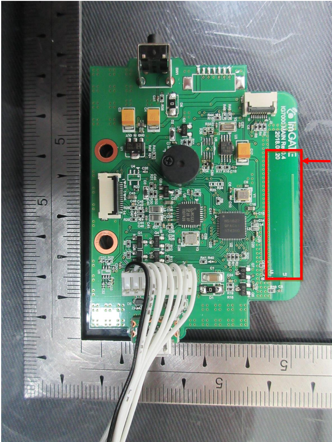
BT Antenna
