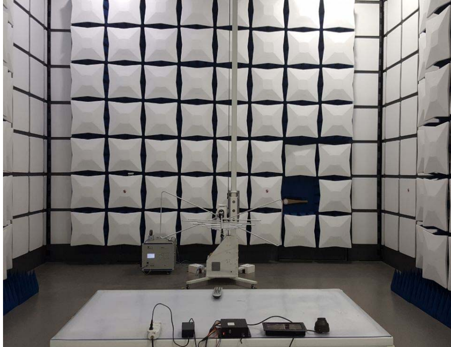
Radiated Emission
