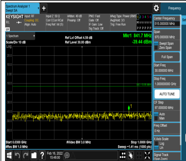
Band66-1.4MHz-QPSK-131979-1RB#0-Range1:30 ~1000MHz
