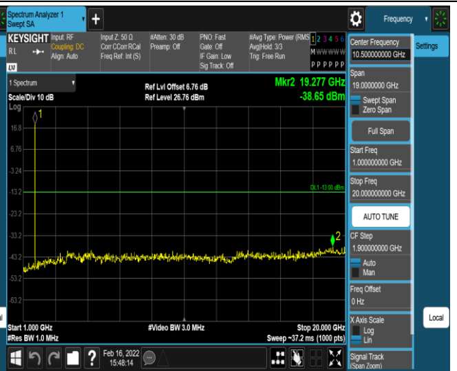
Band66-1.4MHz-QPSK-131979-1RB#0-Range2:1000 ~20000MHz
