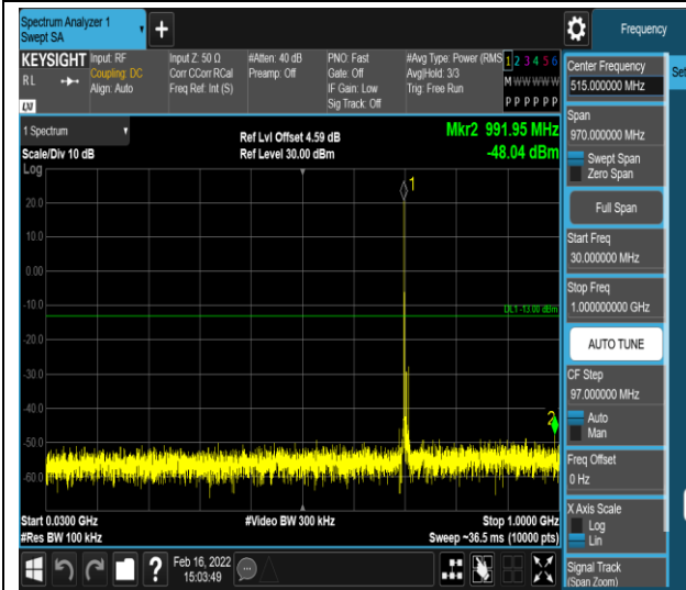
Band66-1.4MHz-QPSK-131979-1RB#0-Range1:30 ~1000MHz
