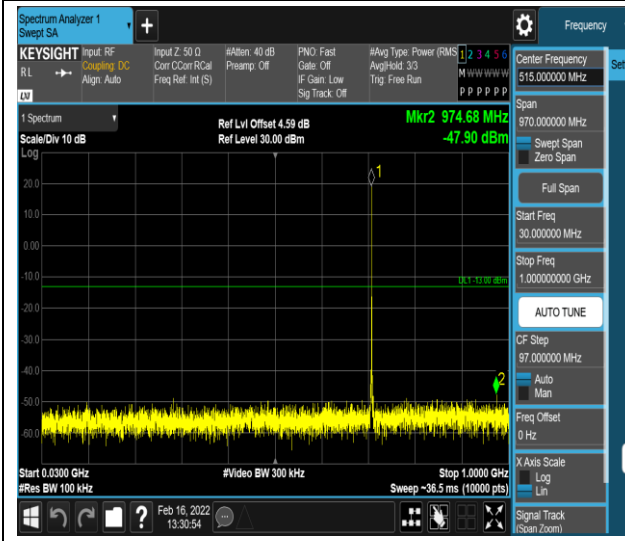
Band12-1.4MHz-QPSK-23173-1RB#0-Range1:30~1000MHz
