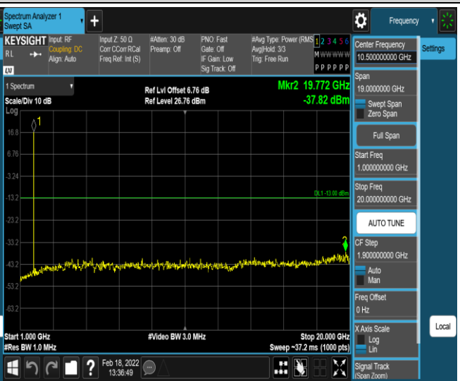
Band66-1.4MHz-16QAM-132665-1RB#0-Range2:100 0~20000MHz
