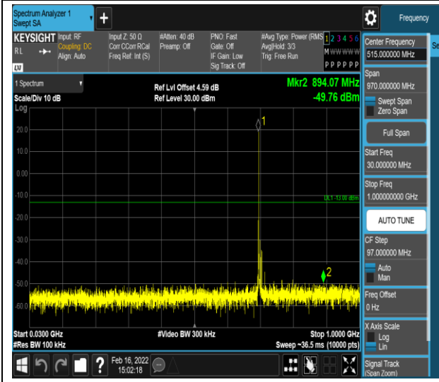
Band12-10MHz-QPSK-23095-1RB#0-Range1:30~1000MHz
