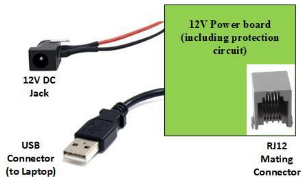
Figure 9: Power Board with DriverI/DCM Setup
