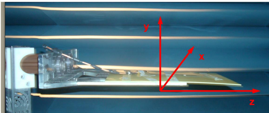
Device tested in AMS-8500 Rectangular test chamber.
