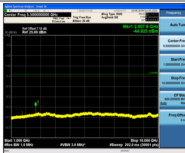
Band5-1.4MHz-QPSK-20525-1-0-Low-1000-10000--44.92-PASS
