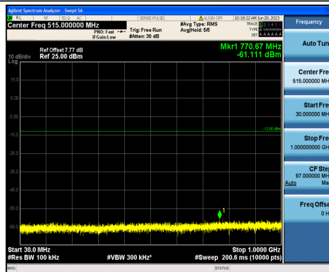
Band4-20MHz-16QAM-20050-1-0-Low-30-1000--61.11-PASS
