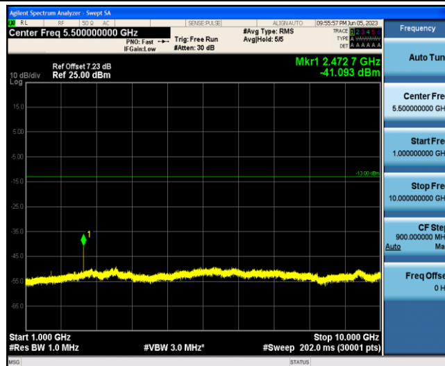
Band5-1.4MHz-QPSK-20407-1-0-Low-1000-10000--41.09-PASS
