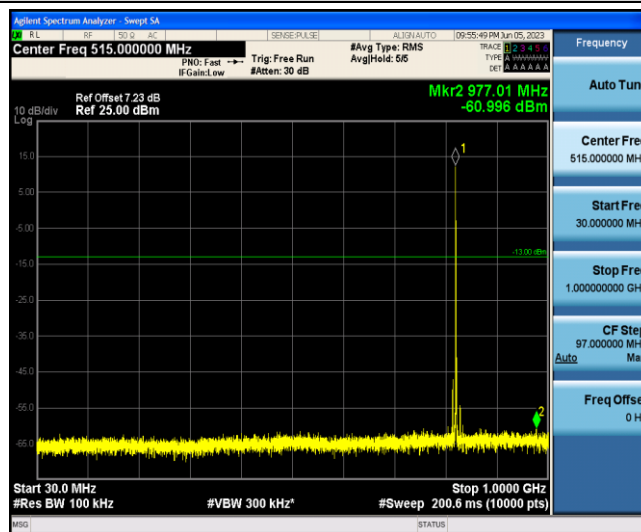
Band5-1.4MHz-QPSK-20407-1-0-Low-30-1000--61-PASS
