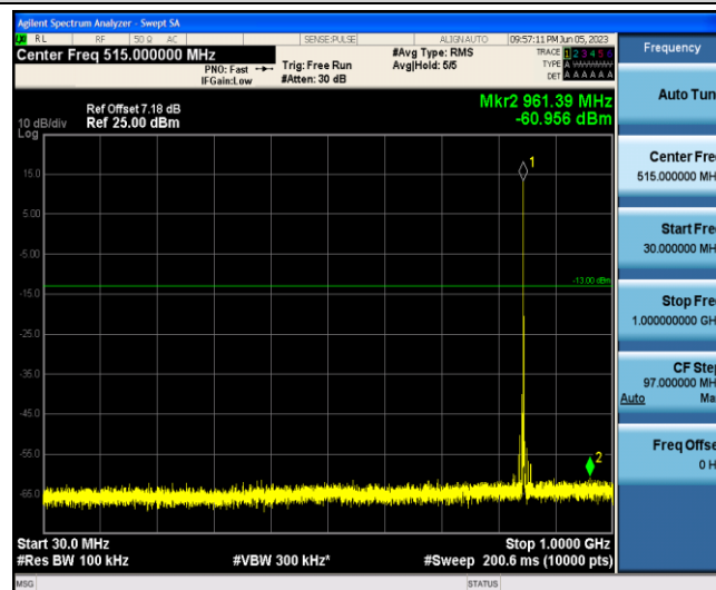
Band5-1.4MHz-QPSK-20643-1-0-Low-30-1000--60.96-PASS
