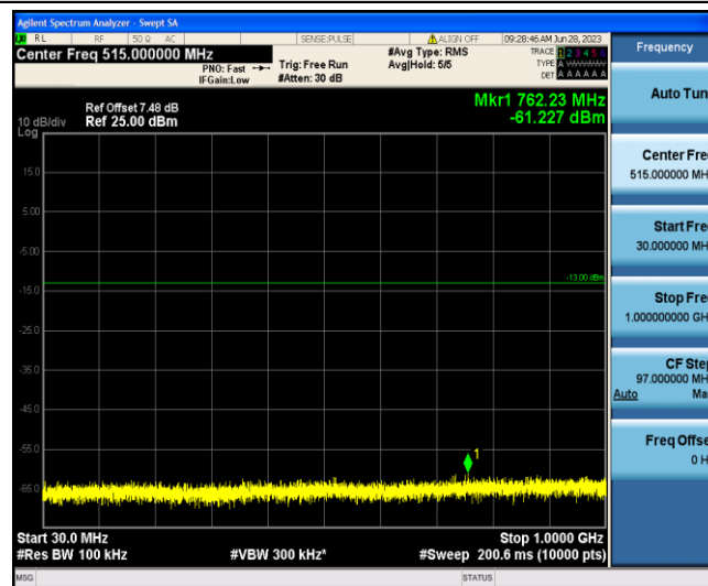
Band4-5MHz-16QAM-20375-1-0-Low-30-1000--61.23-PASS
