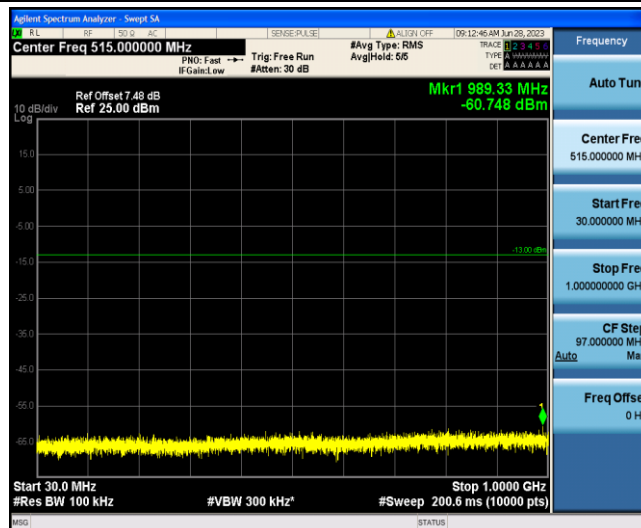
Band4-3MHz-QPSK-20175-1-0-Low-30-1000--60.75-PASS
