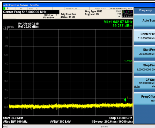
Band2-10MHz-16QAM-18900-1-0-Low-30-1000--59.24-PASS
