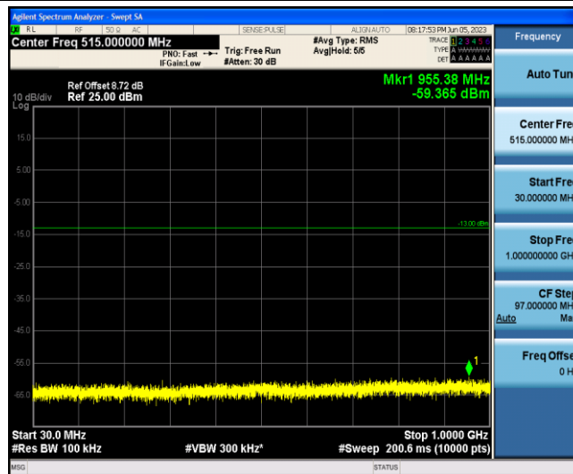
Band2-10MHz-16QAM-18650-1-0-Low-30-1000--59.37-PASS
