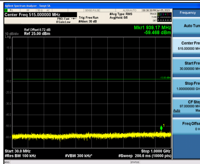
Band2-15MHz-QPSK-18900-1-0-Low-30-1000--59.47-PASS
