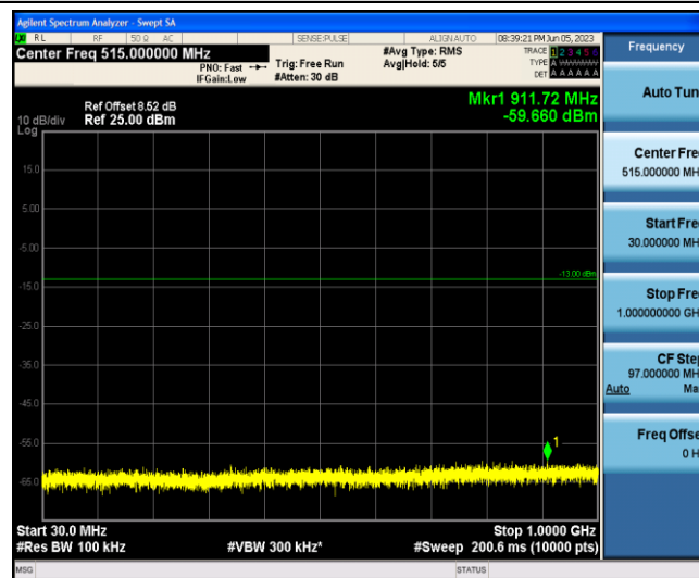
Band2-15MHz-QPSK-19125-1-0-Low-30-1000--59.66-PASS
