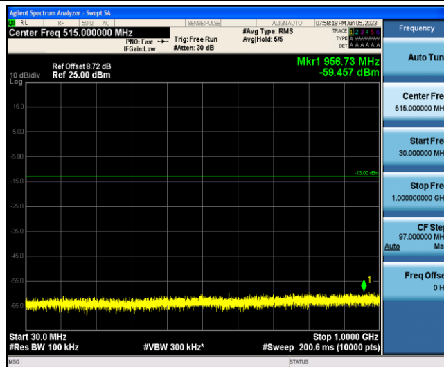
Band2-5MHz-16QAM-18625-1-0-Low-30-1000--59.46-PASS
