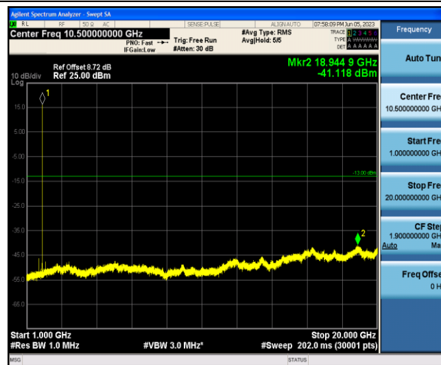
Band2-5MHz-QPSK-18625-1-0-Low-1000-20000--41.12-PASS
