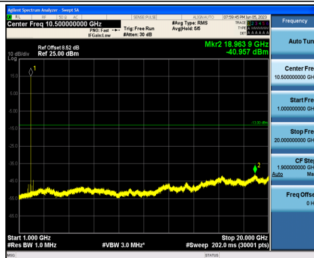
Band2-5MHz-QPSK-19175-1-0-Low-1000-20000--40.96-PASS
