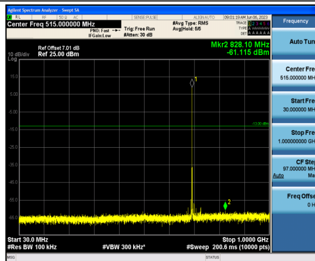
Band12-5MHz-16QAM-23035-1-0-Low-30-1000--61.12-PASS
