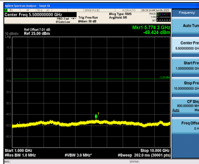
Band12-10MHz-QPSK-23130-1-0-Low-1000-10000--49.42-PASS
