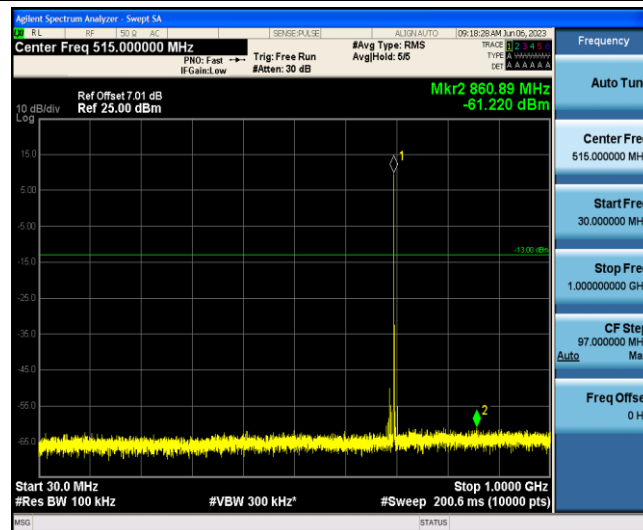
Band12-10MHz-QPSK-23095-1-0-Low-30-1000--61.22-PASS
