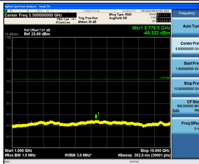
Band12-10MHz-16QAM-23095-1-0-Low-1000-10000--49.33-PASS
