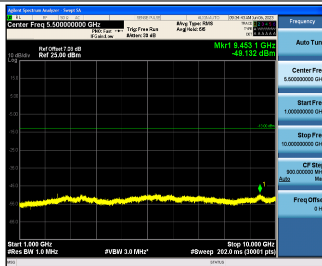
Band13-5MHz-16QAM-23205-1-0-Low-1000-10000--49.13-PASS
