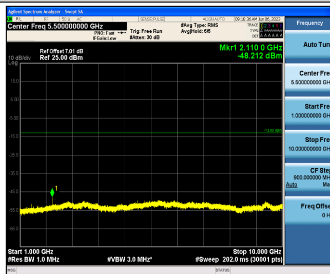
Band12-10MHz-QPSK-23095-1-0-Low-1000-10000--48.21-PASS
