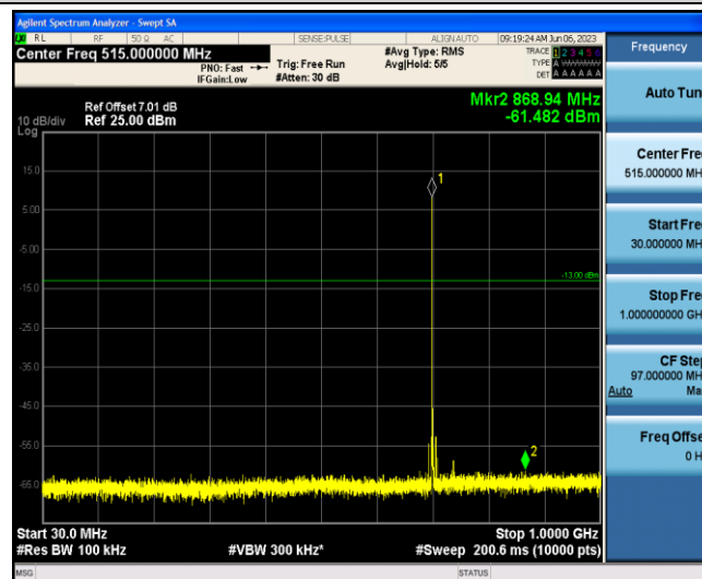
Band12-10MHz-16QAM-23130-1-0-Low-30-1000--61.48-PASS
