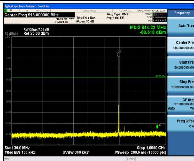
Band12-10MHz-QPSK-23060-1-0-Low-30-1000--60.62-PASS
