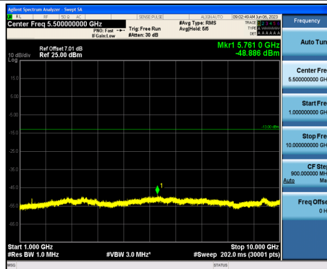
Band12-5MHz-QPSK-23155-1-0-Low-1000-10000--48.89-PASS
