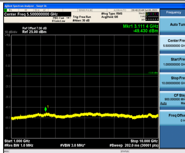
Band13-10MHz-16QAM-23230-1-0-Low-1000-10000--49.43-PASS
