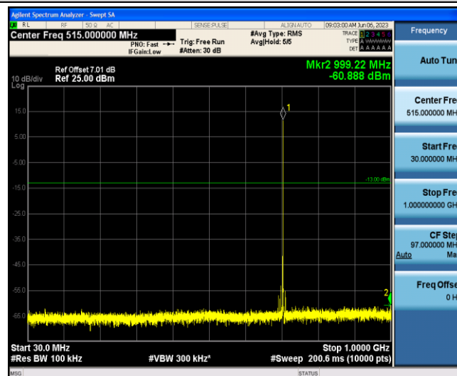
Band12-5MHz-16QAM-23155-1-0-Low-30-1000--60.89-PASS
