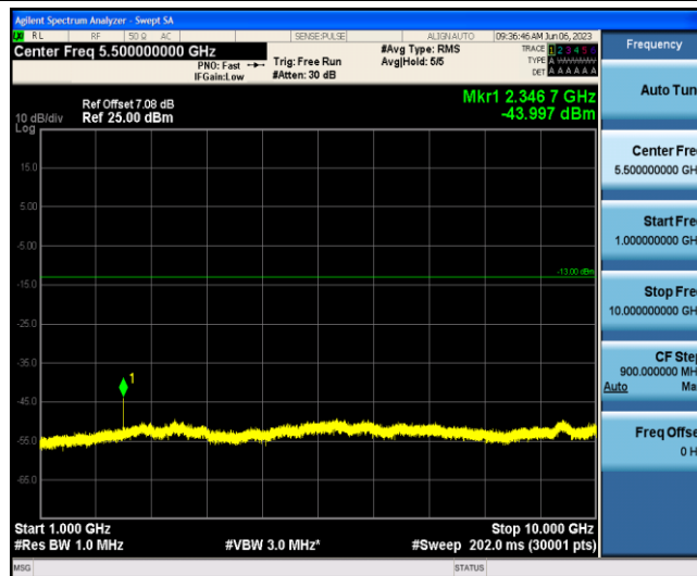
Band13-5MHz-16QAM-23255-1-0-Low-1000-10000--44-PASS
