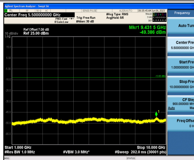
Band13-5MHz-16QAM-23230-1-0-Low-1000-10000--49.39-PASS
