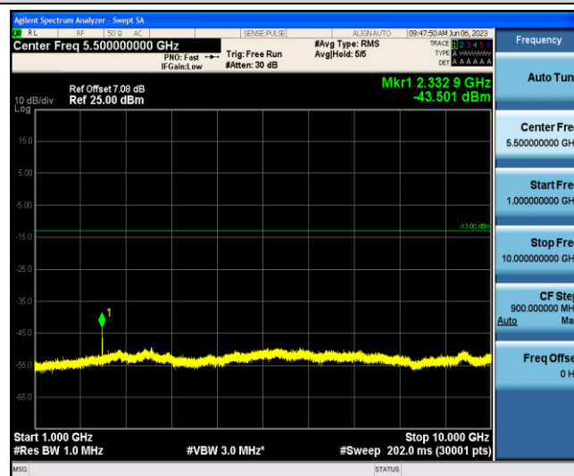
Band13-10MHz-QPSK-23230-1-0-Low-1000-10000--43.5-PASS
