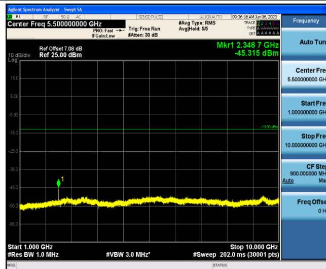
Band13-5MHz-QPSK-23255-1-0-Low-1000-10000--45.32-PASS
