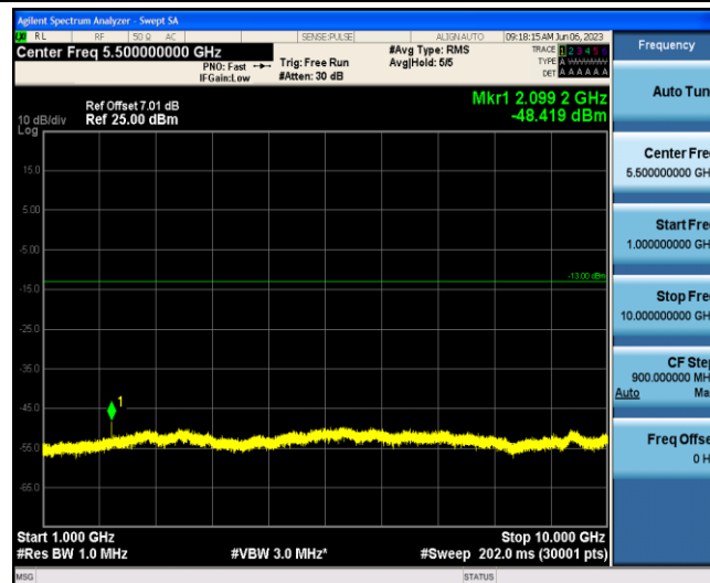
Band12-10MHz-16QAM-23060-1-0-Low-1000-10000--48.42-PASS
