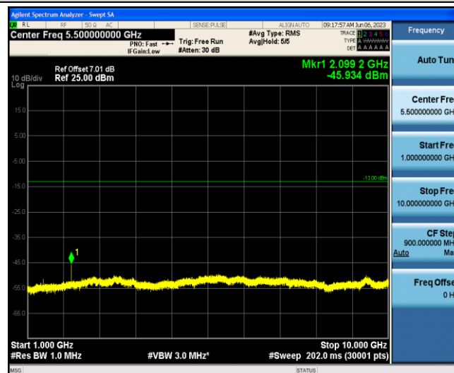
Band12-10MHz-QPSK-23060-1-0-Low-1000-10000--45.93-PASS
