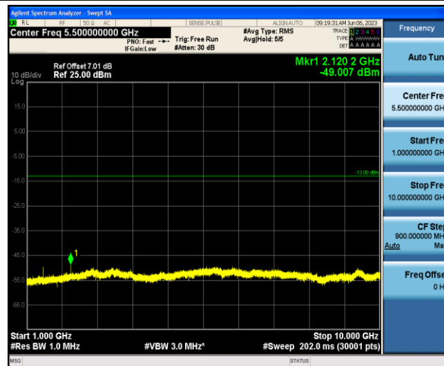
Band12-10MHz-16QAM-23130-1-0-Low-1000-10000--49.01-PASS
