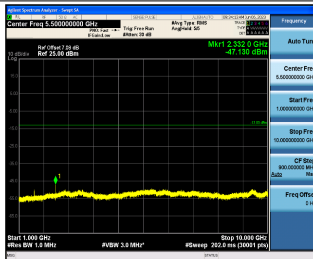
Band13-5MHz-QPSK-23205-1-0-Low-1000-10000--47.13-PASS
