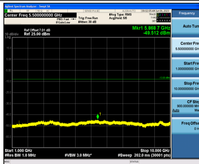
Band12-5MHz-16QAM-23095-1-0-Low-1000-10000--49.51-PASS
