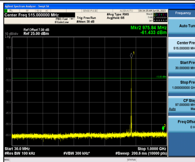
Band13-5MHz-16QAM-23205-1-0-Low-30-1000--61.43-PASS
