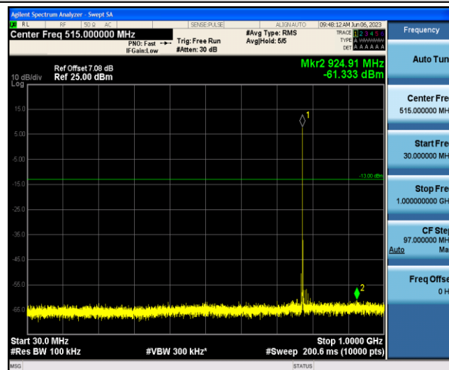
Band13-10MHz-16QAM-23230-1-0-Low-30-1000--61.33-PASS
