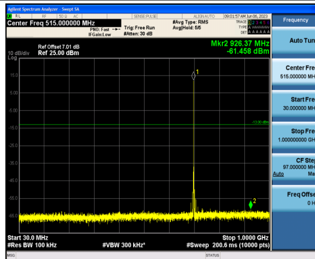
Band12-5MHz-16QAM-23095-1-0-Low-30-1000--61.46-PASS
