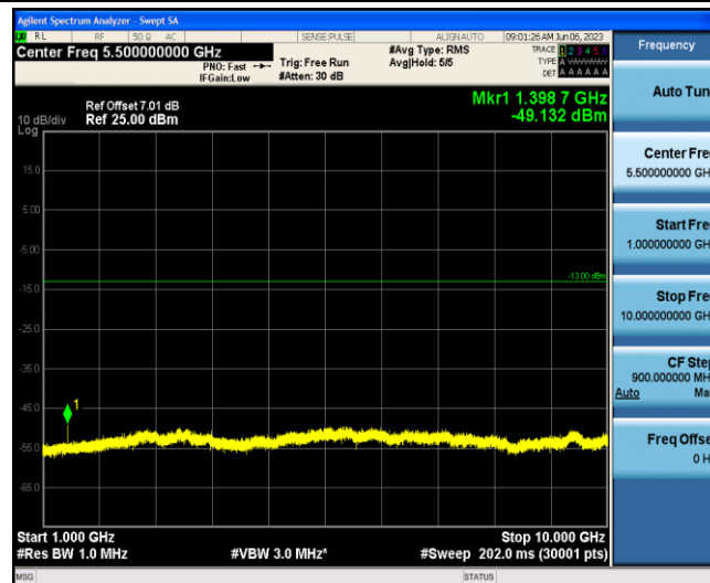
Band12-5MHz-16QAM-23035-1-0-Low-1000-10000--49.13-PASS
