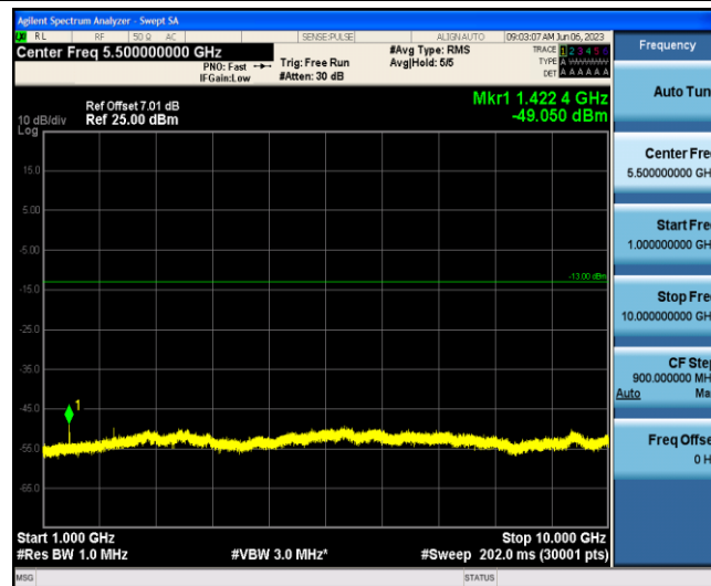
Band12-5MHz-16QAM-23155-1-0-Low-1000-10000--49.05-PASS
