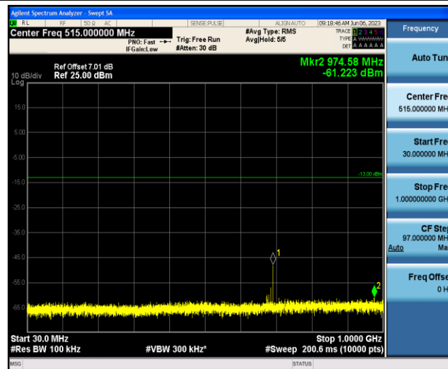
Band12-10MHz-16QAM-23095-1-0-Low-30-1000--61.22-PASS
