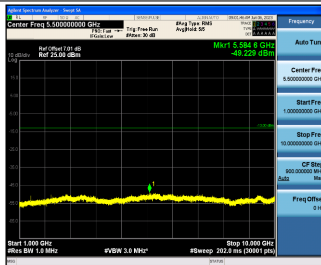
Band12-5MHz-QPSK-23095-1-0-Low-1000-10000--49.23-PASS
