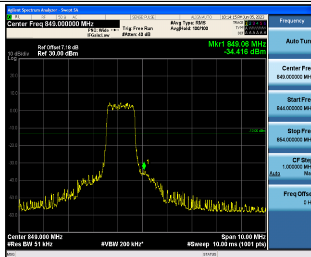
Band5-3MHz-QPSK-20635-6-0-High--34.42-PASS
