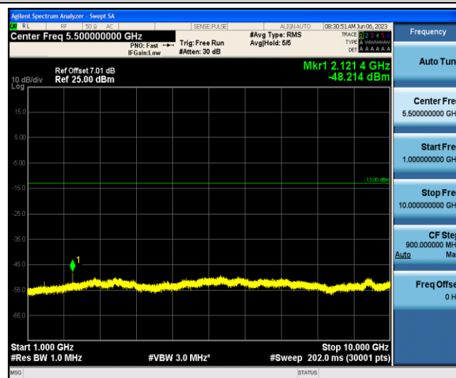
Band12-1.4MHz-16QAM-23095-1-0-Low-1000-10000--48.21-PASS
