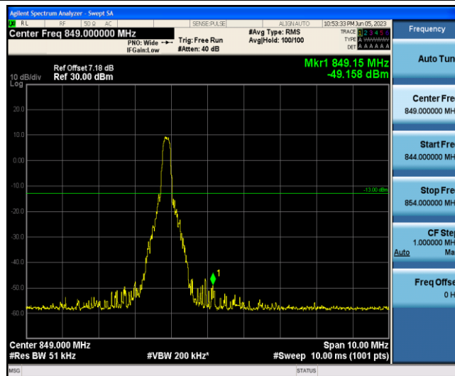
Band5-10MHz-16QAM-20600-1-5-High--49.16-PASS
