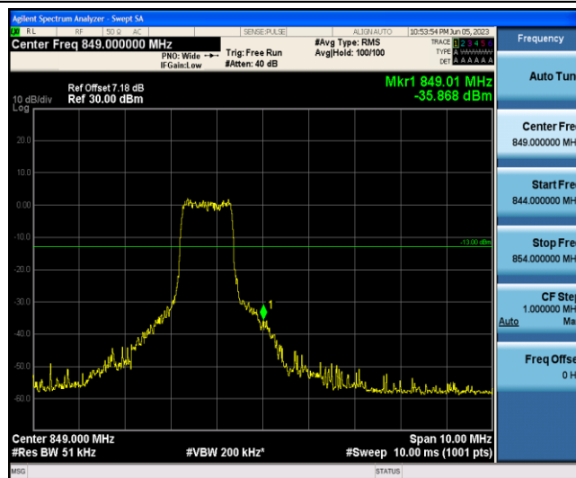
Band5-10MHz-16QAM-20600-6-0-High--35.87-PASS
