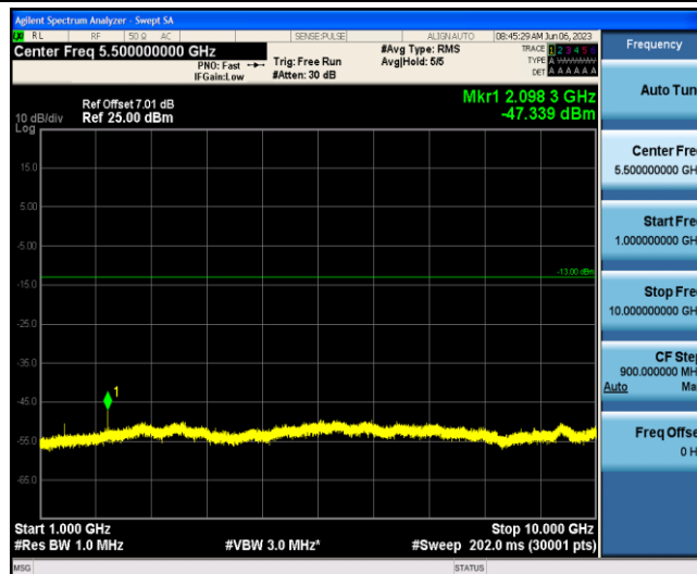
Band12-3MHz-QPSK-23025-1-0-Low-1000-10000--47.34-PASS
