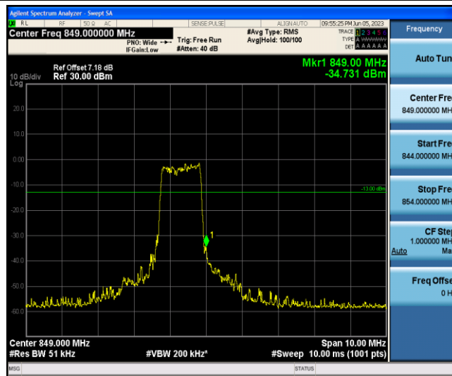
Band5-1.4MHz-QPSK-20643-6-0-High--34.73-PASS
