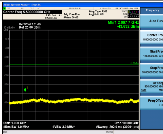
Band12-1.4MHz-OPSK-23017-1-0-Low-1000-10000--43.63-PASS
