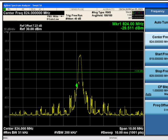
Band5-1.4MHz-16QAM-20407-1-0-Low--29.51-PASS
