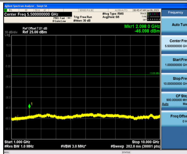
Band12-3MHz-16QAM-23025-1-0-Low-1000-10000--46.1-PASS
