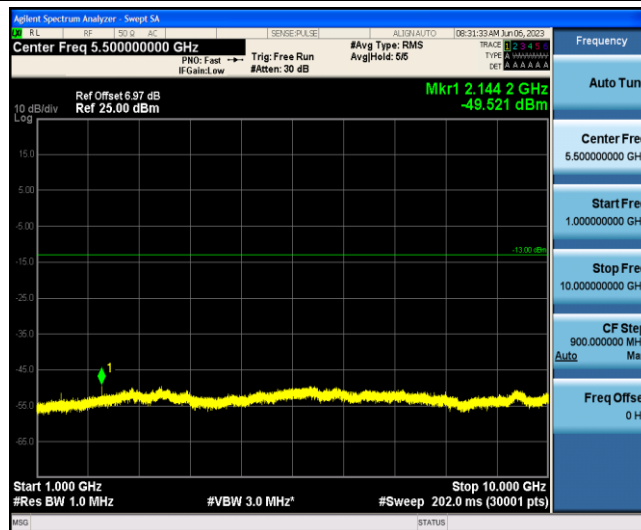
Band12-1.4MHz-16QAM-23173-1-0-Low-1000-10000--49.52-PASS
