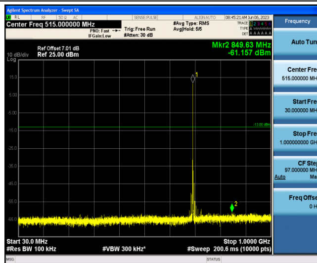
Band12-3MHz-QPSK-23025-1-0-Low-30-1000--61.16-PASS
