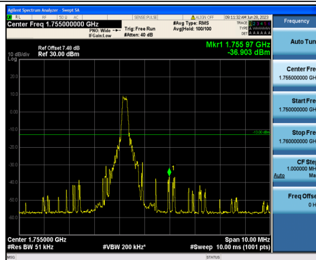
Band4-3MHz-16QAM-20385-1-5-High--36.90-PASS
