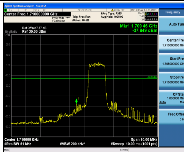
Band4-3MHz-16QAM-19965-6-0-Low--37.85-PASS
