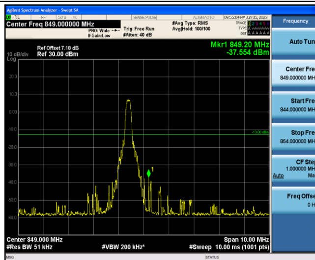
Band5-1.4MHz-QPSK-20643-1-5-High--37.55-PASS
