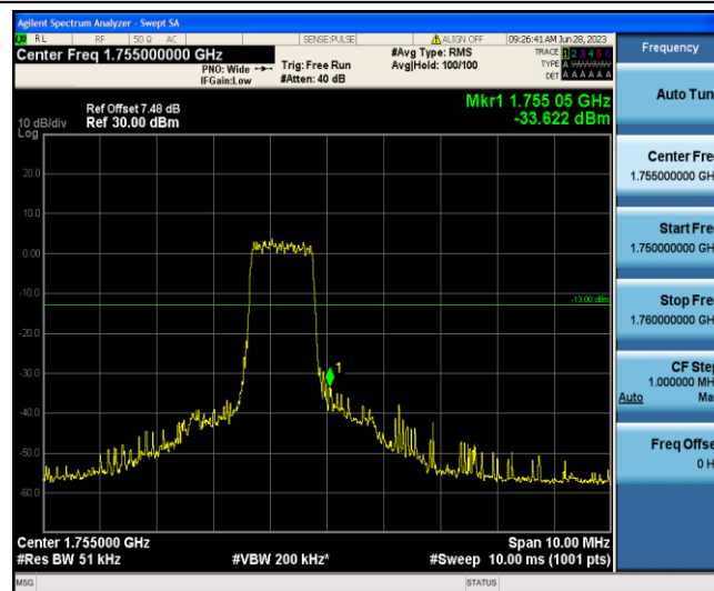
Band4-5MHz-QPSK-20375-6-0-High--33.62-PASS
