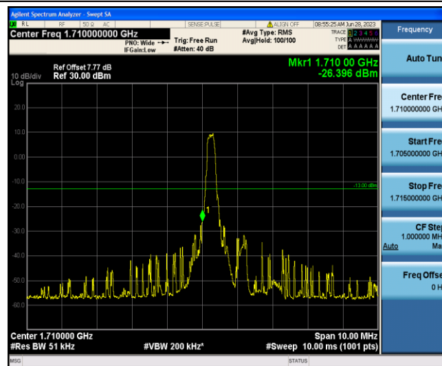
Band4-1.4MHz-16QAM-19957-1-0-Low--26.40-PASS
