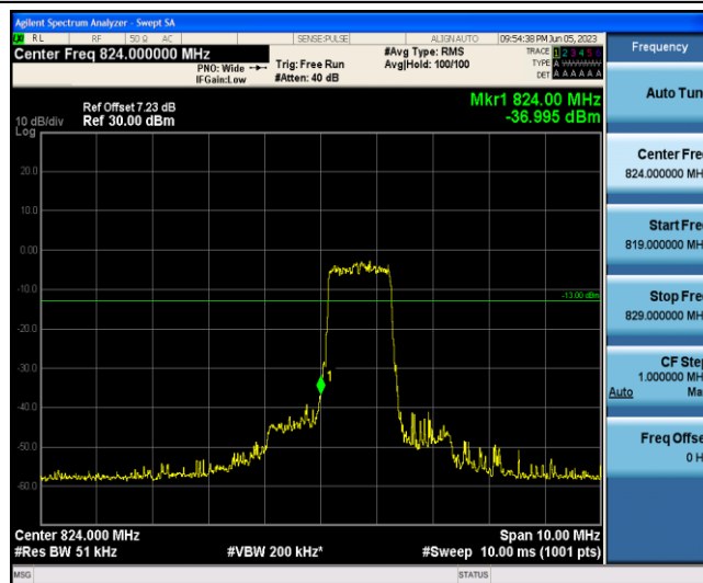
Band5-1.4MHz-QPSK-20407-6-0-Low--37.00-PASS
