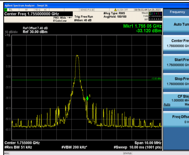
Band4-1.4MHz-QPSK-20393-1-5-High--33.12-PASS
