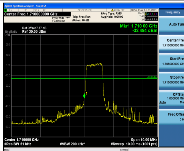
Band4-1.4MHz-16QAM-19957-6-0-Low--32.48-PASS
