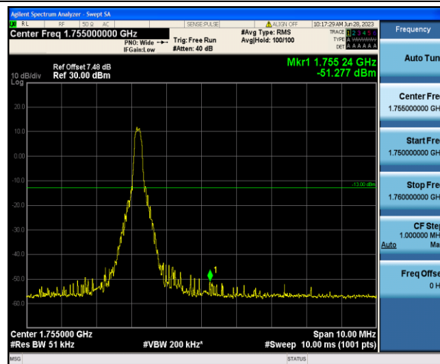
Band4-20MHz-16QAM-20300-1-5-High--51.28-PASS
