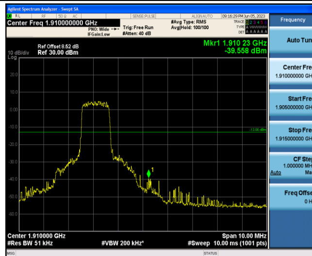
Band2-20MHz-16QAM-19100-6-0-High--39.56-PASS
