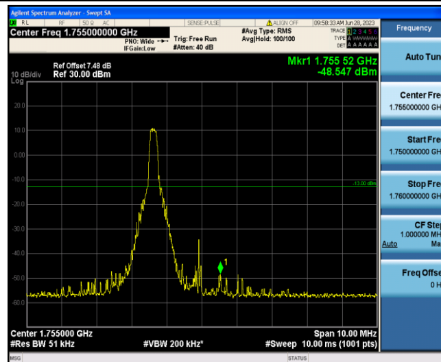
Band4-15MHz-16QAM-20325-1-5-High--48.55-PASS
