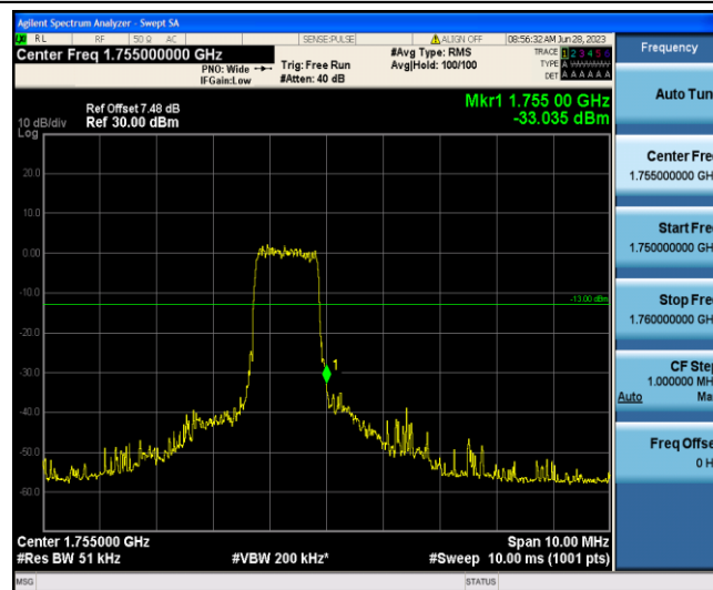
Band4-1.4MHz-16QAM-20393-6-0-High--33.04-PASS
