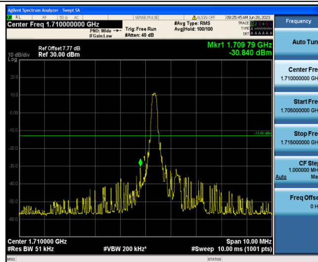
Band4-5MHz-16QAM-19975-1-0-Low--30.84-PASS
