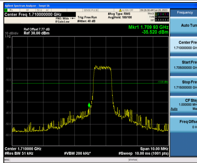
Band4-5MHz-16QAM-19975-6-0-Low--35.52-PASS
