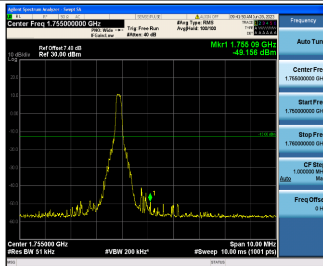
Band4-10MHz-16QAM-20350-1-5-High--49.16-PASS
