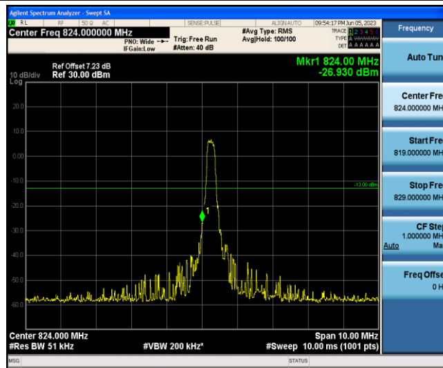
Band5-1.4MHz-QPSK-20407-1-0-Low--26.93-PASS
