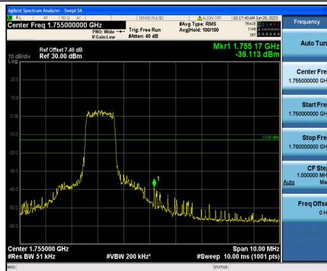
Band4-20MHz-QPSK-20300-6-0-High--39.11-PASS
