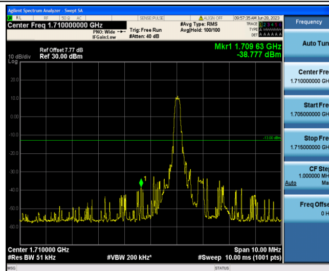
Band4-15MHz-QPSK-20025-1-0-Low--38.78-PASS
