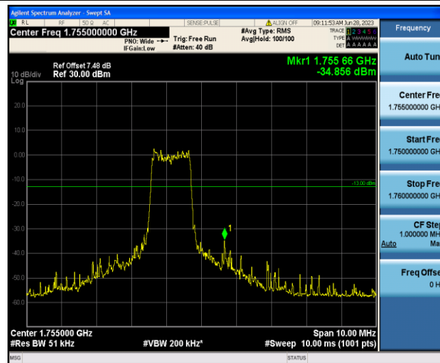
Band4-3MHz-16QAM-20385-6-0-High--34.86-PASS
