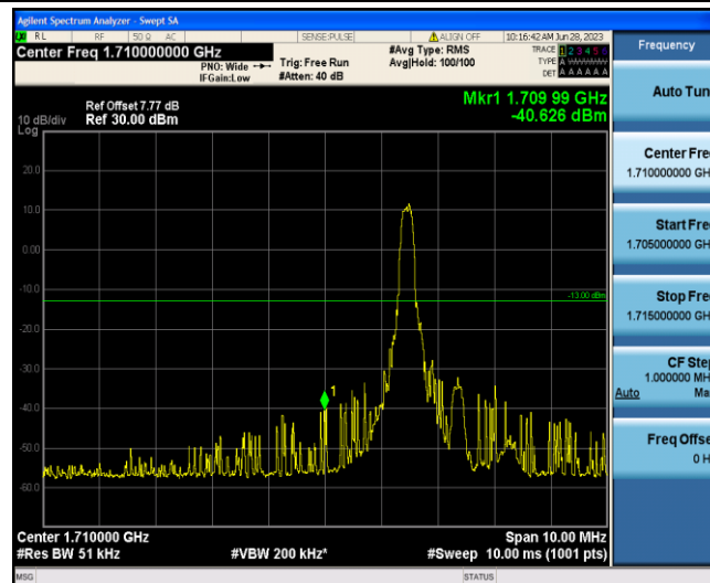
Band4-20MHz-16QAM-20050-1-0-Low--40.63-PASS
