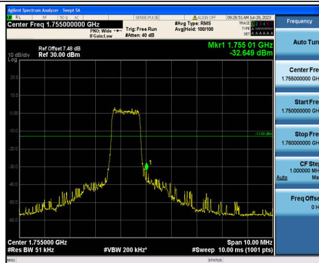
Band4-5MHz-16QAM-20375-6-0-High--32.65-PASS
