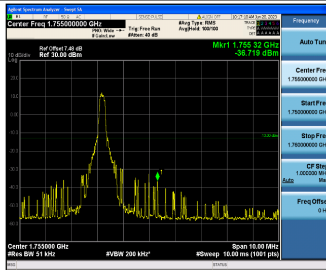
Band4-20MHz-QPSK-20300-1-5-High--36.72-PASS
