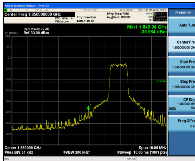
Band2-20MHz-16QAM-18700-6-0-Low--38.96-PASS
