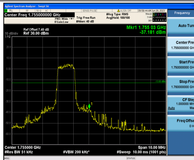
Band4-15MHz-QPSK-20325-6-0-High--37.18-PASS
