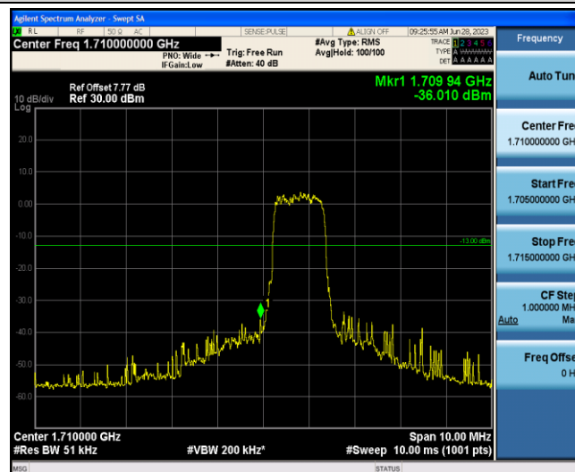
Band4-5MHz-QPSK-19975-6-0-Low--36.01-PASS
