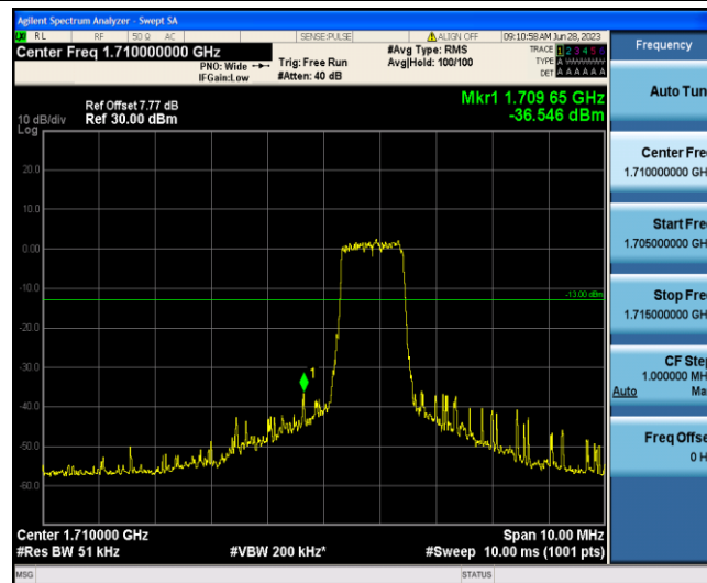
Band4-3MHz-QPSK-19965-6-0-Low--36.55-PASS
