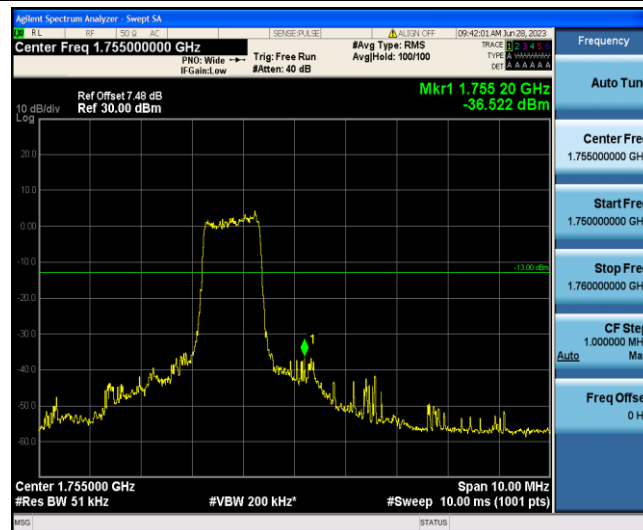
Band4-10MHz-QPSK-20350-6-0-High--36.52-PASS
