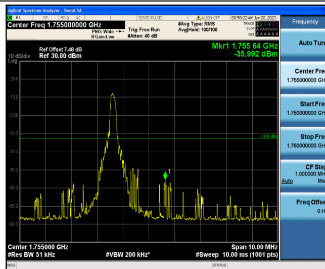
Band4-15MHz-QPSK-20325-1-5-High--35.99-PASS
