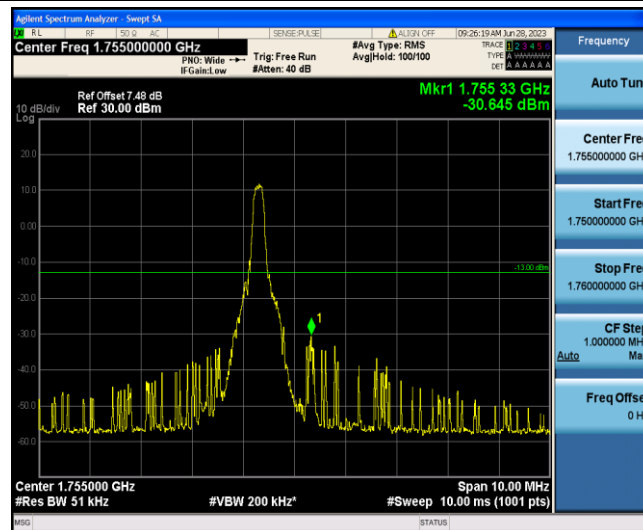
Band4-5MHz-QPSK-20375-1-5-High--30.64-PASS
