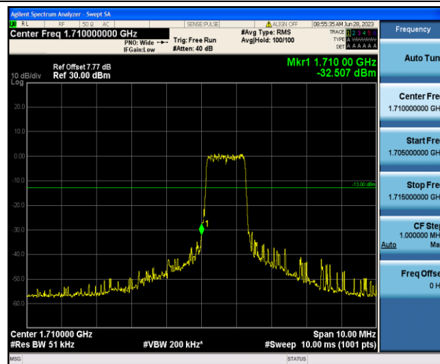
Band4-1.4MHz-QPSK-19957-6-0-Low--32.51-PASS
