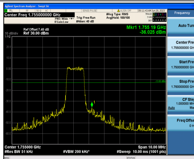
Band4-3MHz-QPSK-20385-6-0-High--36.02-PASS
