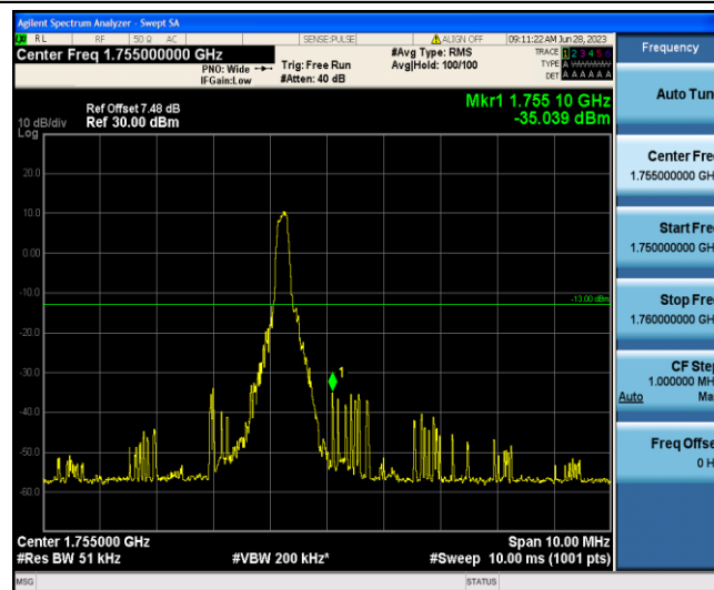
Band4-3MHz-QPSK-20385-1-5-High--35.04-PASS
