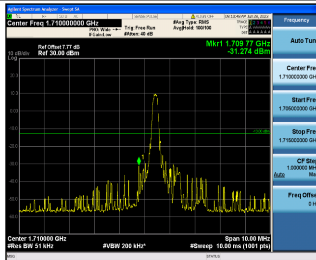
Band4-3MHz-16QAM-19965-1-0-Low--31.27-PASS
