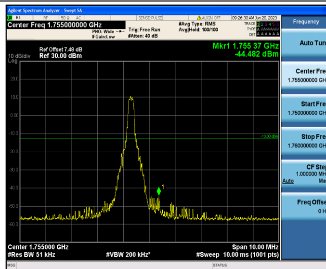
Band4-5MHz-16QAM-20375-1-5-High--44.48-PASS
