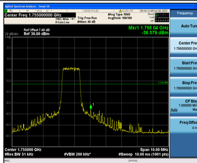
Band4-10MHz-16QAM-20350-6-0-High--36.58-PASS
