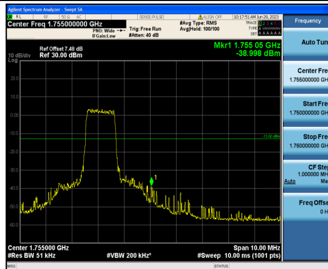
Band4-20MHz-16QAM-20300-6-0-High--39.00-PASS
