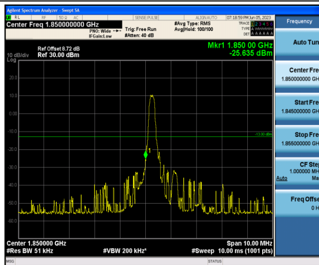
Band2-1.4MHz-16QAM-18607-1-0-Low--25.63-PASS
