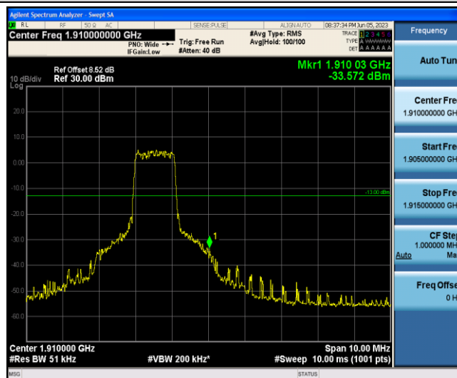
Band2-15MHz-QPSK-19125-6-0-High--33.57-PASS
