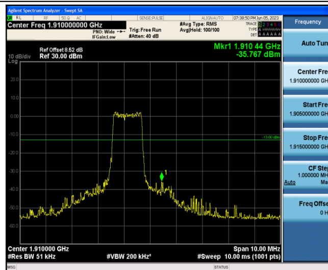
Band2-3MHz-QPSK-19185-6-0-High--35.77-PASS
