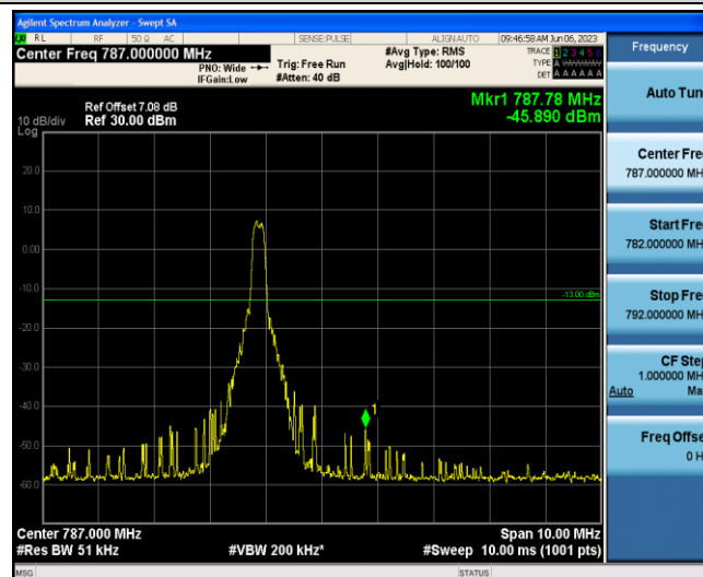
Band13-10MHz-QPSK-23230-1-5-High--45.89-PASS
