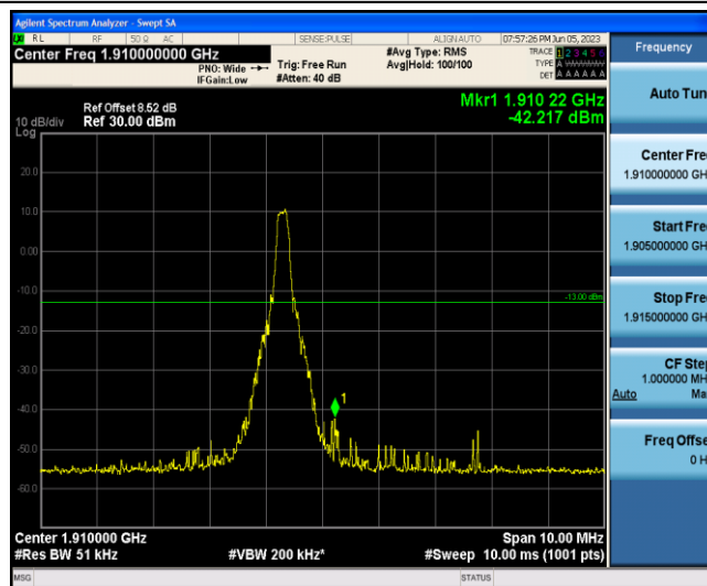
Band2-5MHz-16QAM-19175-1-5-High--42.22-PASS
