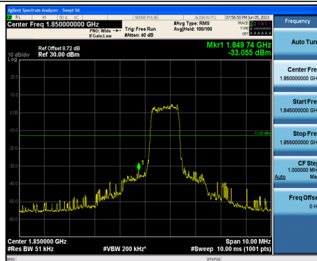
Band2-5MHz-QPSK-18625-6-0-Low--33.05-PASS
