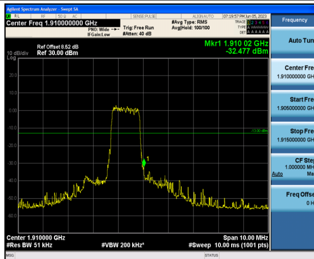
Band2-1.4MHz-QPSK-19193-6-0-High--32.48-PASS
