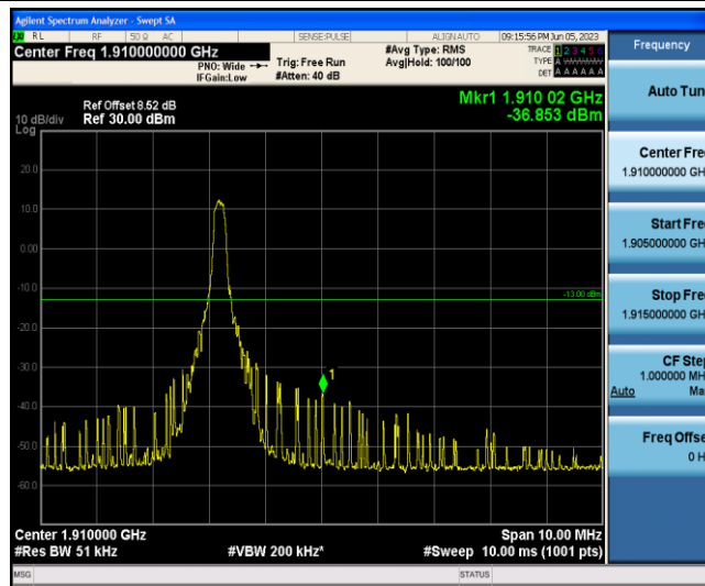
Band2-20MHz-QPSK-19100-1-5-High--36.85-PASS
