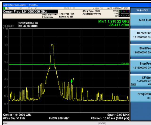
Band2-15MHz-QPSK-19125-1-5-High--35.42-PASS
