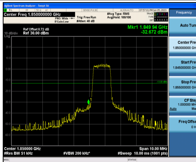
Band2-5MHz-16QAM-18625-6-0-Low--32.67-PASS
