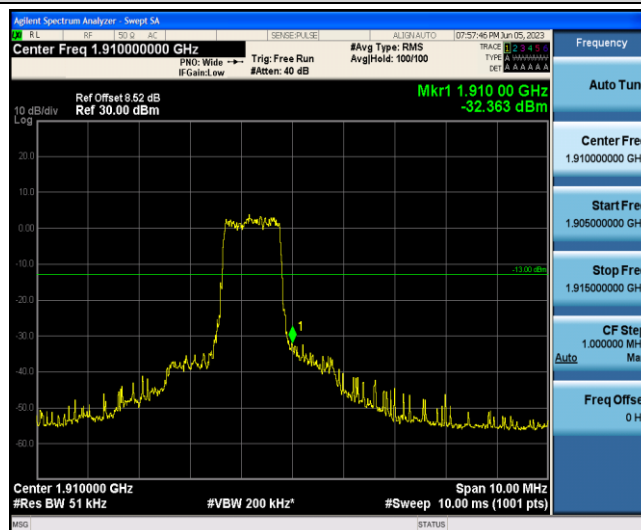
Band2-5MHz-16QAM-19175-6-0-High--32.36-PASS
