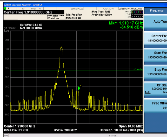
Band2-10MHz-QPSK-19150-1-5-High--34.52-PASS
