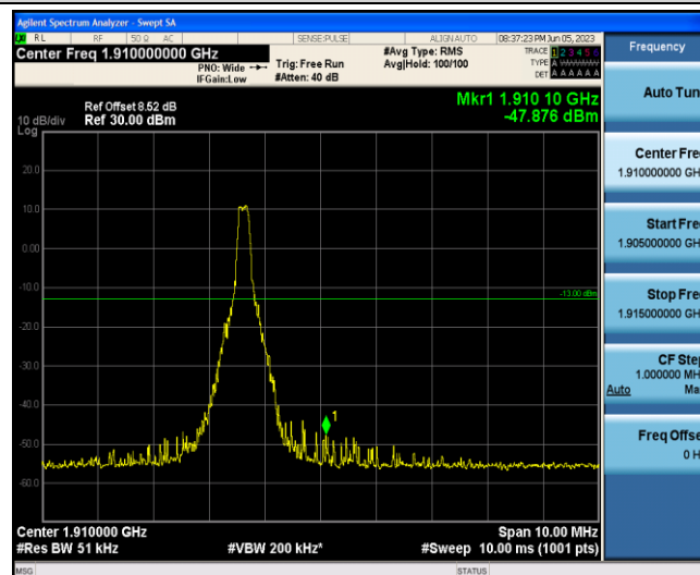
Band2-15MHz-16QAM-19125-1-5-High--47.88-PASS
