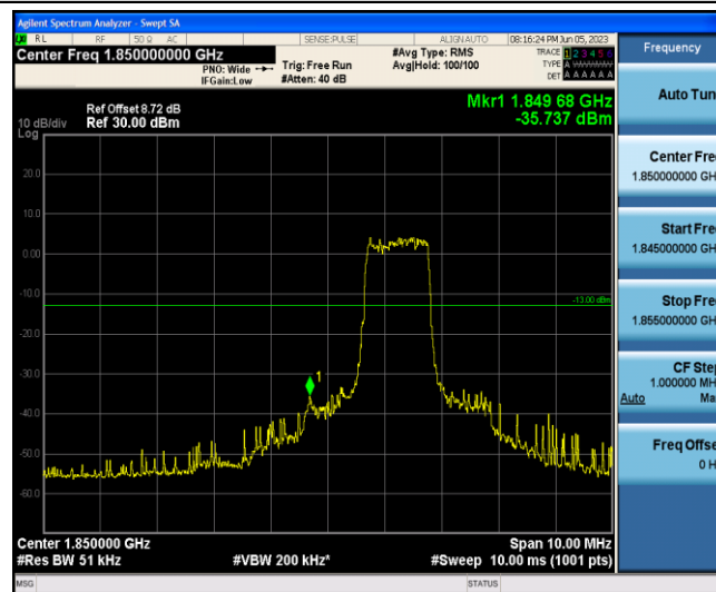
Band2-10MHz-QPSK-18650-6-0-Low--35.74-PASS
