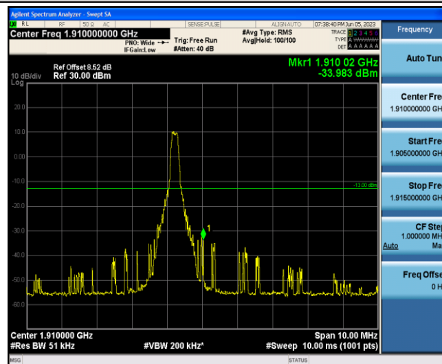
Band2-3MHz-16QAM-19185-1-5-High--33.98-PASS
