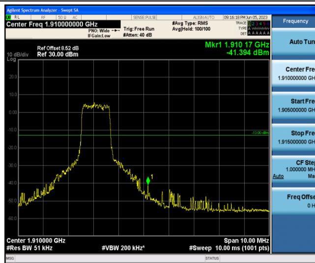
Band2-20MHz-QPSK-19100-6-0-High--41.39-PASS
