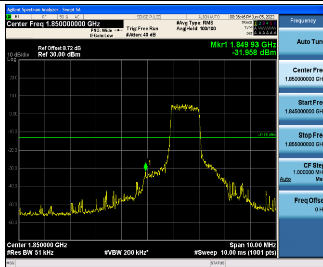
Band2-15MHz-QPSK-18675-6-0-Low--31.96-PASS
