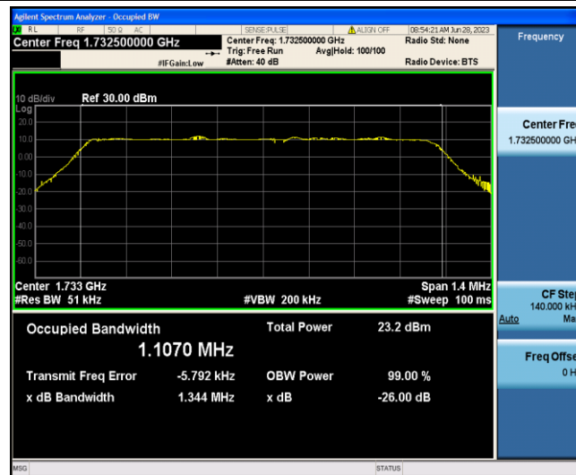
Band4-1.4MHz-16QAM-20175-6-0-Low-1.1070-1.344-PASS
