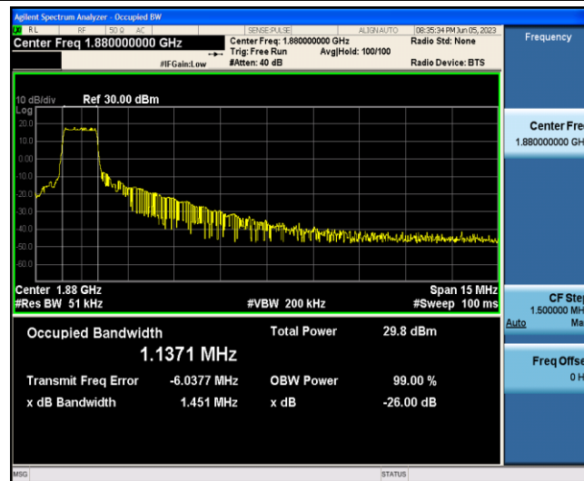
Band2-15MHz-16QAM-18900-6-0-Low-1.1371-1.451-PASS
