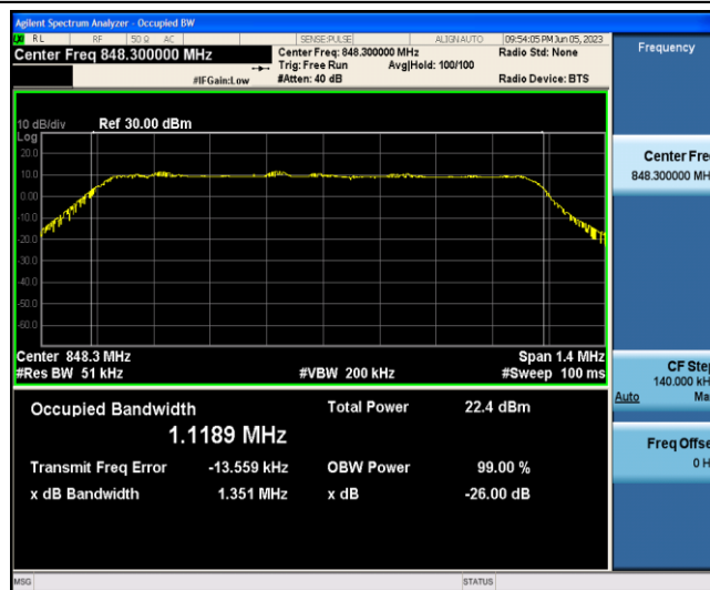
Band5-1.4MHz-16QAM-20643-6-0-Low-1.1189-1.351-PASS
