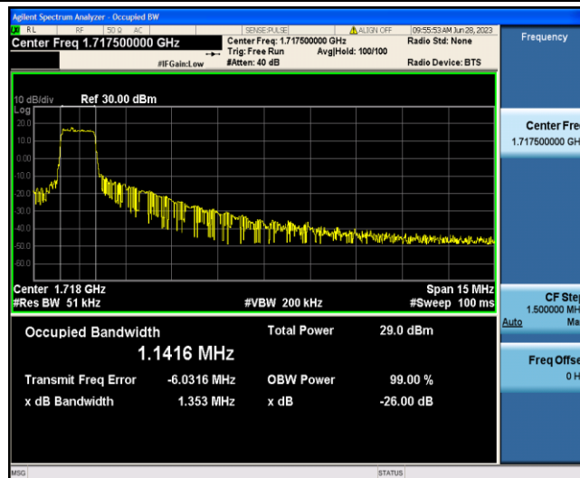
Band4-15MHz-QPSK-20025-6-0-Low-1.1416-1.353-PASS
