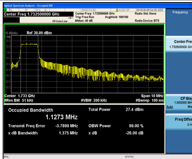
Band4-10MHz-16QAM-20175-6-0-Low-1.1273-1.375-PASS
