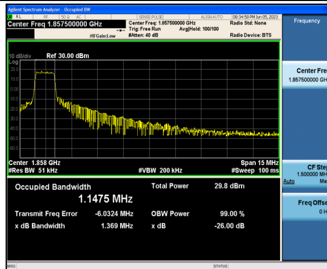
Band2-15MHz-16QAM-18675-6-0-Low-1.1475-1.369-PASS
