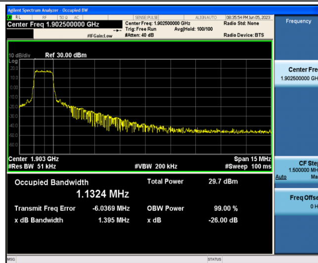
Band2-15MHz-QPSK-19125-6-0-Low-1.1324-1.395-PASS
