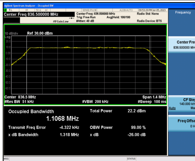
Band5-1.4MHz-16QAM-20525-6-0-Low-1.1068-1.318-PASS
