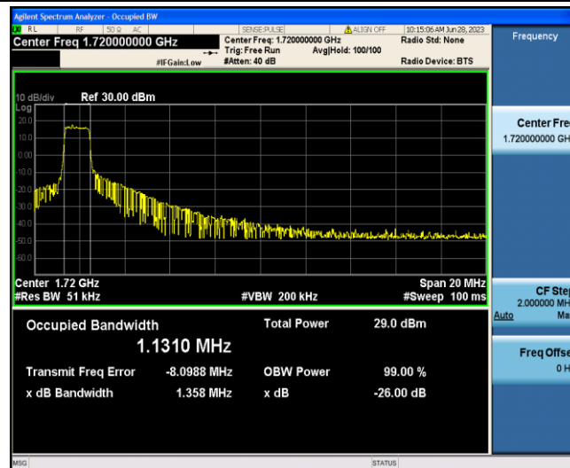
Band4-20MHz-16QAM-20050-6-0-Low-1.1310-1.358-PASS
