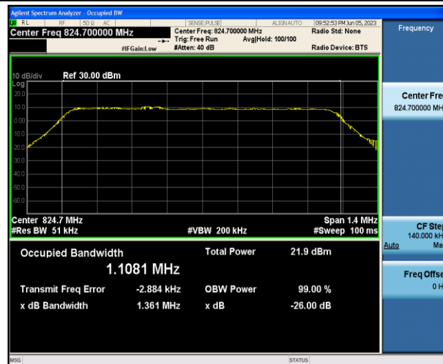
Band5-1.4MHz-16QAM-20407-6-0-Low-1.1081-1.361-PASS
