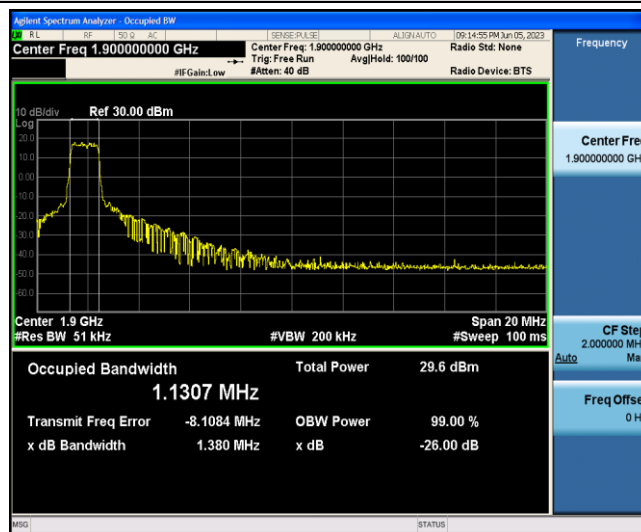
Band2-20MHz-16QAM-19100-6-0-Low-1.1307-1.380-PASS
