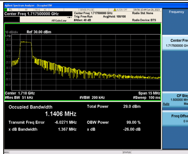
Band4-15MHz-16QAM-20025-6-0-Low-1.1406-1.367-PASS
