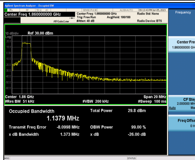
Band2-20MHz-16QAM-18700-6-0-Low-1.1379-1.373-PASS
