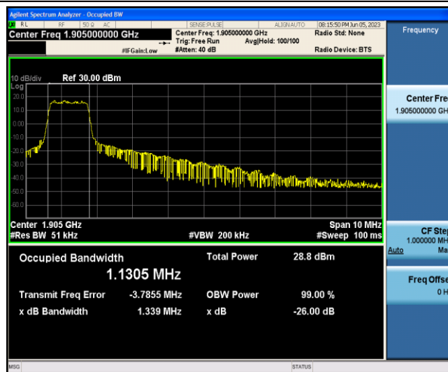
Band2-10MHz-16QAM-19150-6-0-Low-1.1305-1.339-PASS
