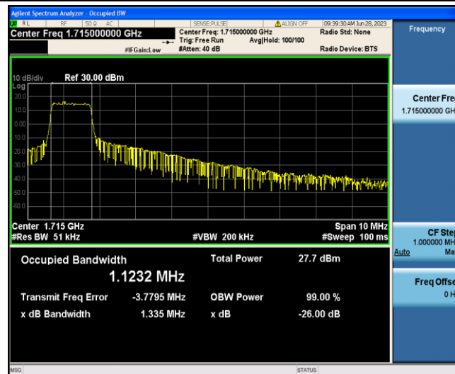
Band4-10MHz-16QAM-20000-6-0-Low-1.1232-1.335-PASS
