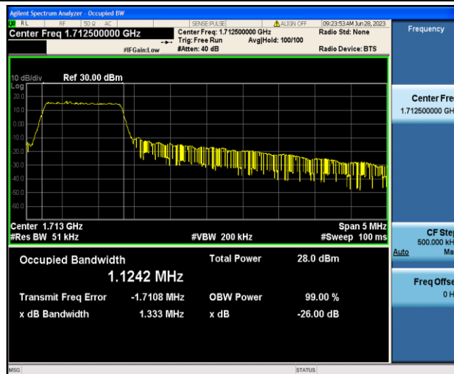
Band4-5MHz-QPSK-19975-6-0-Low-1.1242-1.333-PASS
