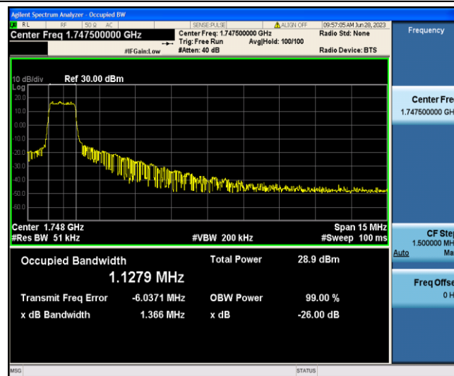
Band4-15MHz-QPSK-20325-6-0-Low-1.1279-1.366-PASS
