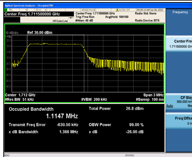
Band4-3MHz-16QAM-19965-6-0-Low-1.1147-1.366-PASS
