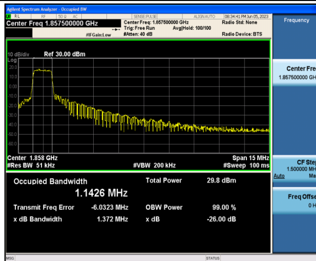
Band2-15MHz-QPSK-18675-6-0-Low-1.1426-1.372-PASS
