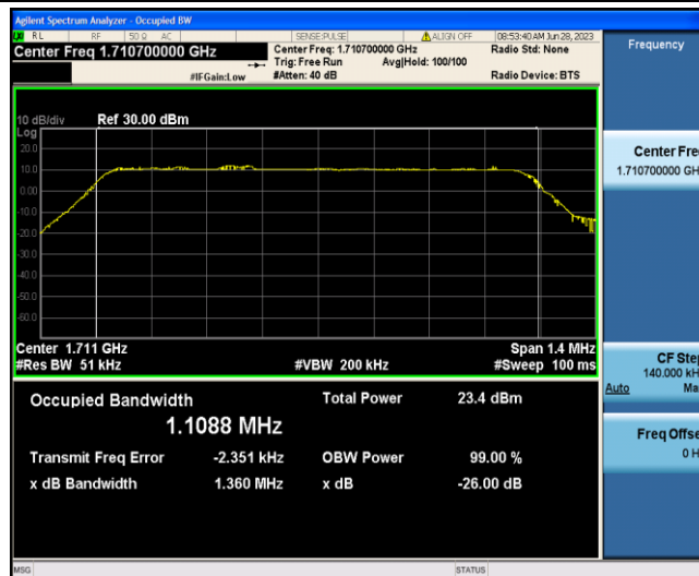
Band4-1.4MHz-16QAM-19957-6-0-Low-1.1088-1.360-PASS
