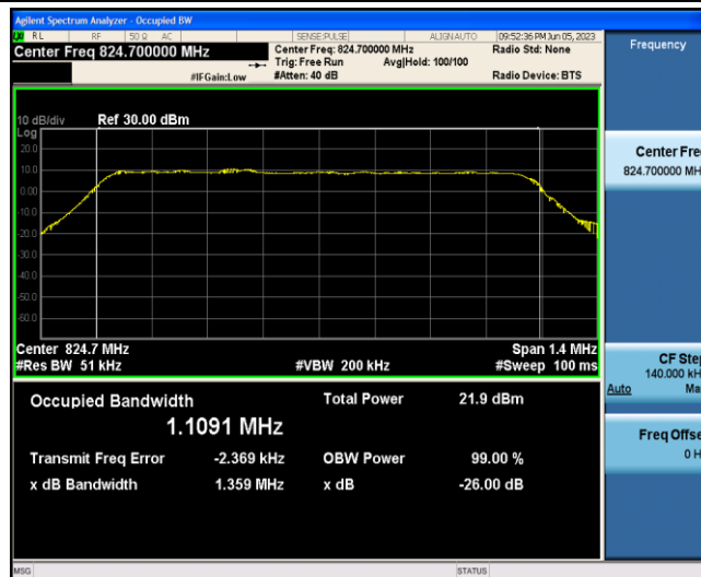
Band5-1.4MHz-QPSK-20407-6-0-Low-1.1091-1.359-PASS
