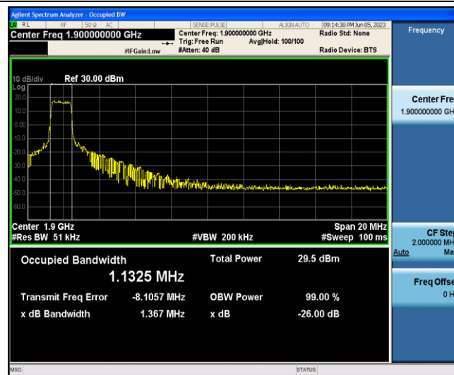
Band2-20MHz-QPSK-19100-6-0-Low-1.1325-1.367-PASS
