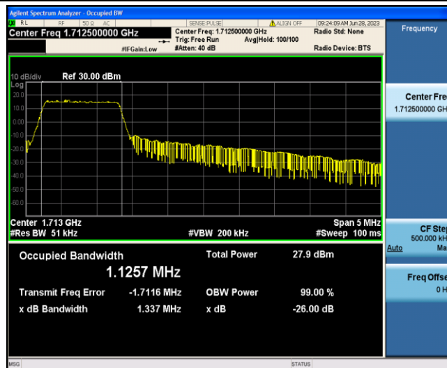
Band4-5MHz-16QAM-19975-6-0-Low-1.1257-1.337-PASS
