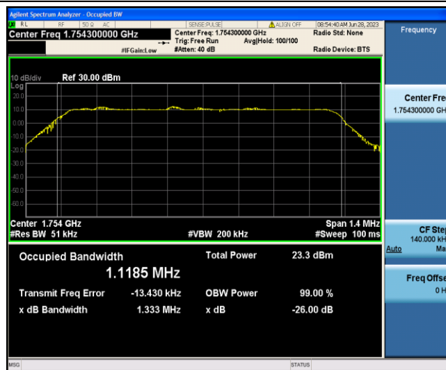
Band4-1.4MHz-QPSK-20393-6-0-Low-1.1185-1.333-PASS
