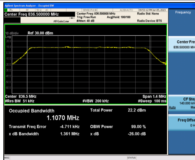
Band5-1.4MHz-QPSK-20525-6-0-Low-1.1070-1.361-PASS
