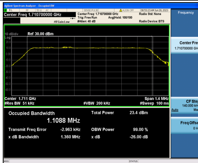
Band4-1.4MHz-QPSK-19957-6-0-Low-1.1088-1.360-PASS
