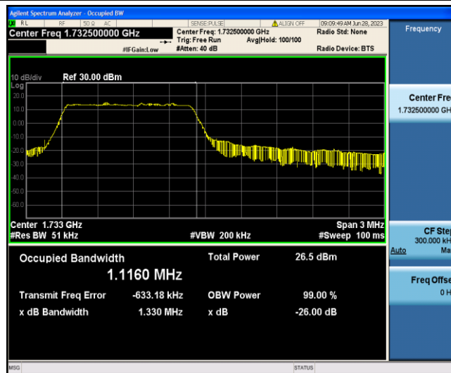
Band4-3MHz-16QAM-20175-6-0-Low-1.1160-1.330-PASS
