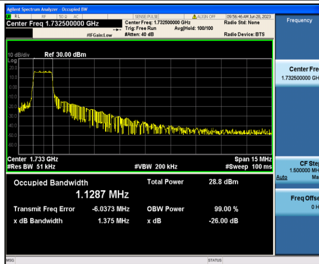
Band4-15MHz-16QAM-20175-6-0-Low-1.1287-1.375-PASS
