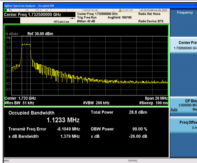
Band4-20MHz-16QAM-20175-6-0-Low-1.1233-1.379-PASS
