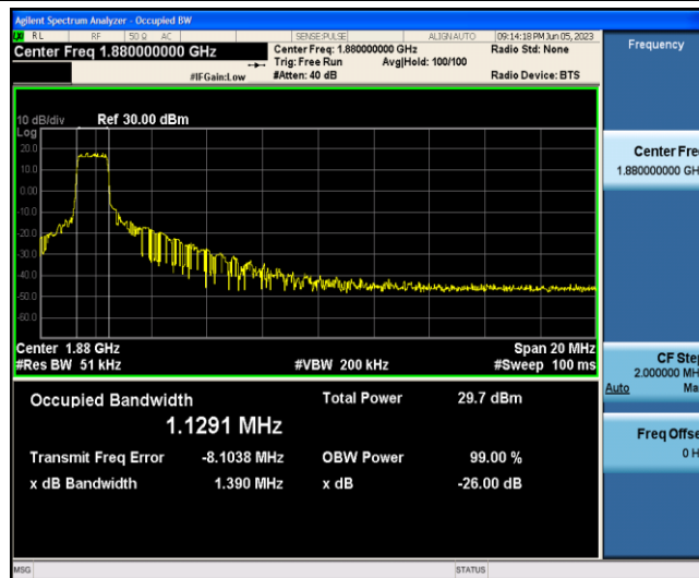
Band2-20MHz-16QAM-18900-6-0-Low-1.1291-1.390-PASS
