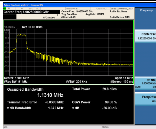
Band2-15MHz-16QAM-19125-6-0-Low-1.1310-1.372-PASS
