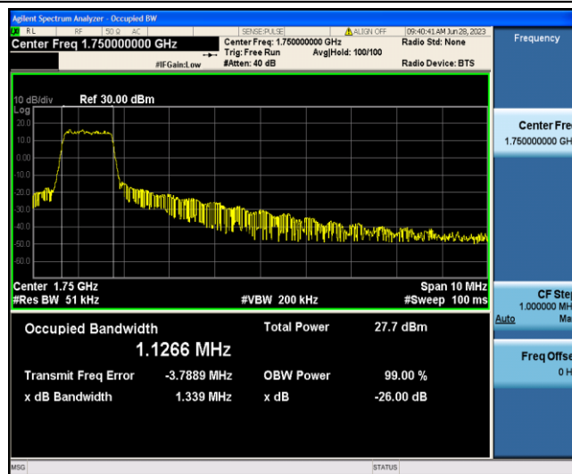
Band4-10MHz-16QAM-20350-6-0-Low-1.1266-1.339-PASS
