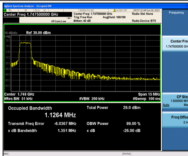
Band4-15MHz-16QAM-20325-6-0-Low-1.1264-1.351-PASS
