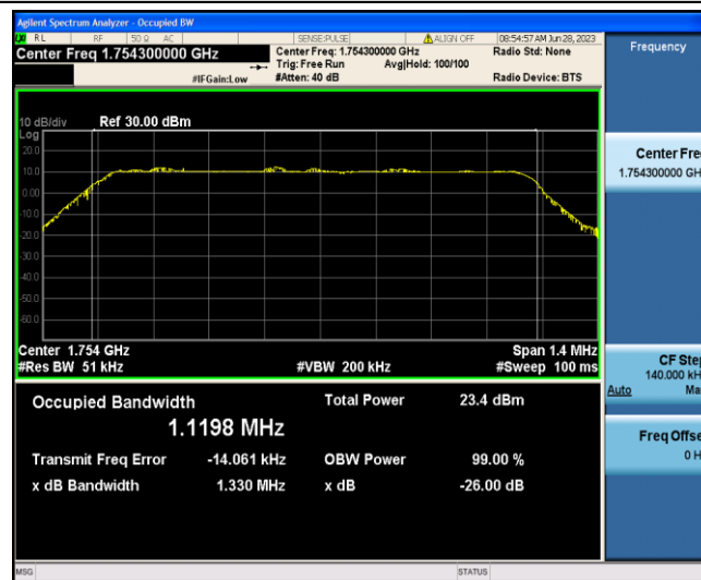
Band4-1.4MHz-16QAM-20393-6-0-Low-1.1198-1.330-PASS
