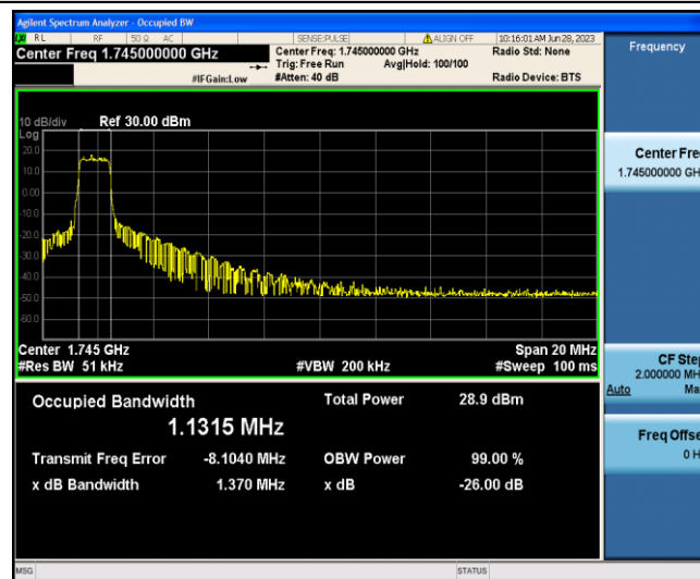
Band4-20MHz-QPSK-20300-6-0-Low-1.1315-1.370-PASS
