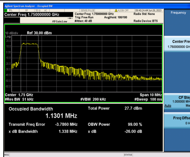
Band4-10MHz-QPSK-20350-6-0-Low-1.1301-1.338-PASS
