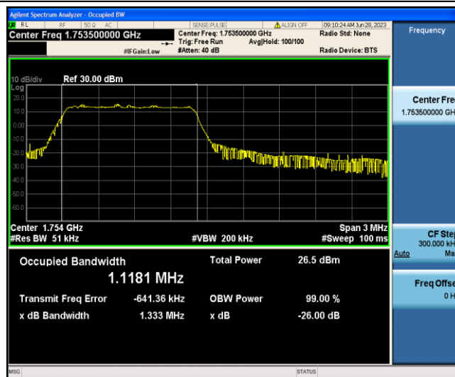
Band4-3MHz-16QAM-20385-6-0-Low-1.1181-1.333-PASS
