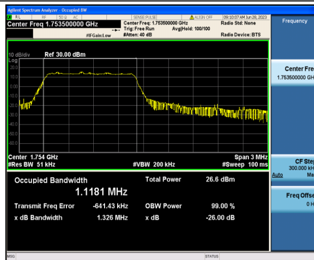
Band4-3MHz-QPSK-20385-6-0-Low-1.1181-1.326-PASS
