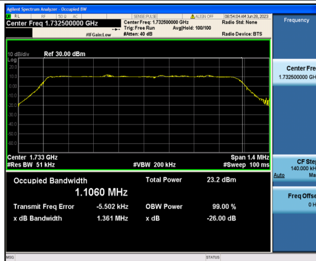
Band4-1.4MHz-QPSK-20175-6-0-Low-1.1060-1.361-PASS
