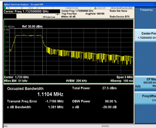
Band4-5MHz-16QAM-20175-6-0-Low-1.1104-1.381-PASS
