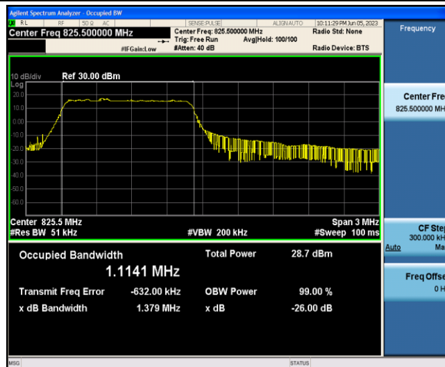
Band5-3MHz-QPSK-20415-6-0-Low-1.1141-1.379-PASS
