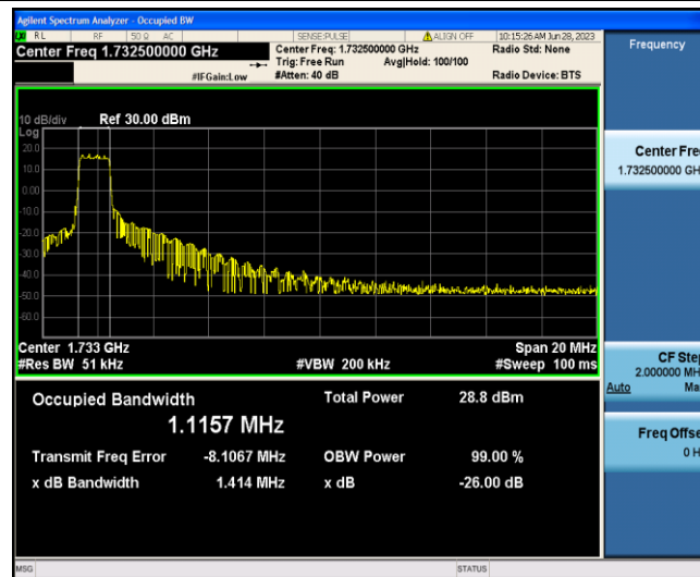
Band4-20MHz-QPSK-20175-6-0-Low-1.1157-1.414-PASS
