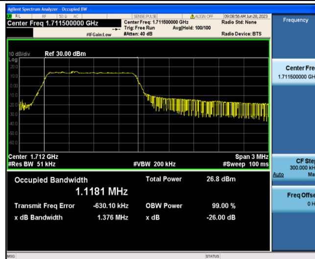
Band4-3MHz-QPSK-19965-6-0-Low-1.1181-1.376-PASS
