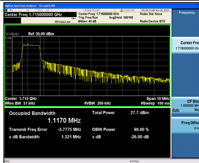
Band4-10MHz-QPSK-20000-6-0-Low-1.1170-1.321-PASS
