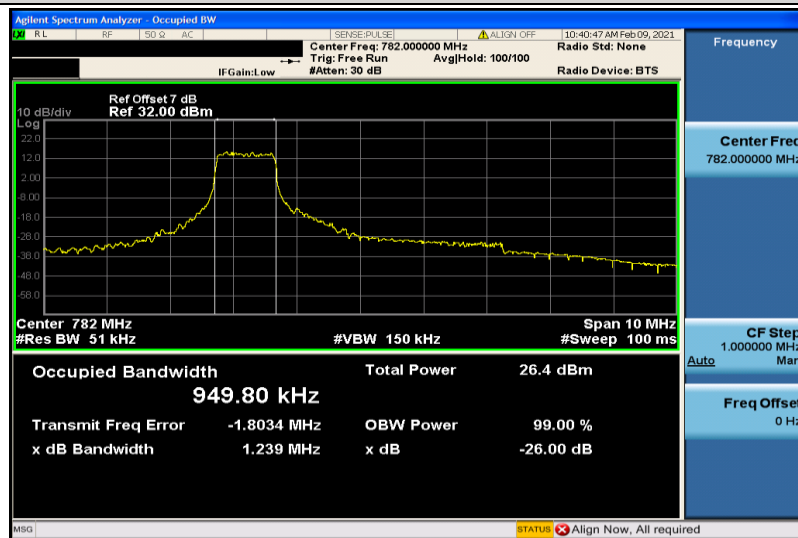
Band13-5MHz-16QAM-23230-6RB#0-0.9498
