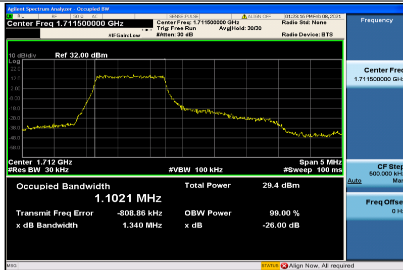
Band4-3MHz-QPSK-19965-6RB#0-1.1021
