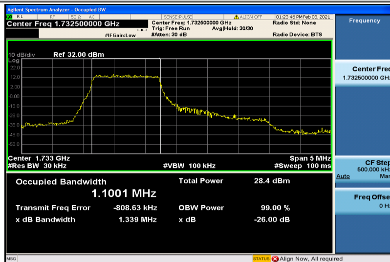
Band4-3MHz-16QAM-20175-6RB#0-1.1001
