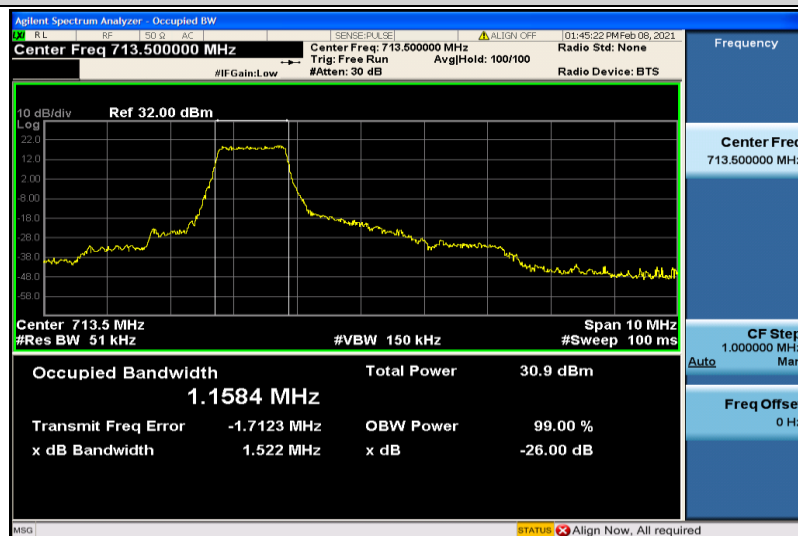
Band12-5MHz-QPSK-23155-6RB#0-1.1584
