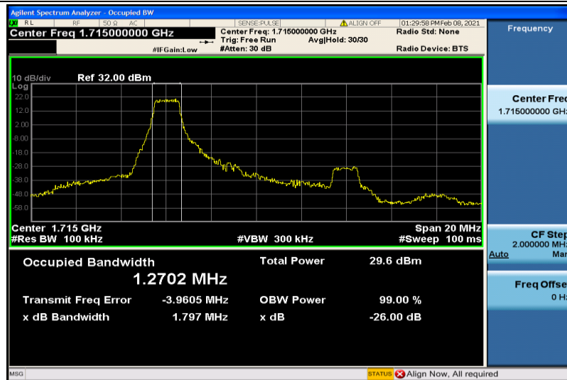
Band4-10MHz-16QAM-20000-6RB#0-1.2702
