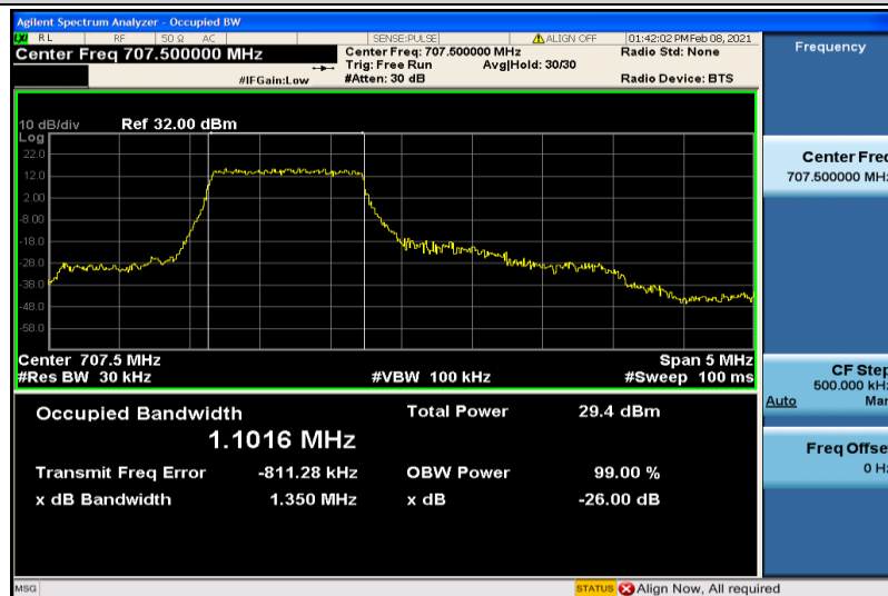
Band12-3MHz-QPSK-23095-6RB#0-1.1016
