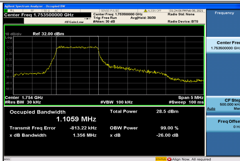
Band4-3MHz-16QAM-20385-6RB#0-1.1059
