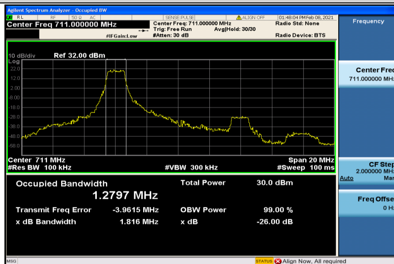
Band12-10MHz-16QAM-23130-6RB#0-1.2797
