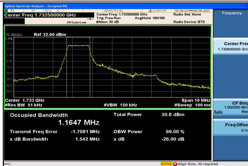
Band4-5MHz-QPSK-20175-6RB#0-1.1647
