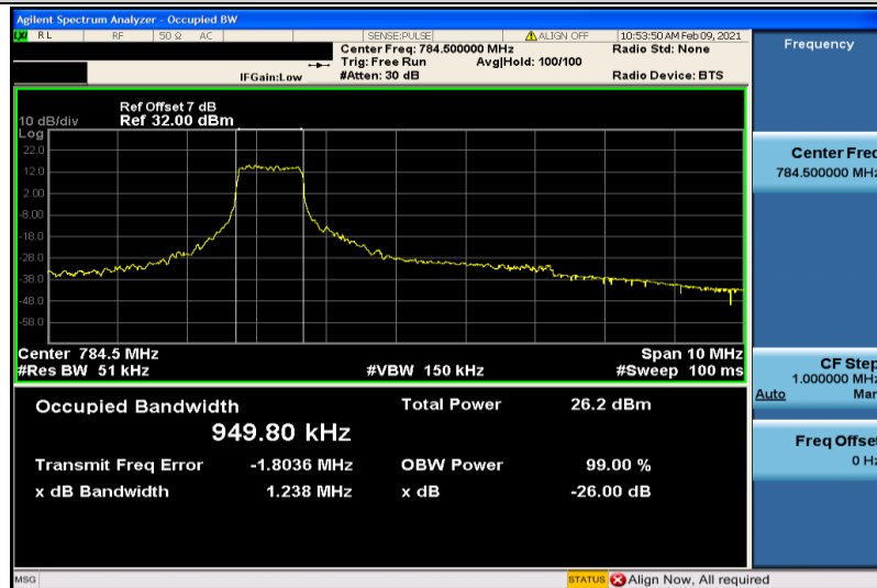
Band13-5MHz-16QAM-23255-6RB#0-0.9498
