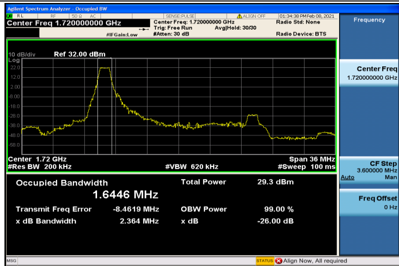
Band4-20MHz-QPSK-20050-6RB#0-1.6446
