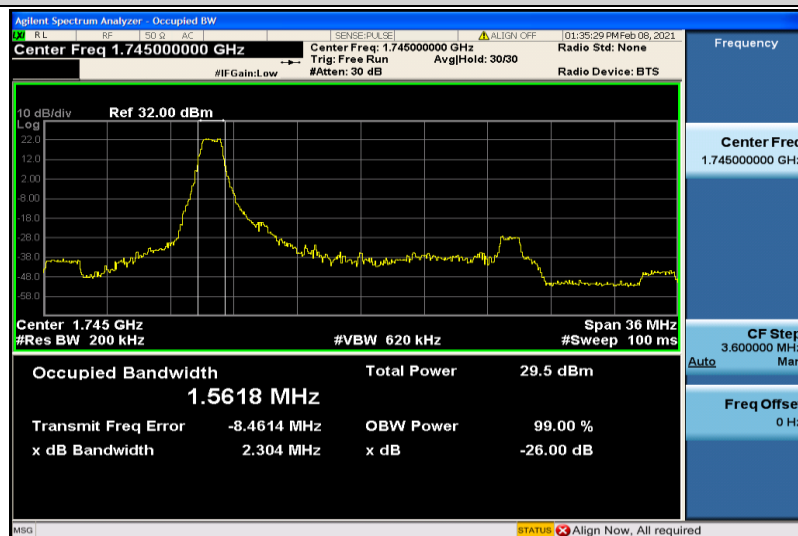
Band4-20MHz-16QAM-20300-6RB#0-1.5618
