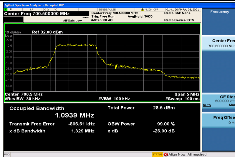
Band12-3MHz-16QAM-23025-6RB#0-1.0939
