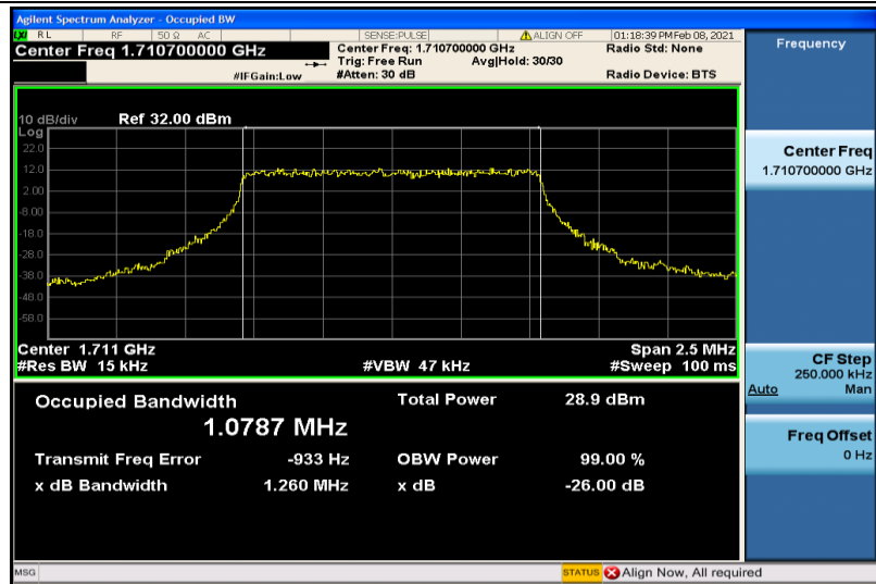
Band4-1.4MHz-QPSK-19957-6RB#0-1.0787
