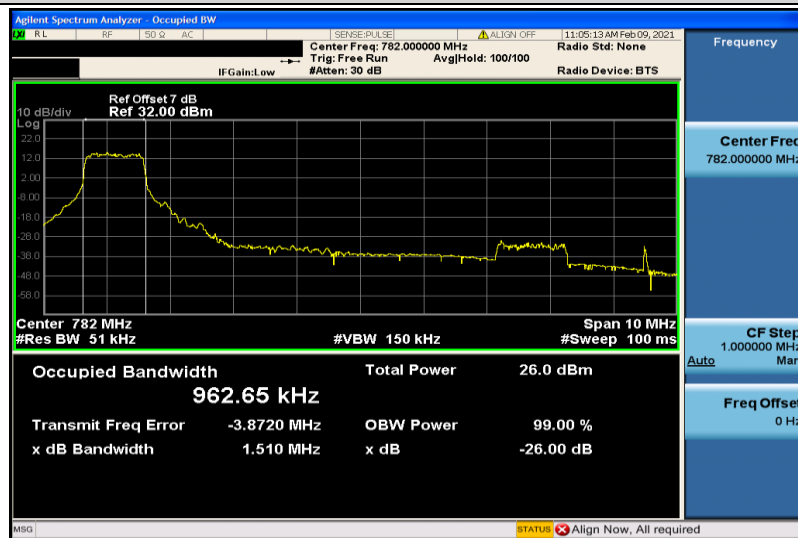
Band13-10MHz-16QAM-23230-6RB#0-0.9627
