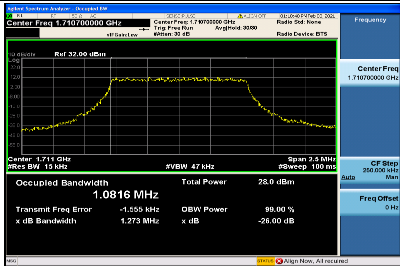
Band4-1.4MHz-16QAM-19957-6RB#0-1.0816
