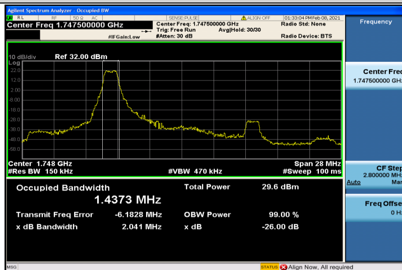
Band4-15MHz-16QAM-20325-6RB#0-1.4373
