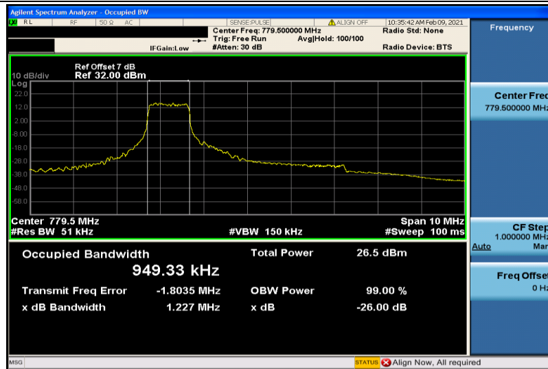
Band13-5MHz-16QAM-23205-6RB#0-0.9493
