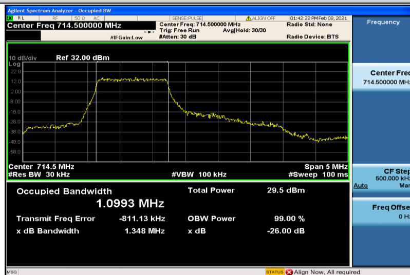
Band12-3MHz-QPSK-23165-6RB#0-1.0993
