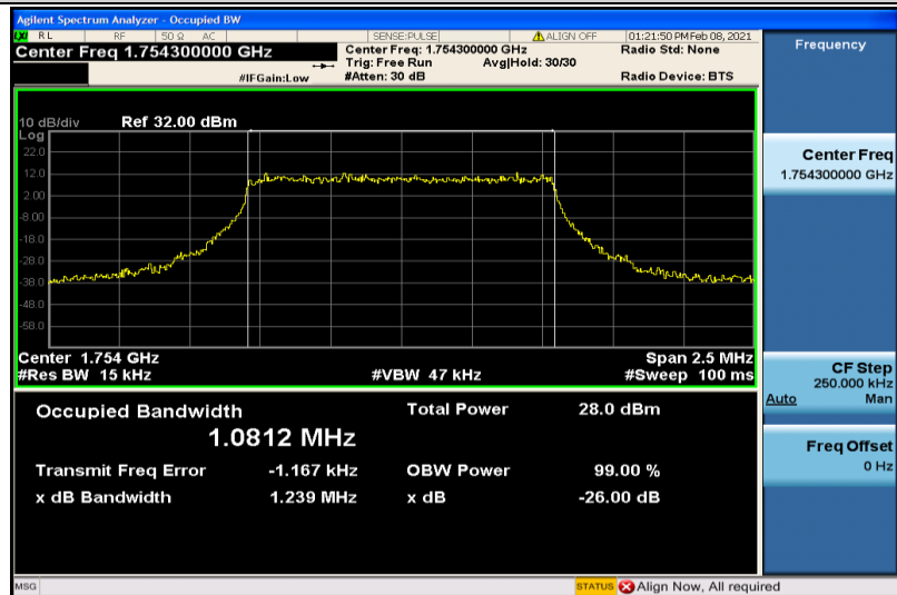
Band4-1.4MHz-16QAM-20393-6RB#0-1.0812
