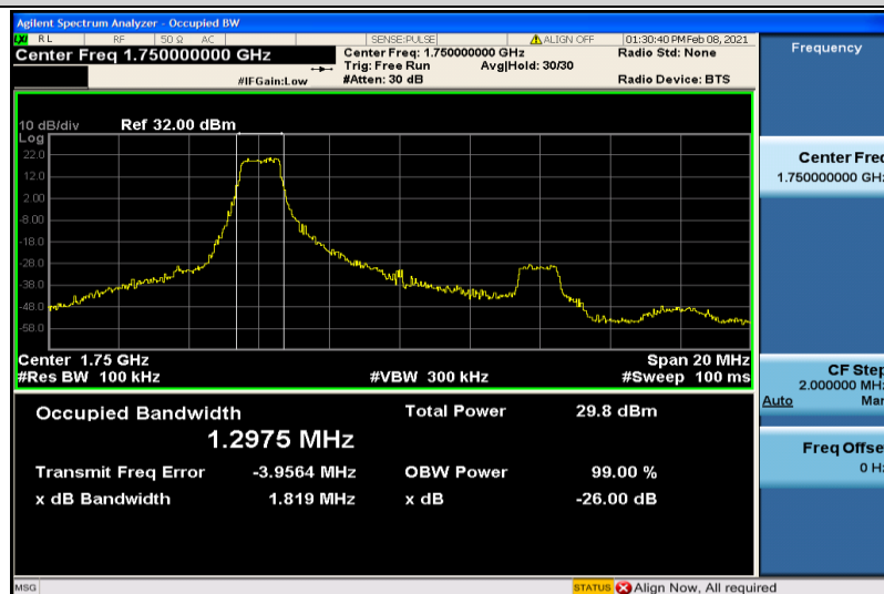
Band4-10MHz-16QAM-20350-6RB#0-1.2975
