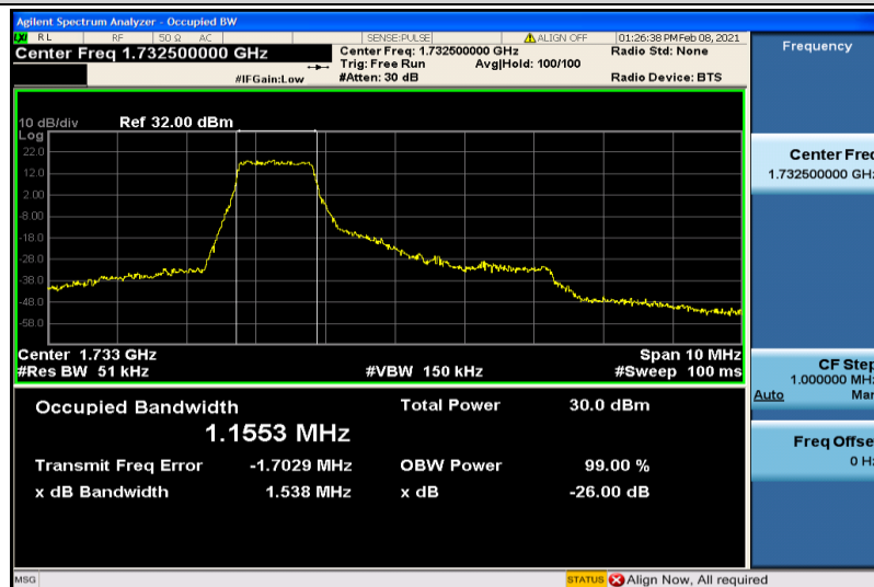
Band4-5MHz-16QAM-20175-6RB#0-1.1553
