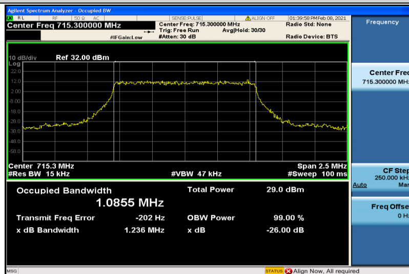
Band12-1.4MHz-QPSK-23173-6RB#0-1.0855
