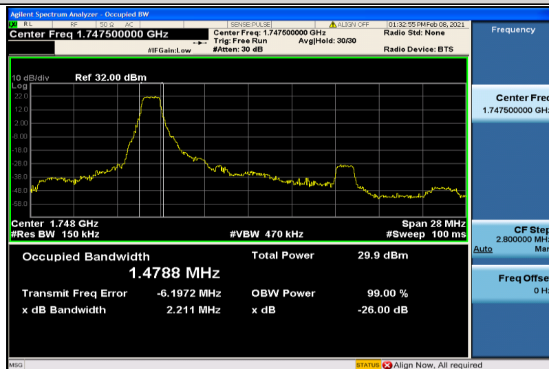
Band4-15MHz-QPSK-20325-6RB#0-1.4788
