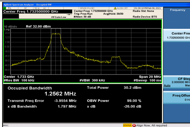
Band4-10MHz-QPSK-20175-6RB#0-1.2562
