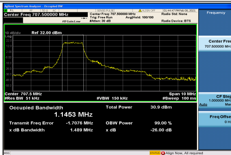
Band12-5MHz-QPSK-23095-6RB#0-1.1453
