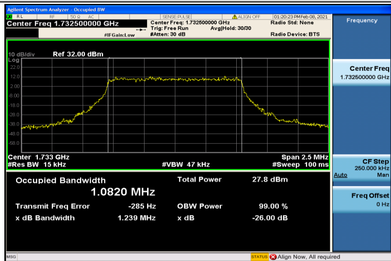
Band4-1.4MHz-16QAM-20175-6RB#0-1.0820
