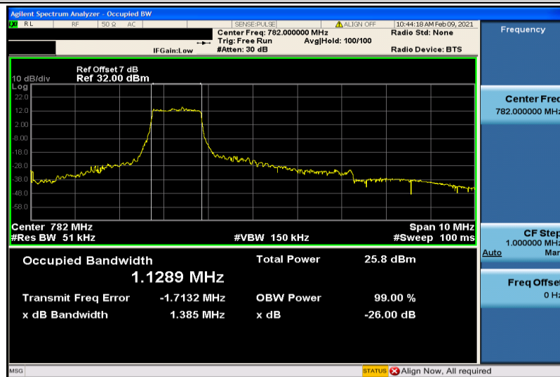
Band13-5MHz-QPSK-23230-6RB#0-1.1289
