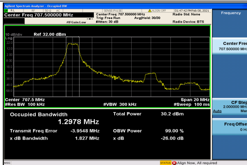
Band12-10MHz-16QAM-23095-6RB#0-1.2978
