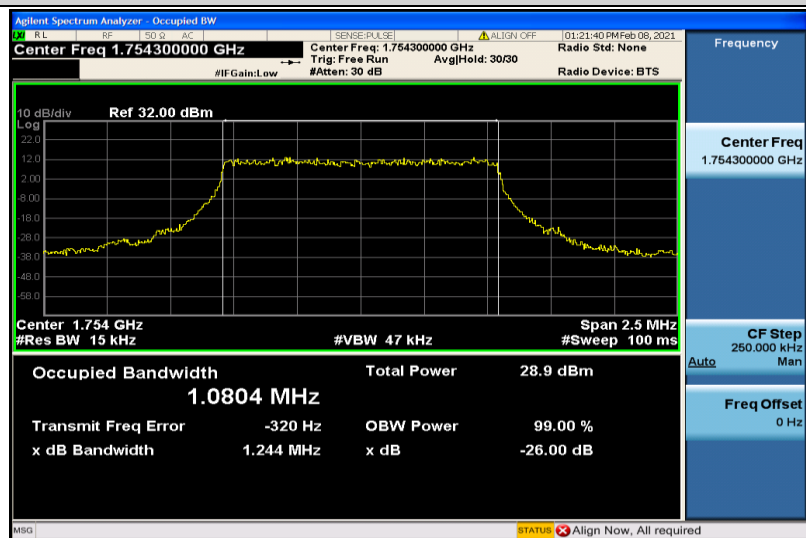
Band4-1.4MHz-QPSK-20393-6RB#0-1.0804
