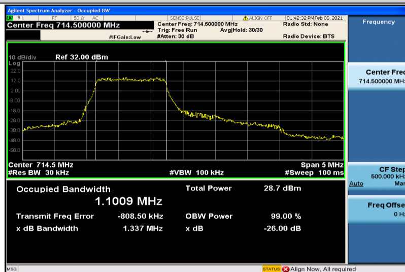
Band12-3MHz-16QAM-23165-6RB#0-1.1009
