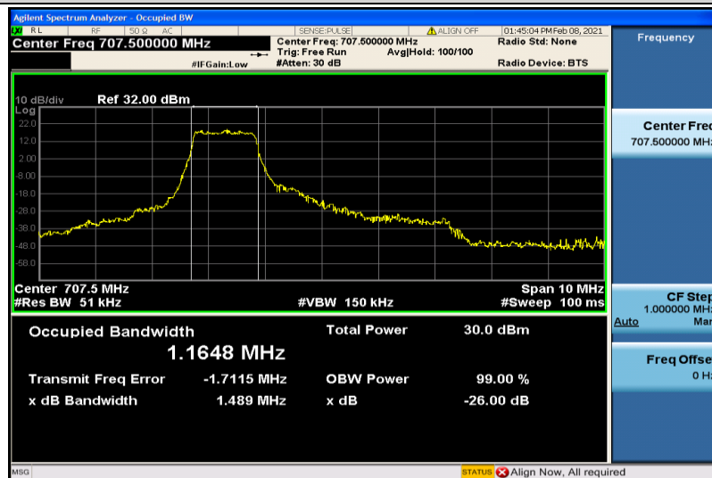
Band12-5MHz-16QAM-23095-6RB#0-1.1648
