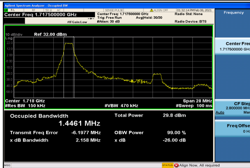
Band4-15MHz-QPSK-20025-6RB#0-1.4461
