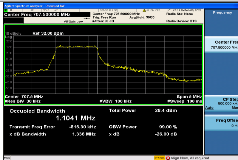
Band12-3MHz-16QAM-23095-6RB#0-1.1041
