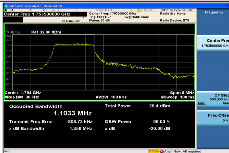
Band4-3MHz-QPSK-20385-6RB#0-1.1033
