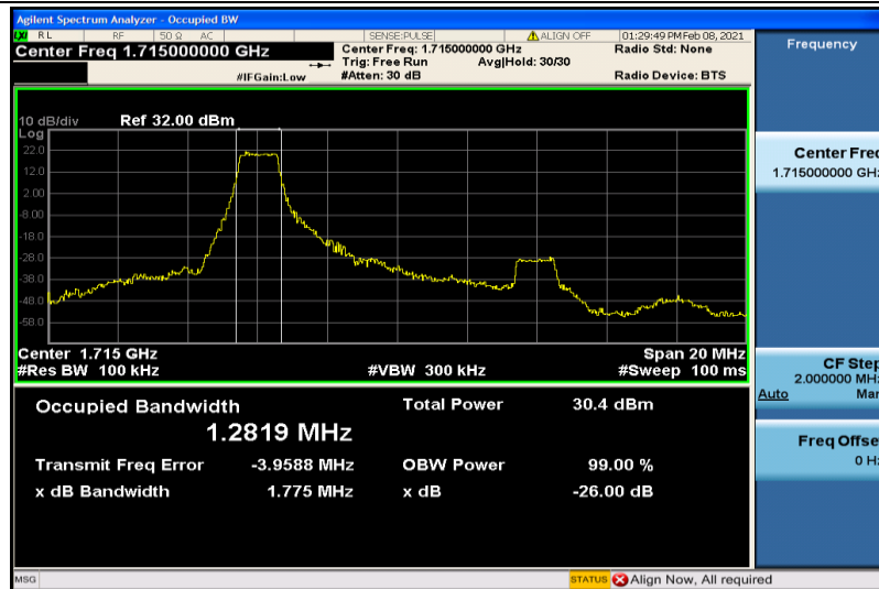
Band4-10MHz-QPSK-20000-6RB#0-1.2819
