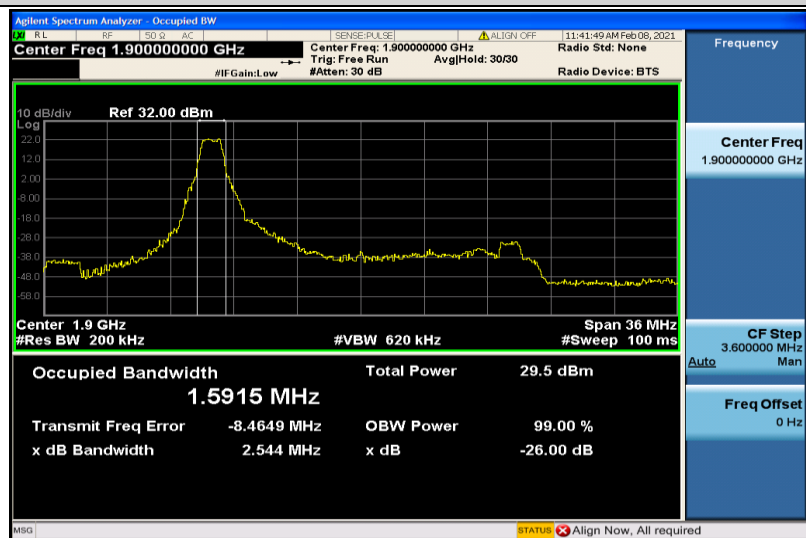
Band2-20MHz-16QAM-19100-6RB#0-1.5915
