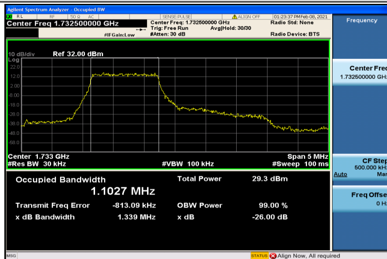
Band4-3MHz-QPSK-20175-6RB#0-1.1027
