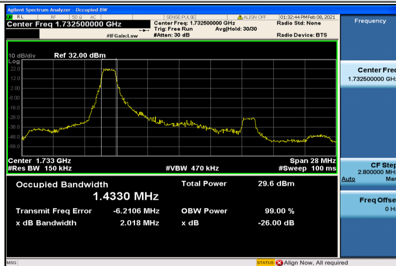
Band4-15MHz-16QAM-20175-6RB#0-1.4330
