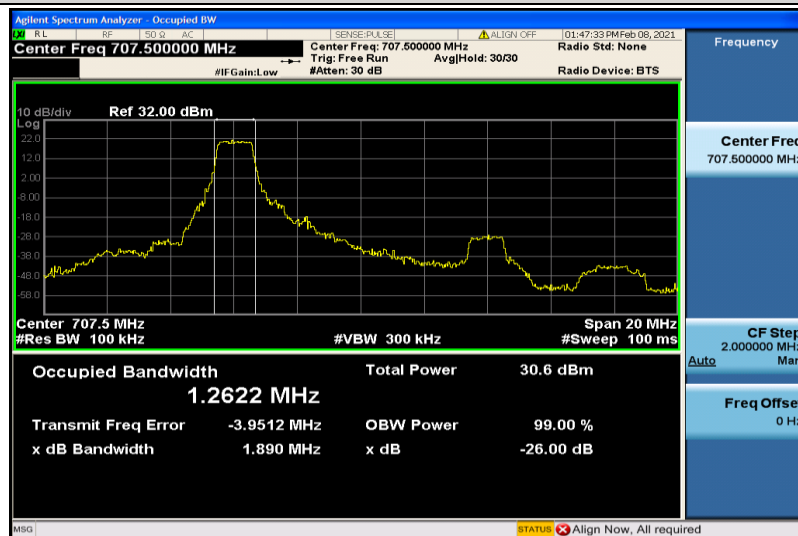
Band12-10MHz-QPSK-23095-6RB#0-1.2622
