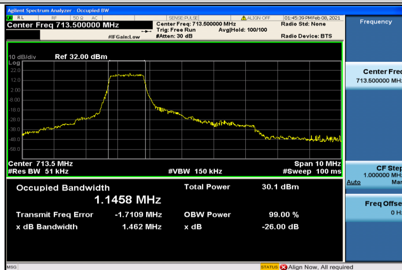
Band12-5MHz-16QAM-23155-6RB#0-1.1458
