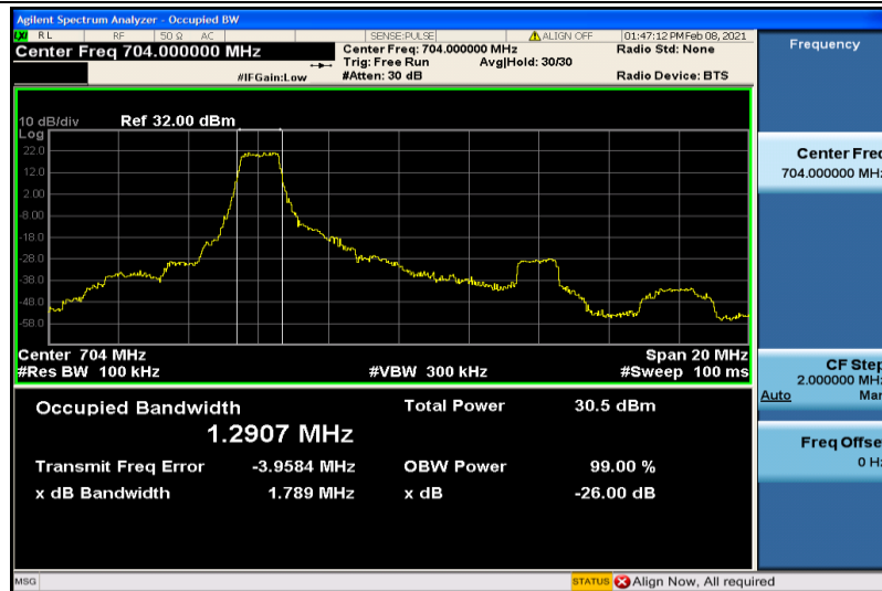
Band12-10MHz-QPSK-23060-6RB#0-1.2907
