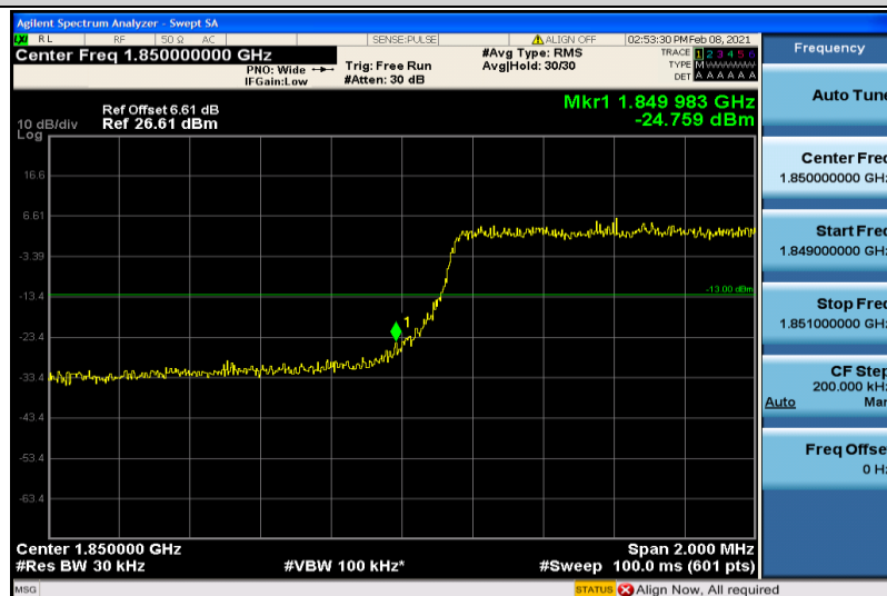
Band2-3MHz-16QAM-18615-6RB#0
