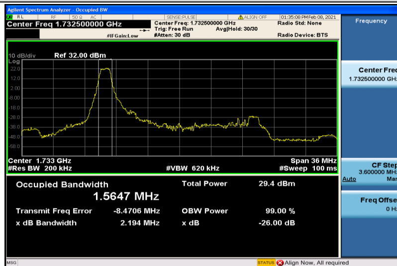
Band4-20MHz-16QAM-20175-6RB#0-1.5647
