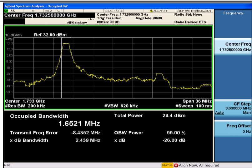
Band4-20MHz-QPSK-20175-6RB#0-1.6521
