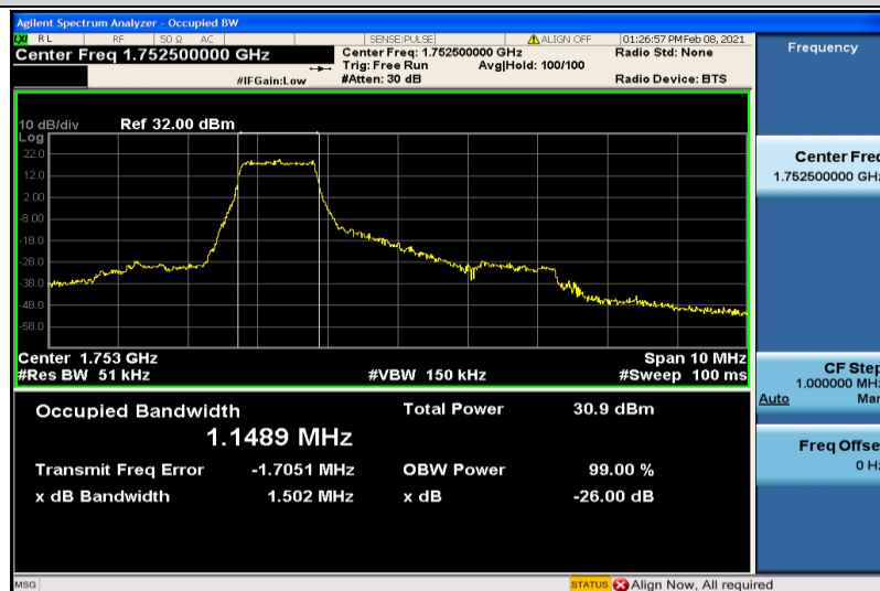
Band4-5MHz-QPSK-20375-6RB#0-1.1489
