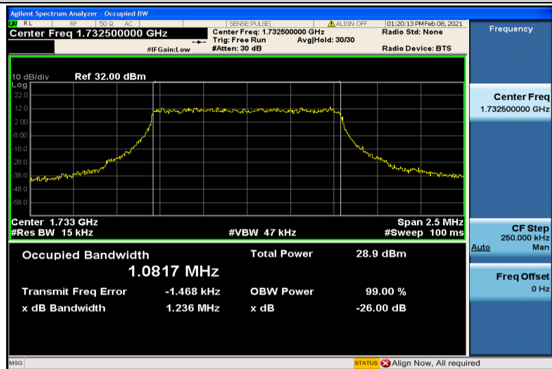
Band4-1.4MHz-QPSK-20175-6RB#0-1.0817
