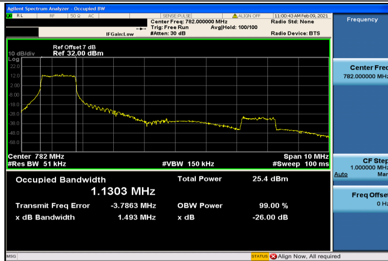
Band13-10MHz-QPSK-23230-6RB#0-1.1303
