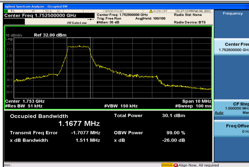
Band4-5MHz-16QAM-20375-6RB#0-1.1677
