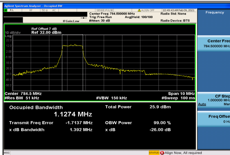
Band13-5MHz-QPSK-23255-6RB#0-1.1274
