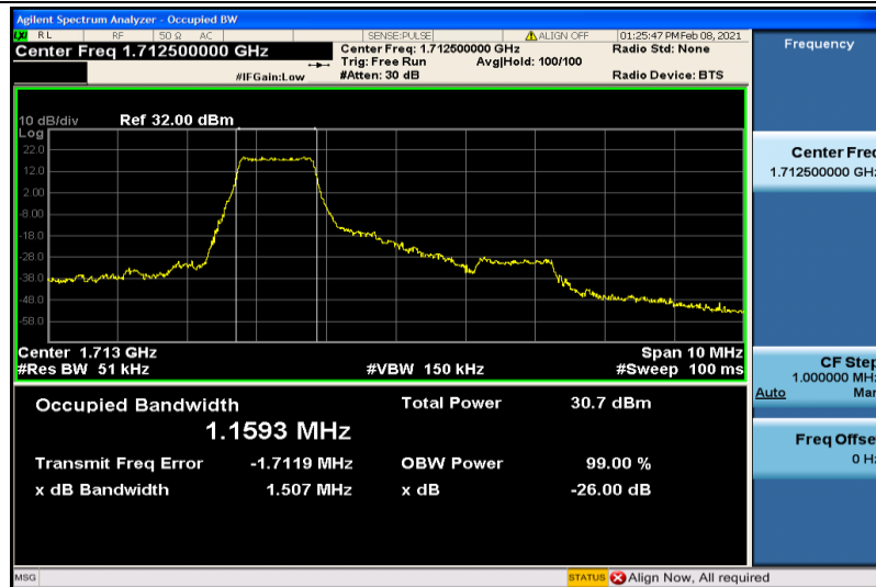
Band4-5MHz-QPSK-19975-6RB#0-1.1593
