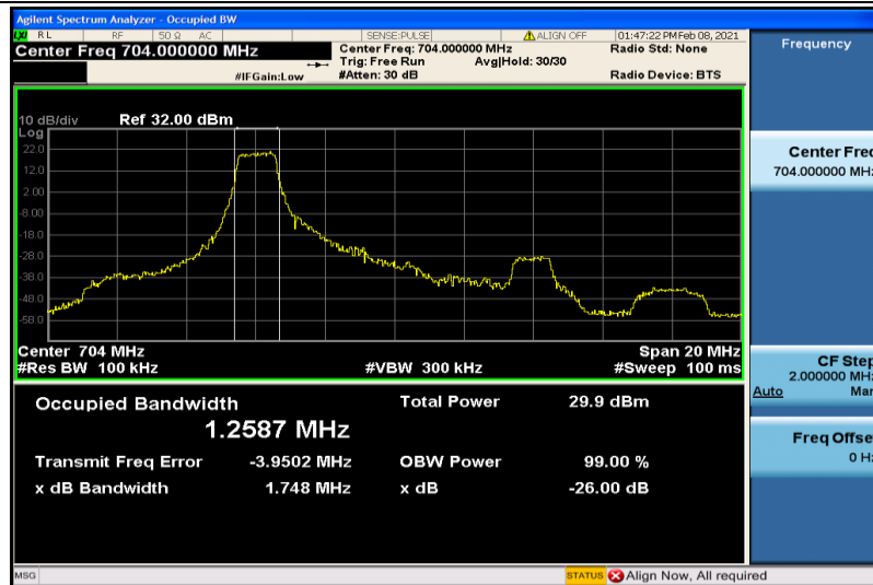
Band12-10MHz-16QAM-23060-6RB#0-1.2587
