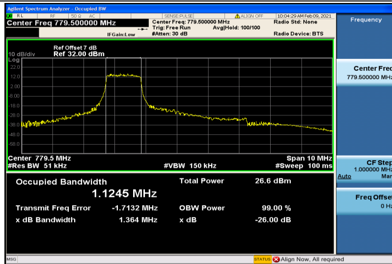
Band13-5MHz-QPSK-23205-6RB#0-1.1245
