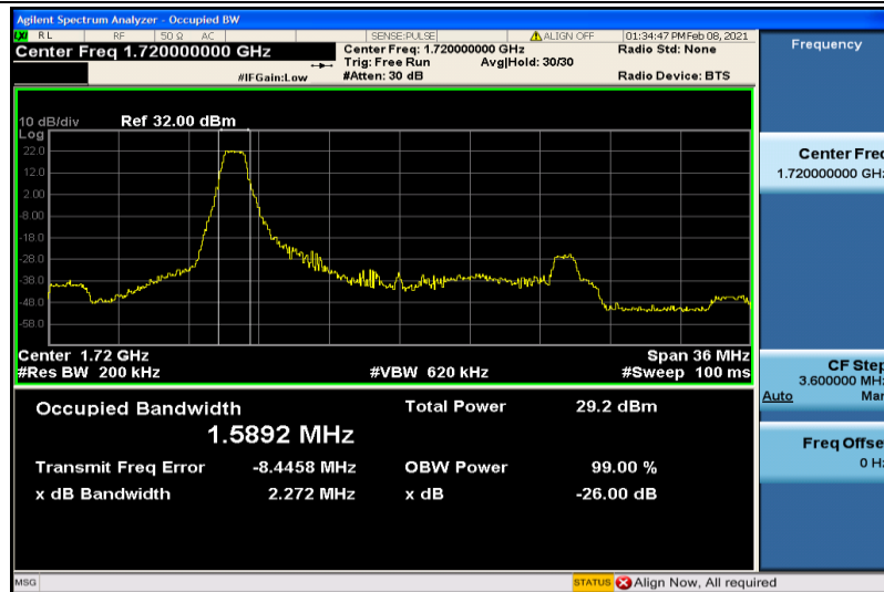
Band4-20MHz-16QAM-20050-6RB#0-1.5892
