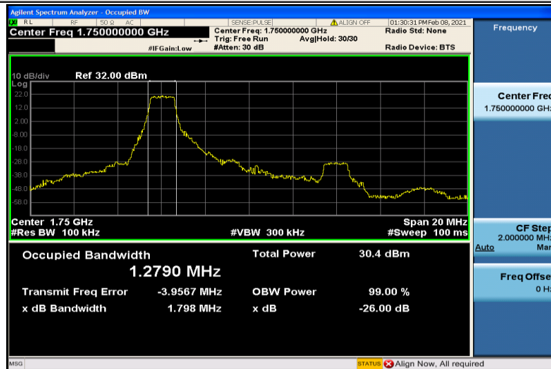
Band4-10MHz-QPSK-20350-6RB#0-1.2790
