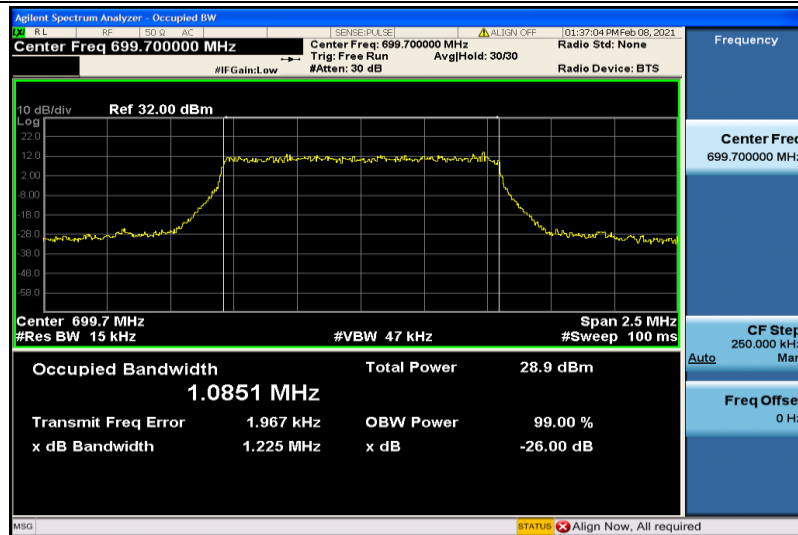
Band12-1.4MHz-QPSK-23017-6RB#0-1.0851
