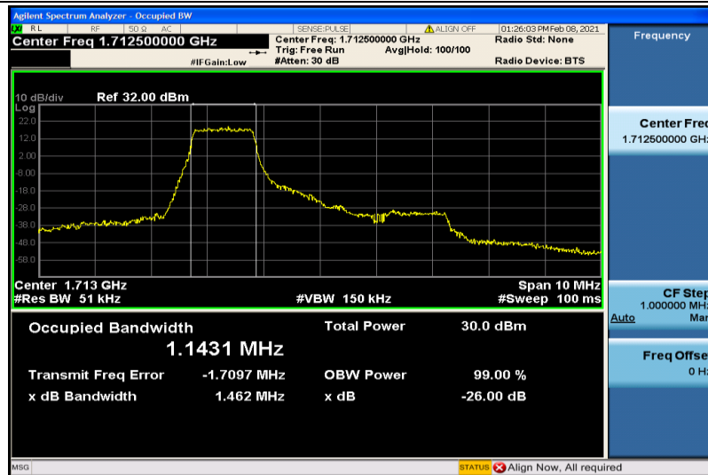
Band4-5MHz-16QAM-19975-6RB#0-1.1431
