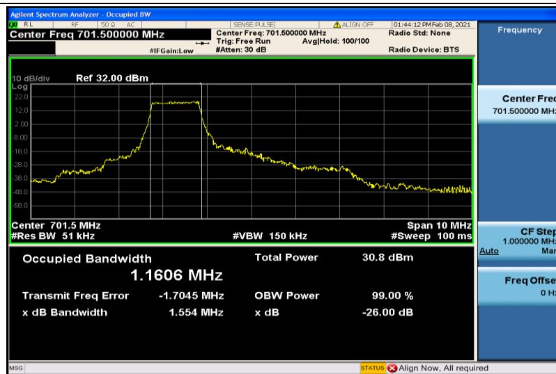
Band12-5MHz-QPSK-23035-6RB#0-1.1606
