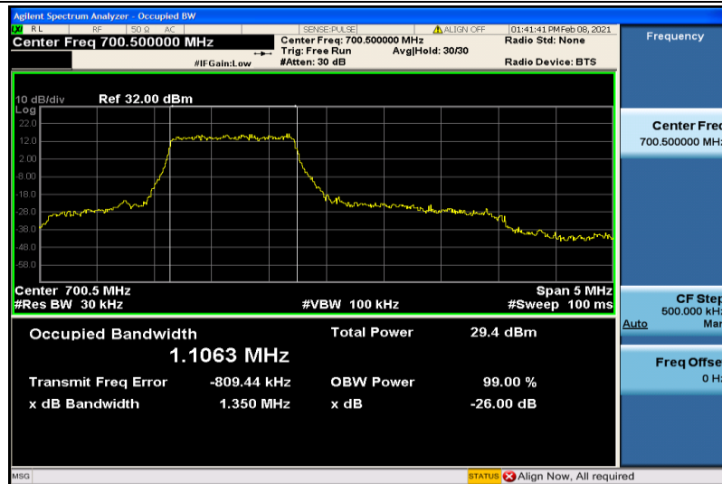
Band12-3MHz-QPSK-23025-6RB#0-1.1063
