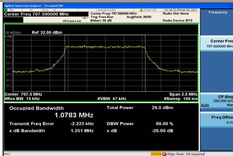
Band12-1.4MHz-QPSK-23095-6RB#0-1.0783
