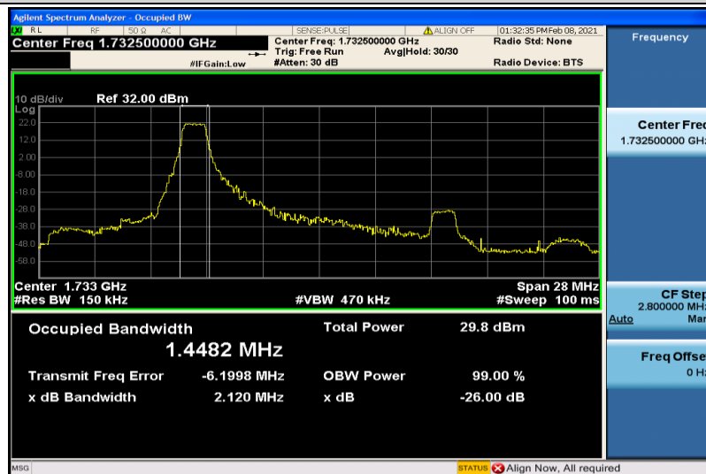
Band4-15MHz-QPSK-20175-6RB#0-1.4482
