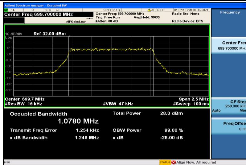
Band12-1.4MHz-16QAM-23017-6RB#0-1.0780
