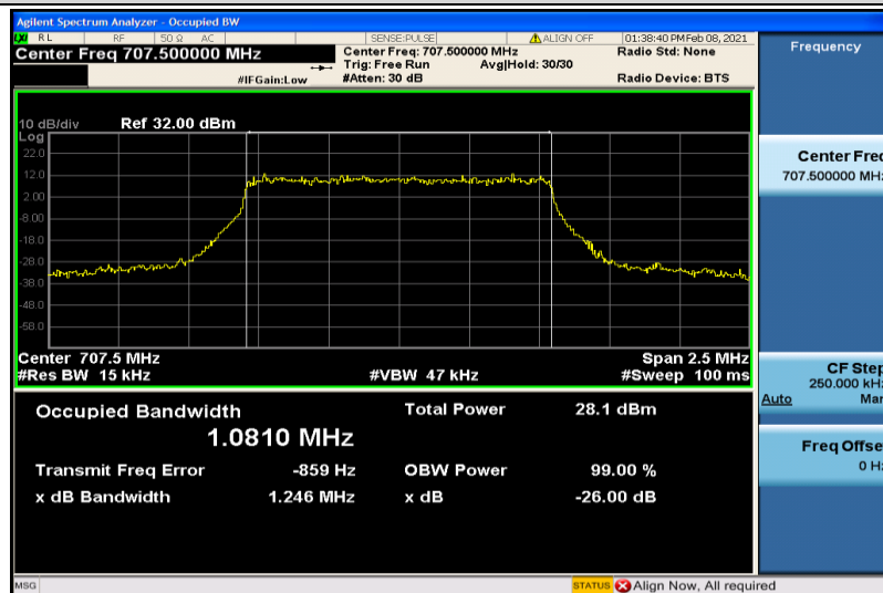
Band12-1.4MHz-16QAM-23095-6RB#0-1.0810
