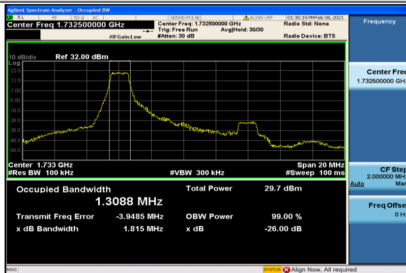
Band4-10MHz-16QAM-20175-6RB#0-1.3088
