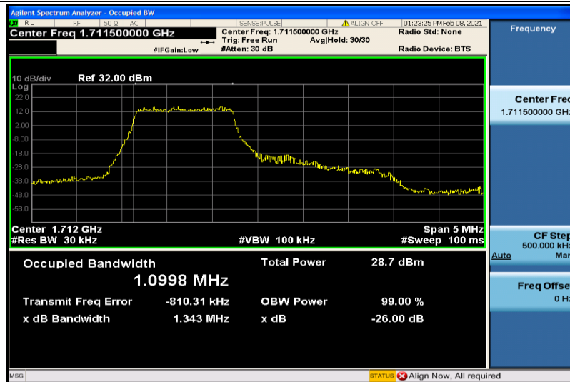
Band4-3MHz-16QAM-19965-6RB#0-1.0998
