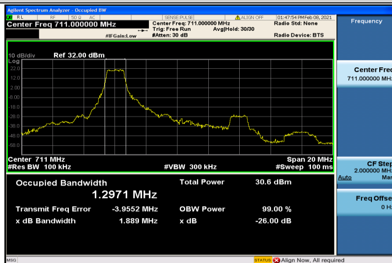
Band12-10MHz-QPSK-23130-6RB#0-1.2971
