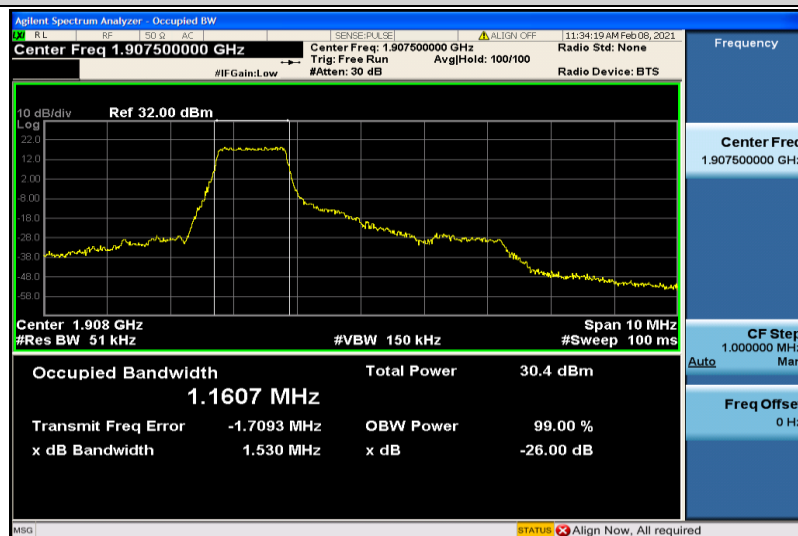
Band2-5MHz-QPSK-19175-6RB#0-1.1607
