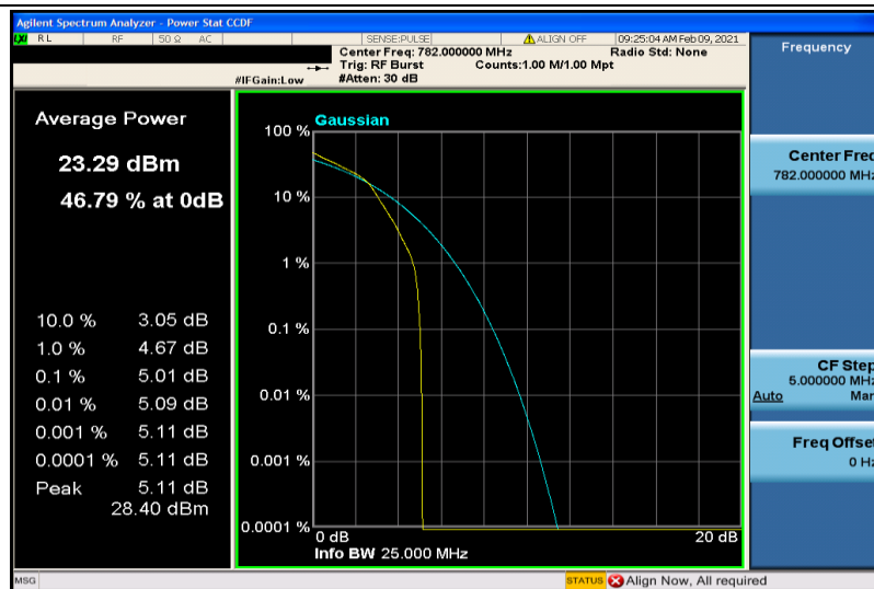
Band13-5MHz-16QAM-23230-6RB#0
