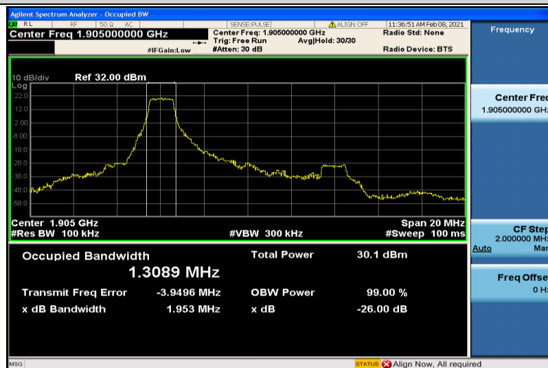
Band2-10MHz-QPSK-19150-6RB#0-1.3089
