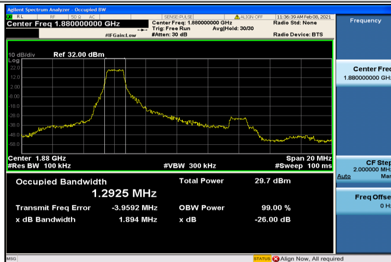
Band2-10MHz-16QAM-18900-6RB#0-1.2925
