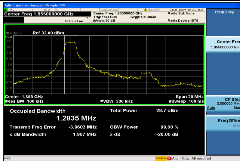
Band2-10MHz-16QAM-18650-6RB#0-1.2835
