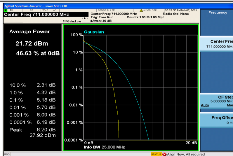
Band12-10MHz-QPSK-23130-6RB#0
