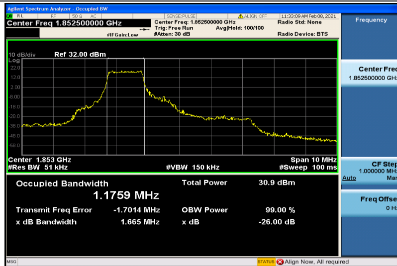
Band2-5MHz-QPSK-18625-6RB#0-1.1759
