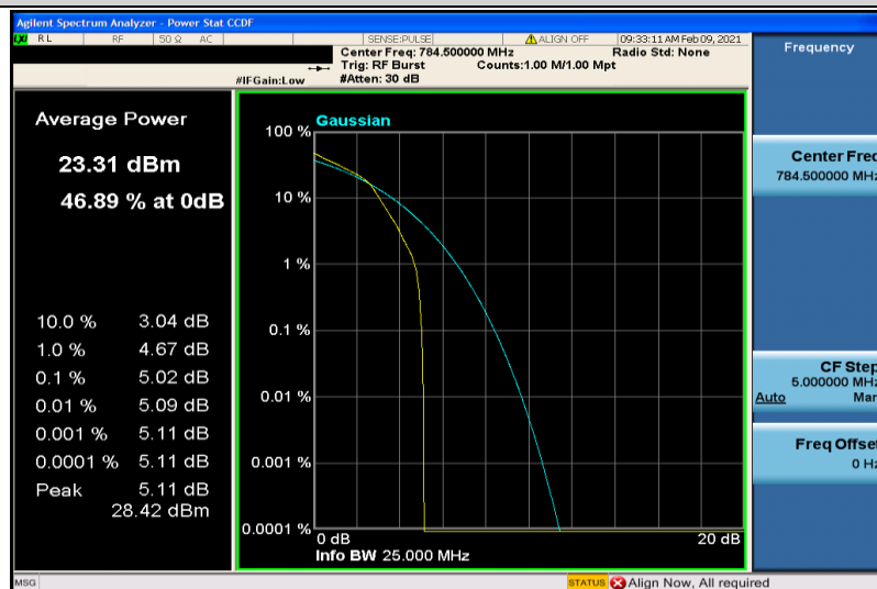
Band13-5MHz-16QAM-23255-6RB#0
