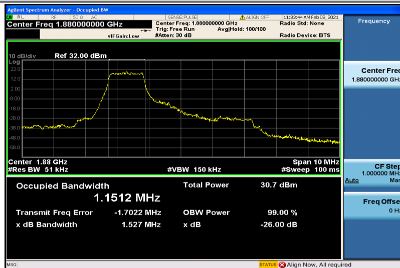
Band2-5MHz-QPSK-18900-6RB#0-1.1512
