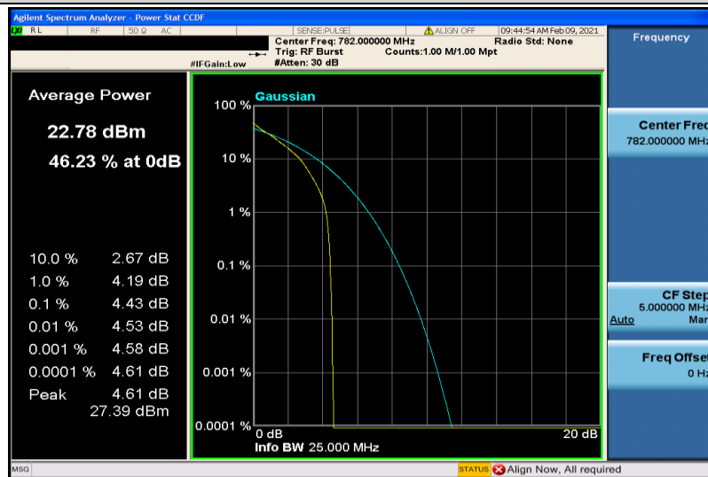
Band13-10MHz-QPSK-23230-6RB#0
