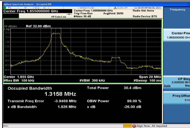
Band2-10MHz-QPSK-18650-6RB#0-1.3158
