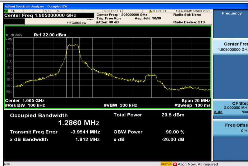
Band2-10MHz-16QAM-19150-6RB#0-1.2860
