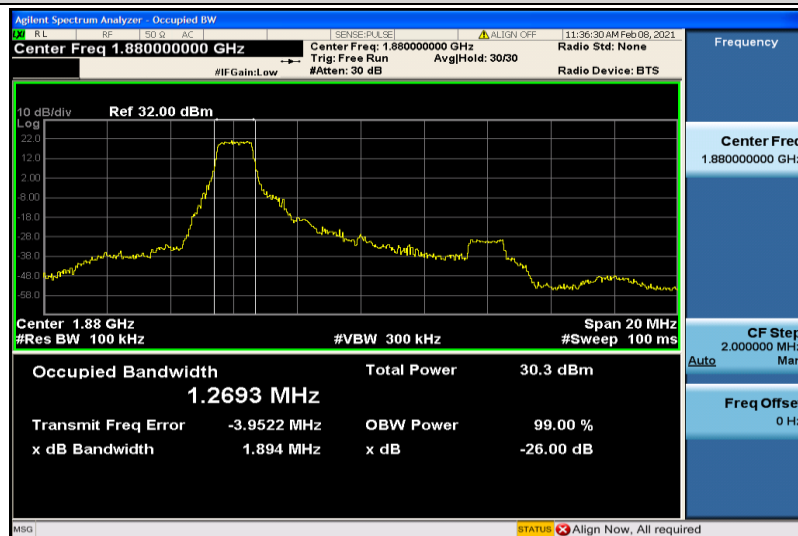
Band2-10MHz-QPSK-18900-6RB#0-1.2693
