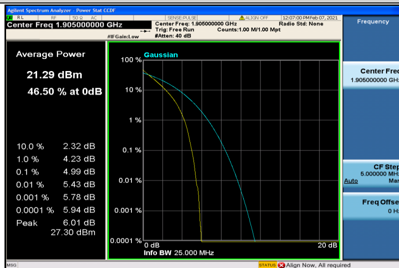
Band2-10MHz-QPSK-19150-6RB#0
