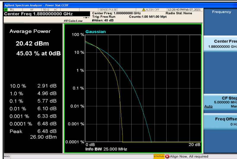
Band2-15MHz-16QAM-18900-6RB#0
