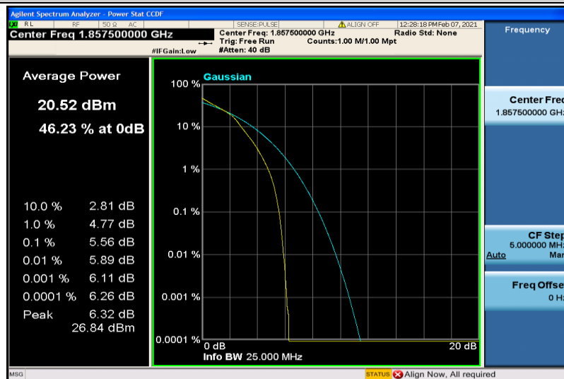
Band2-15MHz-16QAM-18675-6RB#0
