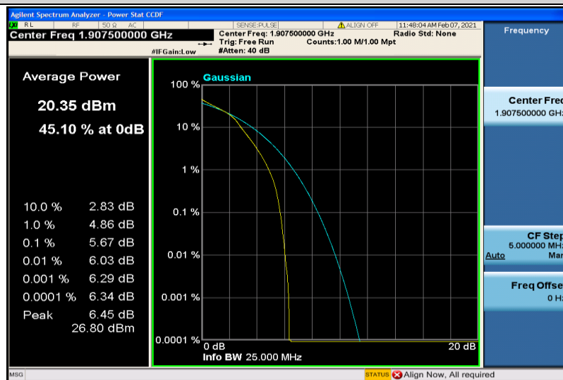
Band2-5MHz-16QAM-19175-6RB#0
