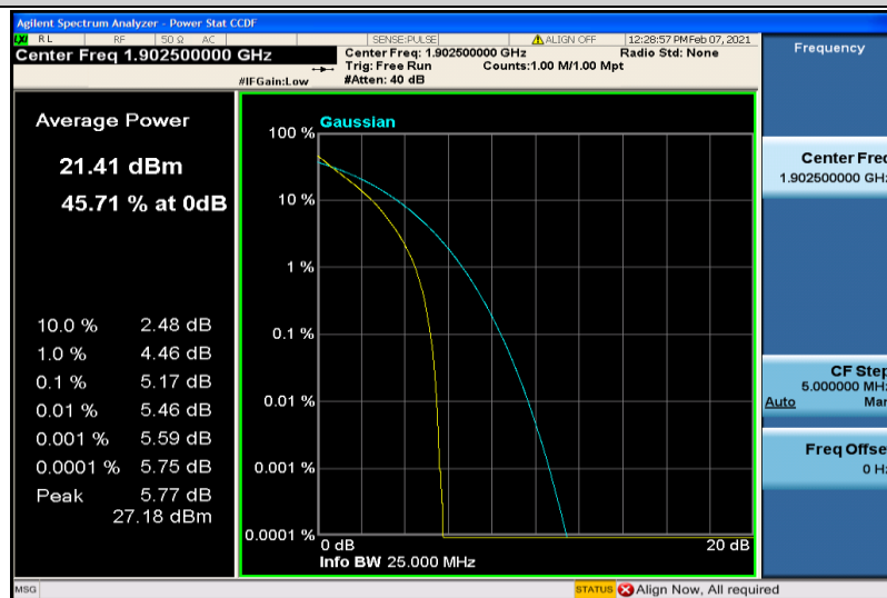
Band2-15MHz-QPSK-19125-6RB#0
