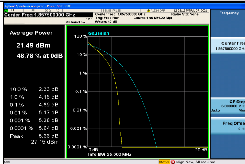
Band2-15MHz-QPSK-18675-6RB#0
