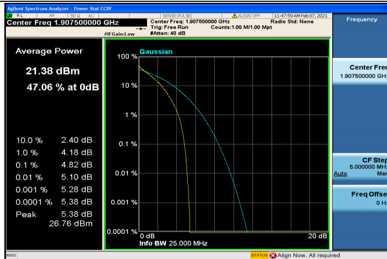
Band2-5MHz-QPSK-19175-6RB#0
