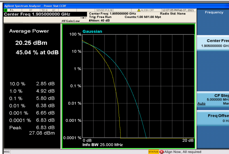
Band2-10MHz-16QAM-19150-6RB#0
