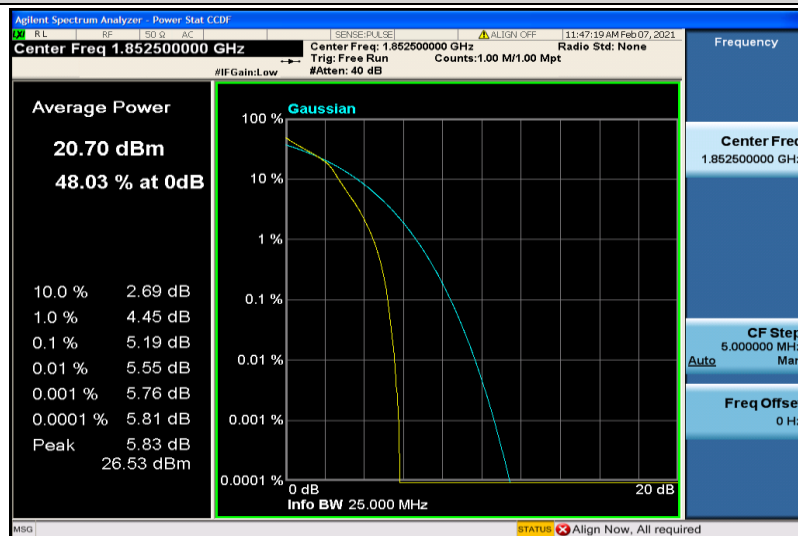
Band2-5MHz-16QAM-18625-6RB#0
