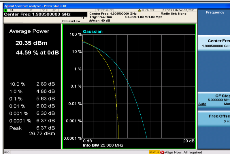
Band2-3MHz-16QAM-19185-6RB#0
