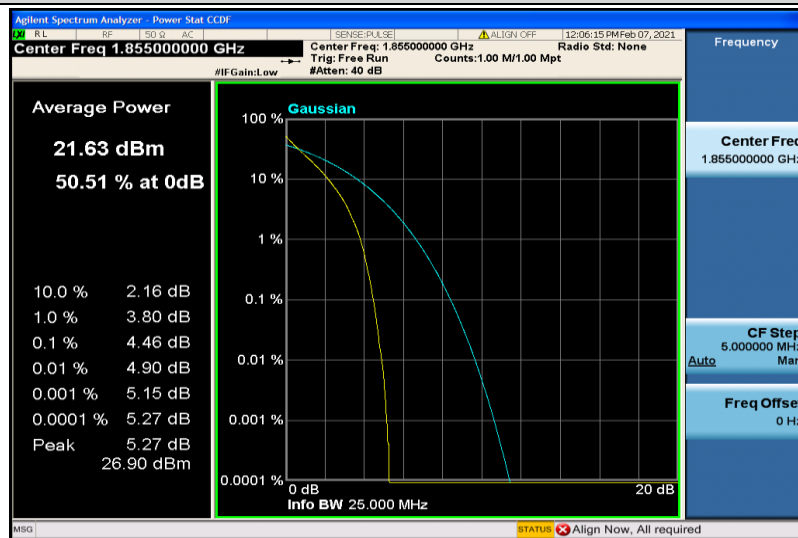
Band2-10MHz-QPSK-18650-6RB#0
