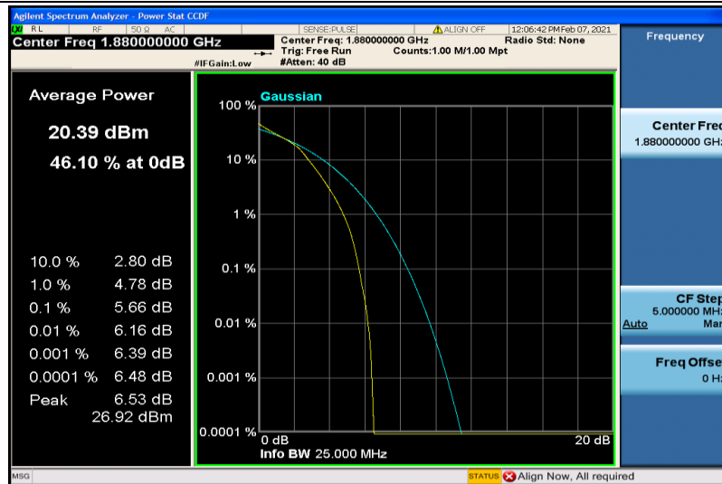
Band2-10MHz-16QAM-18900-6RB#0
