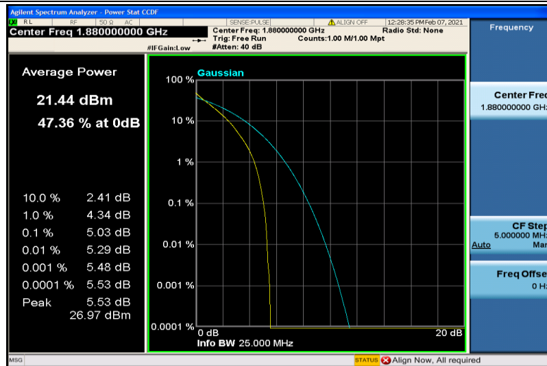
Band2-15MHz-QPSK-18900-6RB#0
