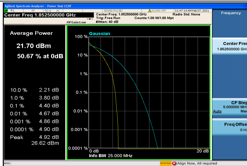
Band2-5MHz-QPSK-18625-6RB#0
