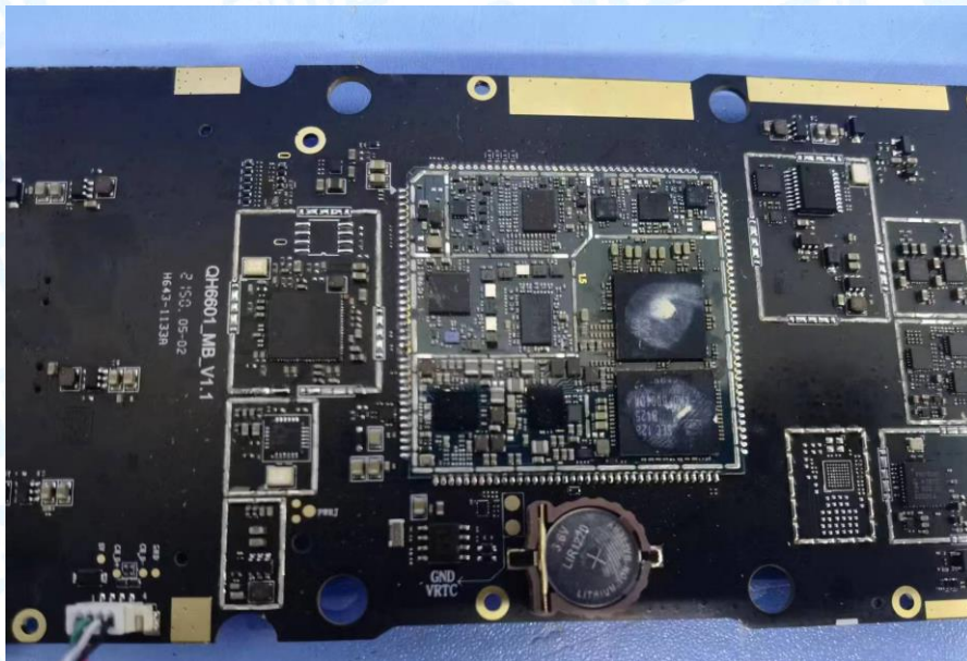
Photo 24 Appearance of EUT
