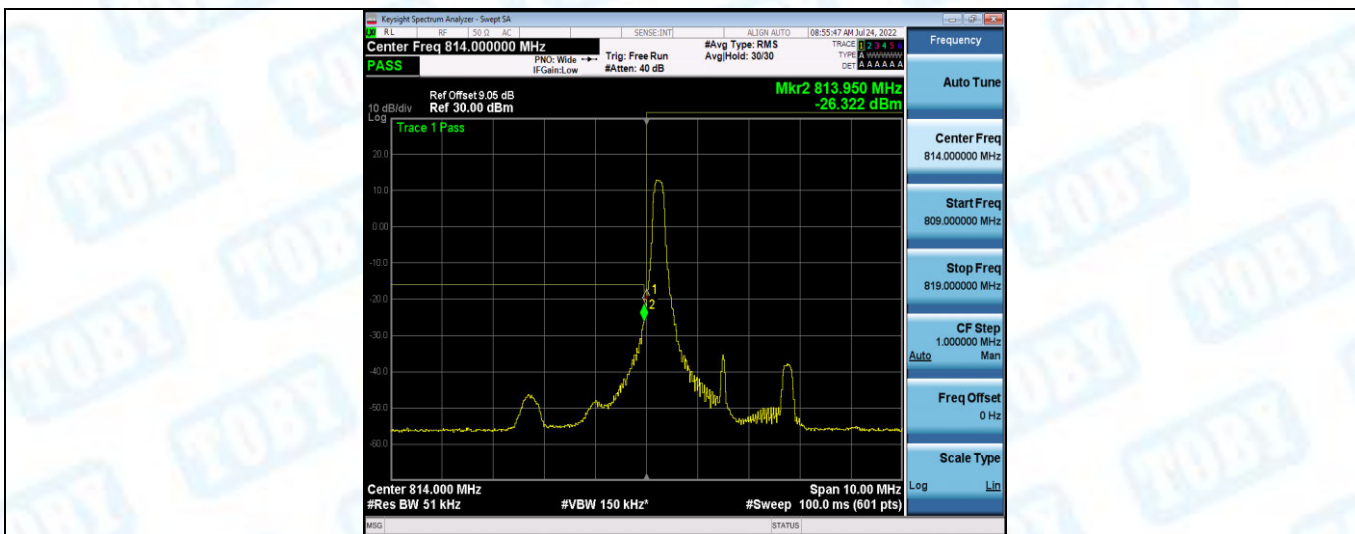
Band26-3MHz-QPSK-26705-1RB#14
