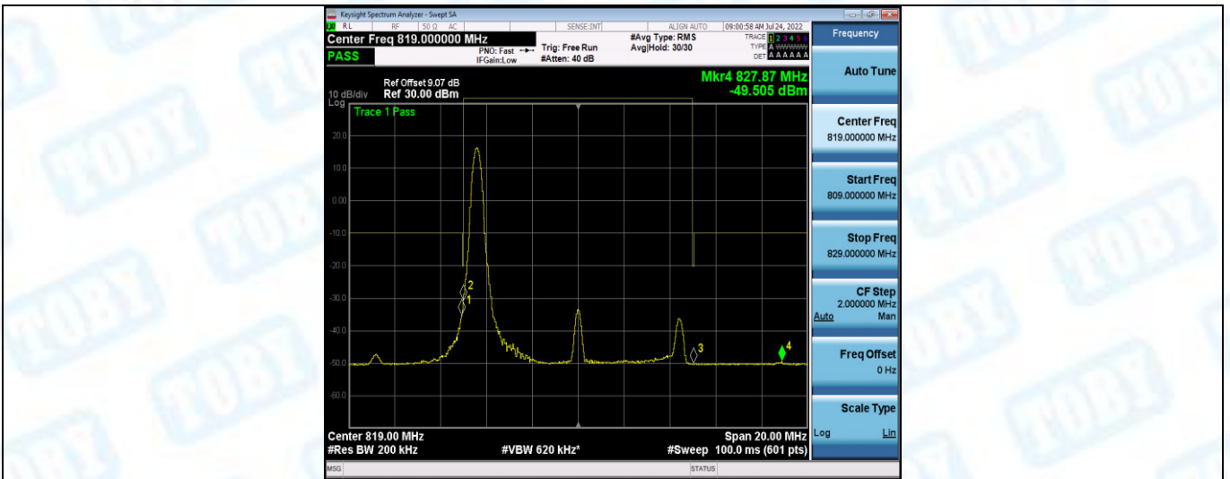
Band26-10MHz-16QAM-26740-1RB#49
