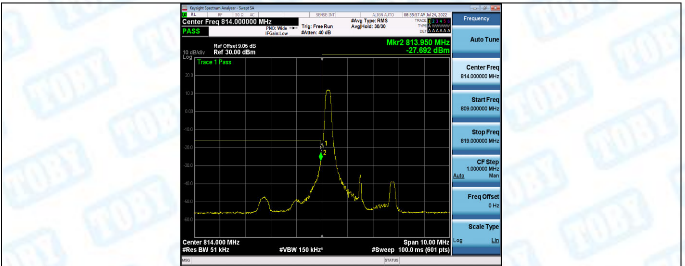
Band26-3MHz-16QAM-26705-1RB#14
