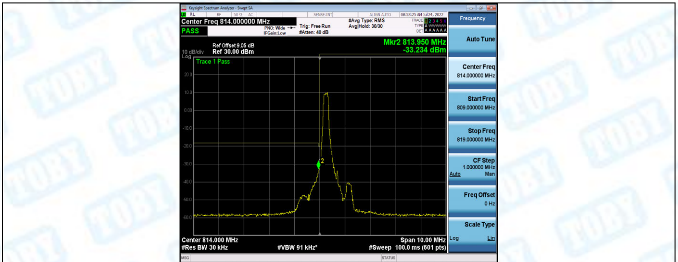
Band26-1.4MHz-16QAM-26697-1RB#5
