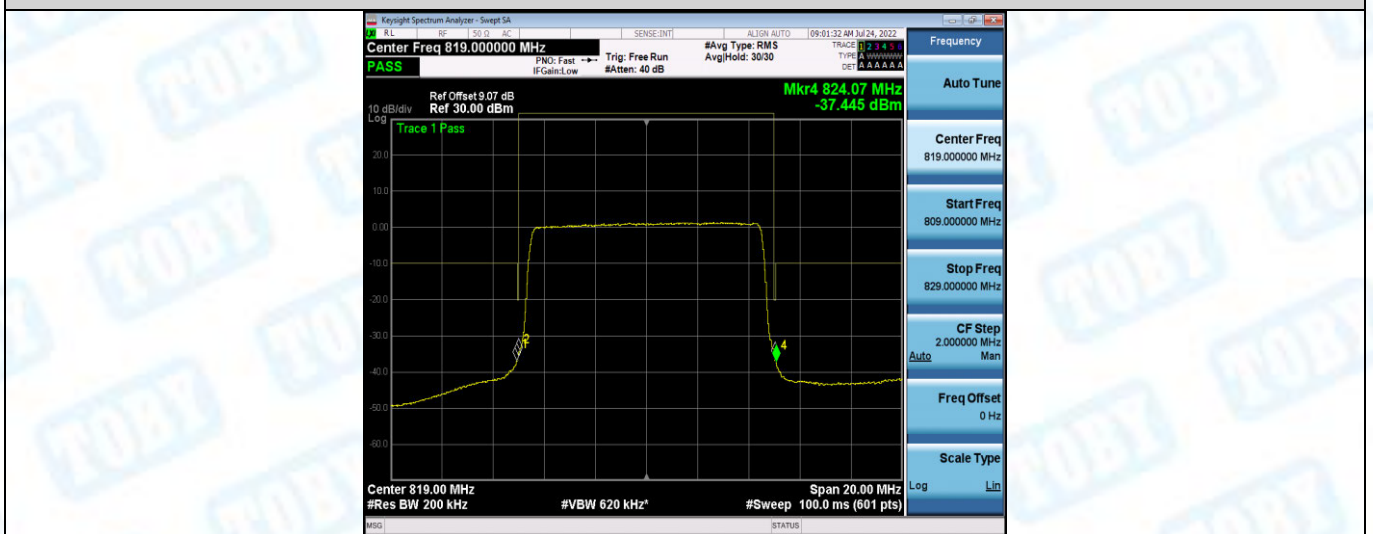
Band26-10MHz-16QAM-26740-1RB#0
