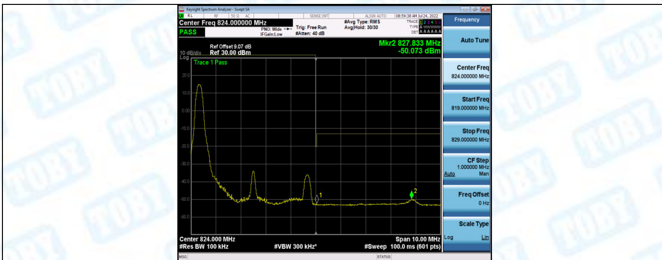
Band26-5MHz-16QAM-26765-1RB#24
