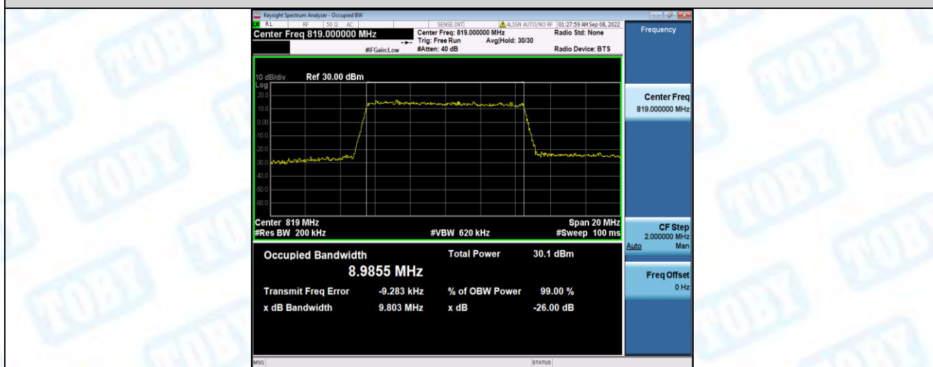
Band26-10MHz-16QAM-26740-50RB#0
