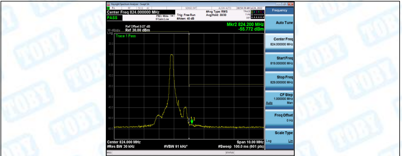
Band26-1.4MHz-16QAM-26783-1RB#5
