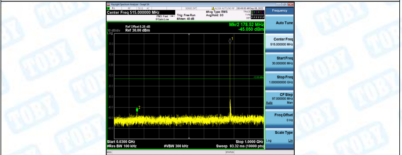
Band13-5MHz-16QAM-23230-1RB#0-Range1:30~1000MHz
