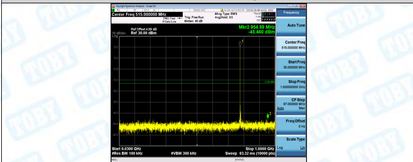
Band13-5MHz-16QAM-23255-1RB#0-Range2:30~1000MHz
