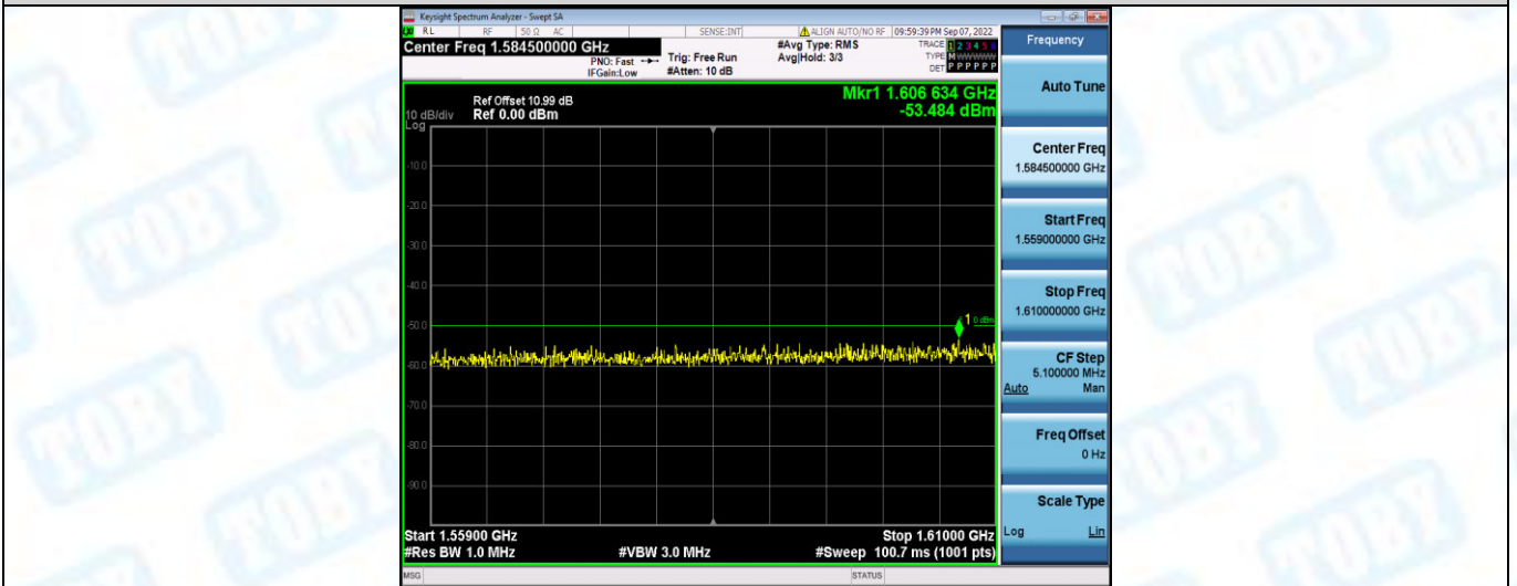
Band13-5MHz-16QAM-23205-1RB#0-Range1:1559~1610MHz
