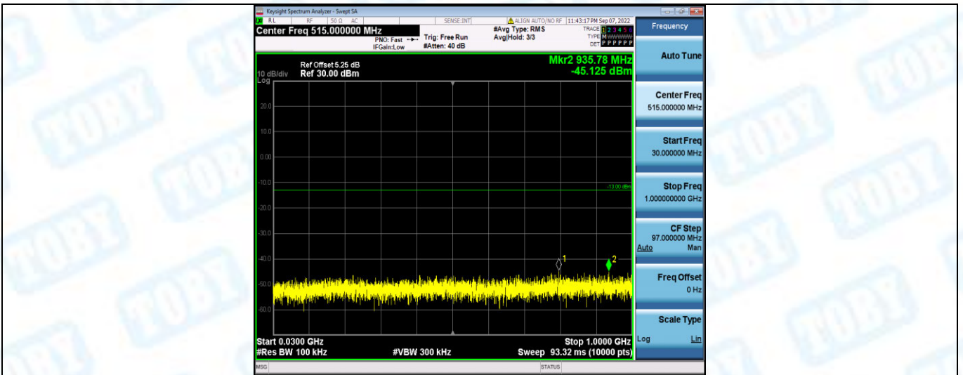
Band13-5MHz-QPSK-23205-1RB#0-Range2:30~1000MHz
