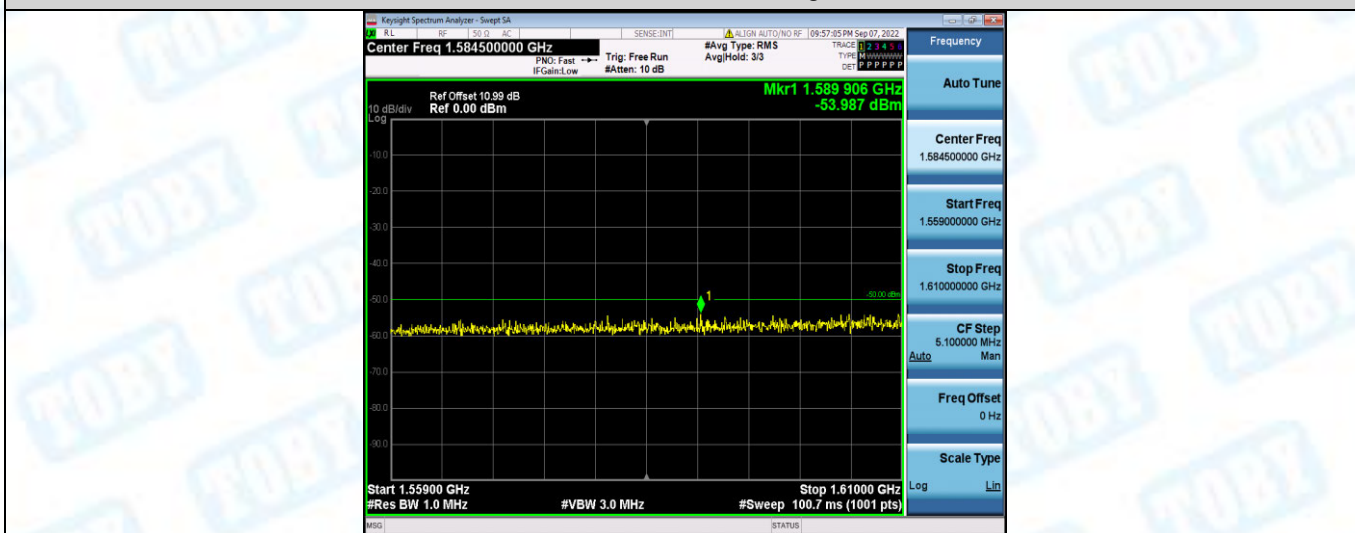
Band13-5MHz-QPSK-23205-1RB#0-Range1:1559~1610MHz
