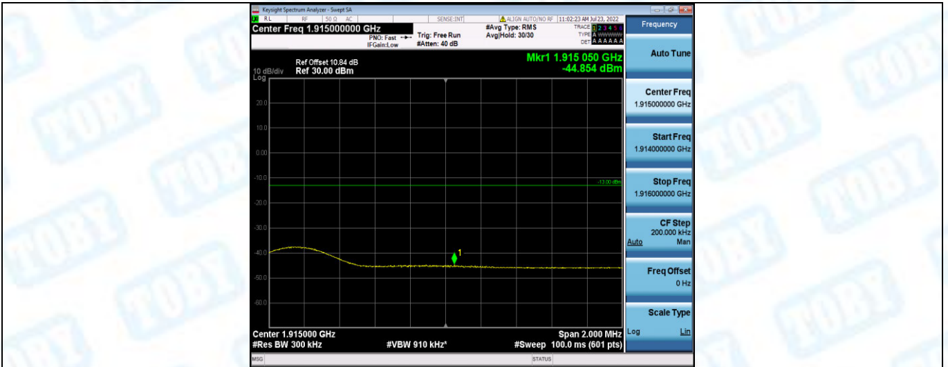
Band25-15MHz-16QAM-26615-1RB#74
