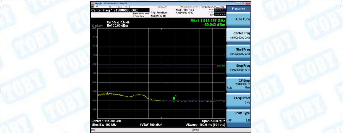
Band25-5MHz-QPSK-26665-1RB#24
