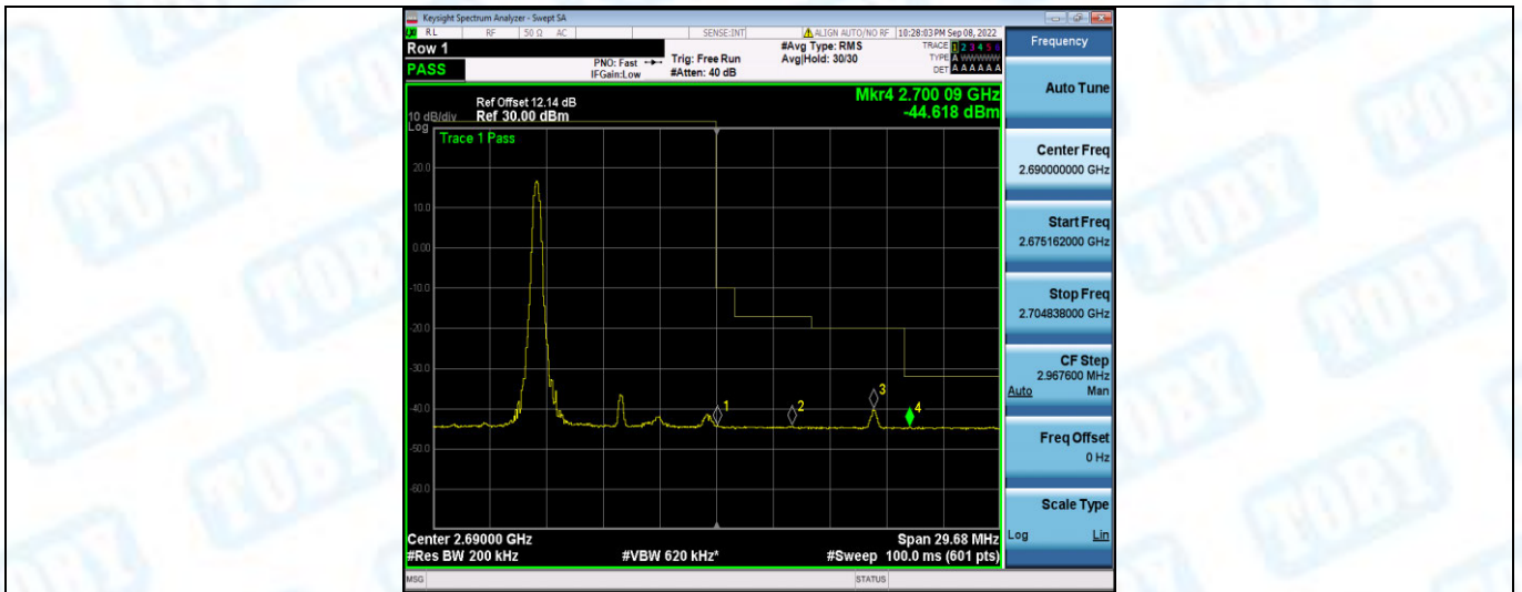
Band41-10MHz-QPSK-41540-1RB#49
