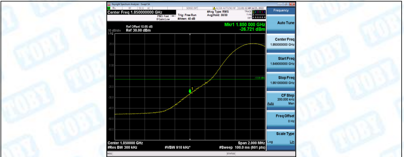
Band25-15MHz-16QAM-26115-1RB#74
