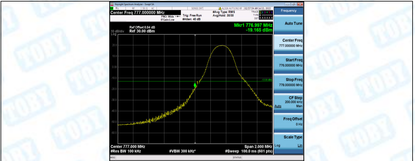
Band13-5MHz-16QAM-23205-1RB#24
