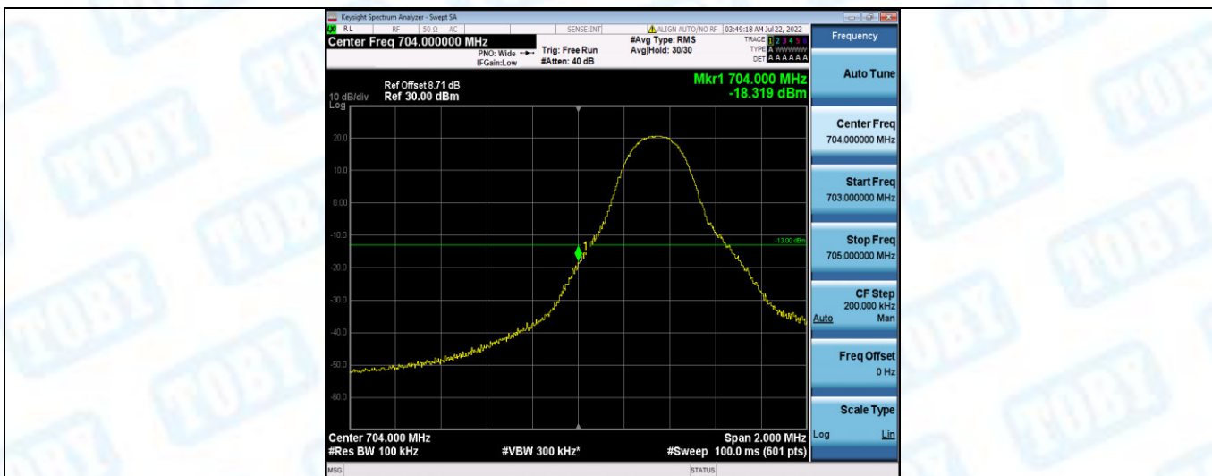
Band17-5MHz-16QAM-23755-1RB#24
