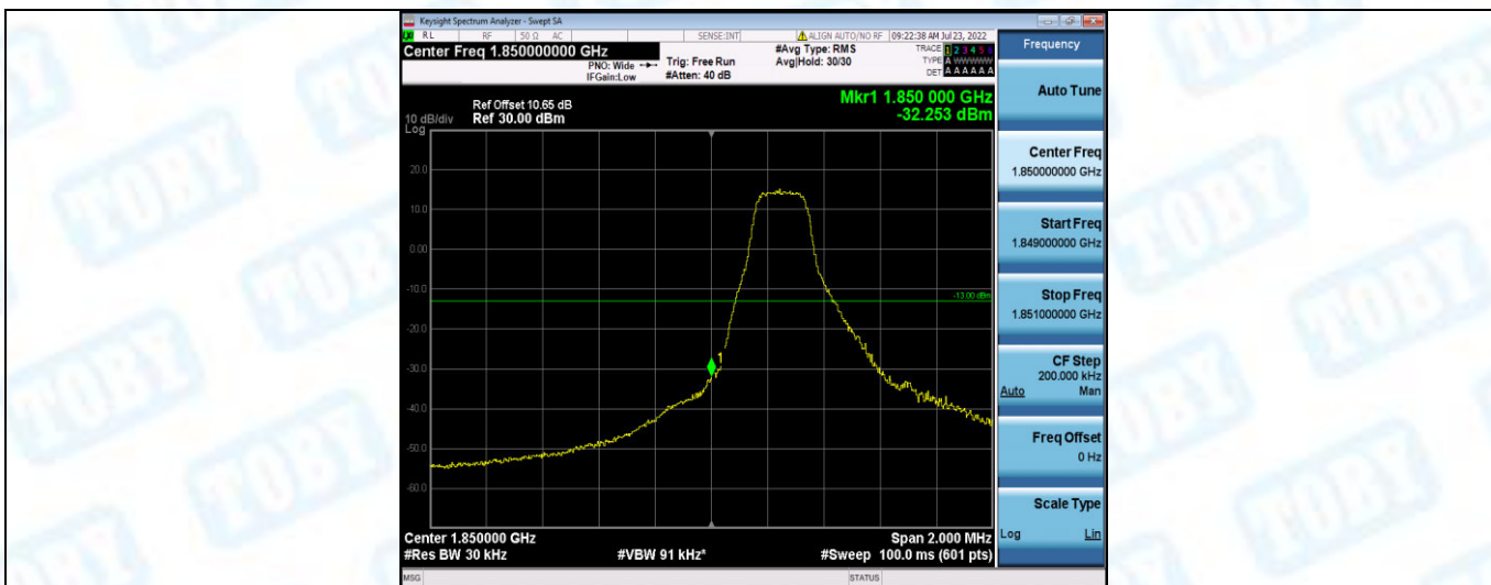
Band25-1.4MHz-QPSK-26047-1RB#5
