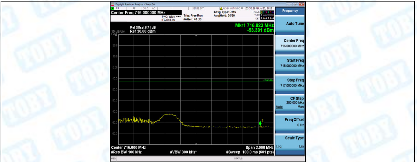
Band17-5MHz-16QAM-23825-1RB#24
