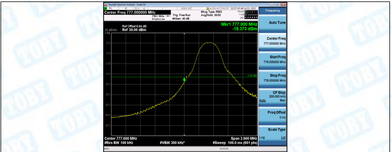
Band13-5MHz-QPSK-23205-1RB#24
