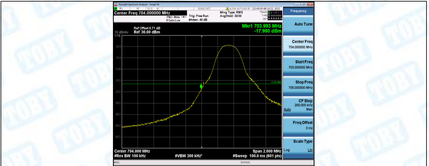
Band17-5MHz-QPSK-23755-1RB#24
