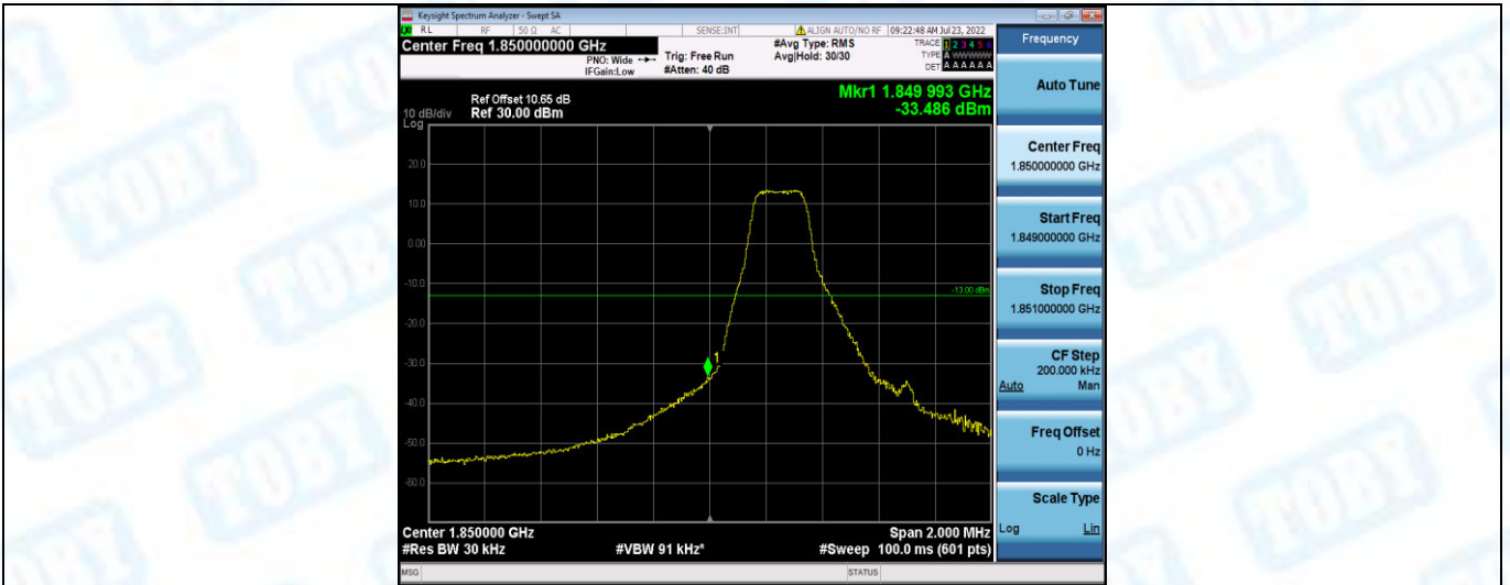
Band25-1.4MHz-16QAM-26047-1RB#5
