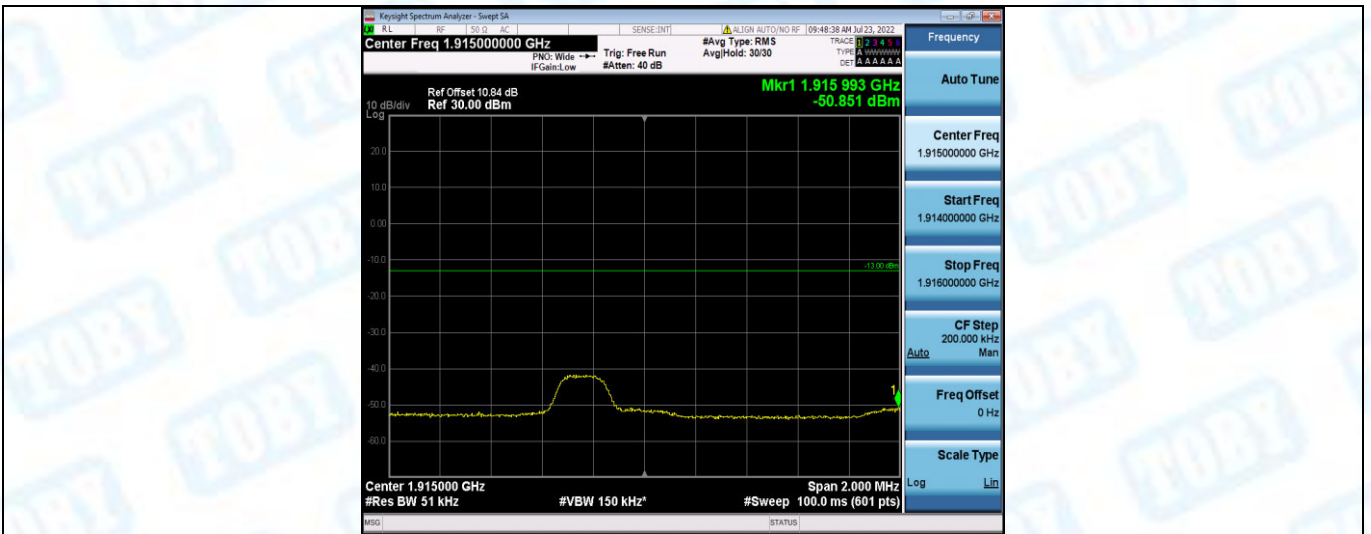
Band25-3MHz-16QAM-26675-1RB#14
