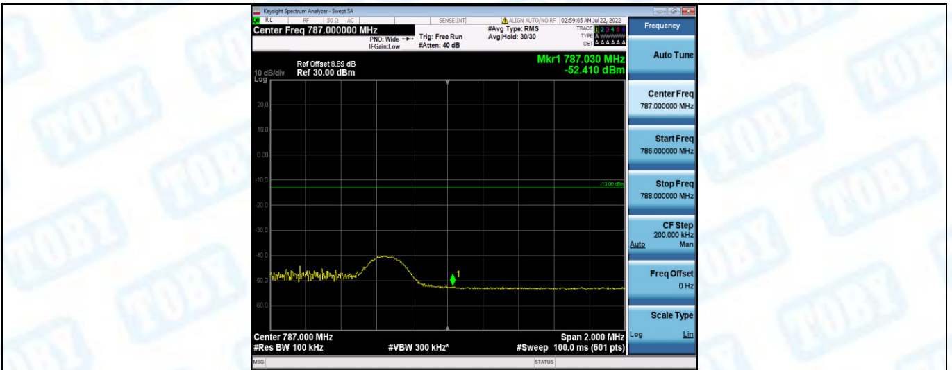
Band13-5MHz-16QAM-23255-1RB#24
