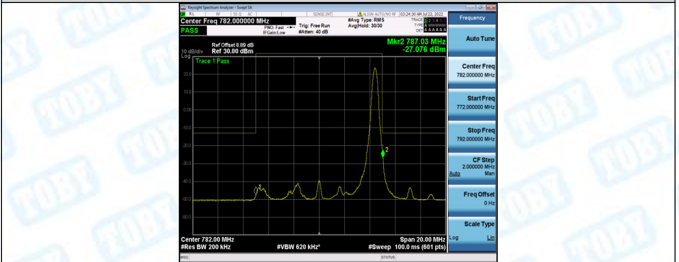
Band13-10MHz-QPSK-23230-50RB#0
