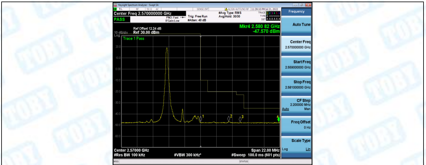
Band7-5MHz-QPSK-21425-1RB#24
