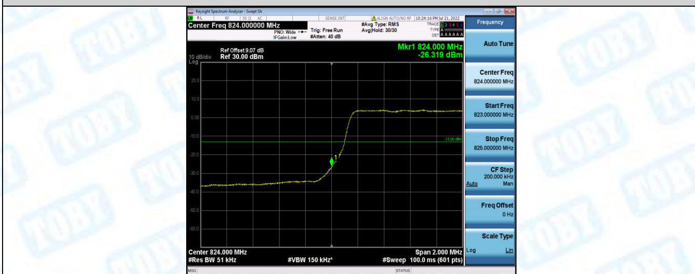
Band5-3MHz-16QAM-20635-1RB#0
