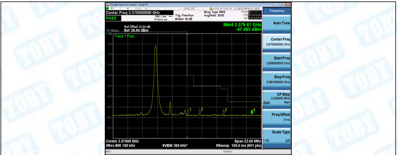
Band7-5MHz-16QAM-21425-1RB#24
