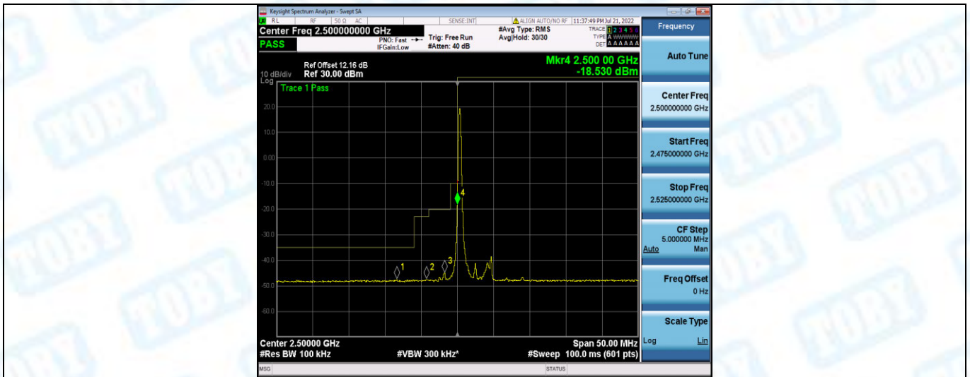
Band7-5MHz-QPSK-20775-1RB#24
