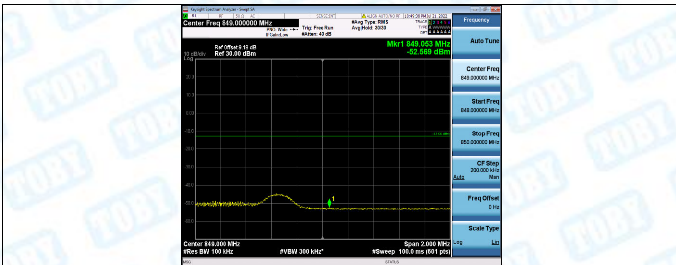
Band5-5MHz-16QAM-20625-1RB#24
