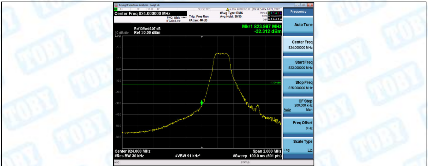
Band5-1.4MHz-16QAM-20407-1RB#5
