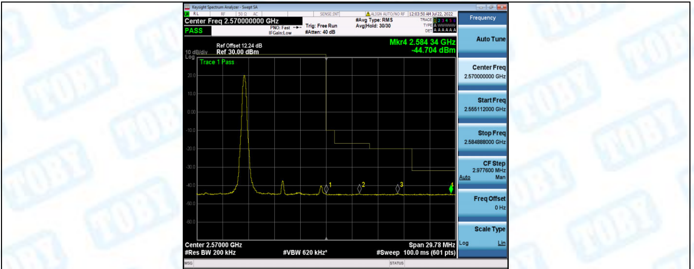
Band7-10MHz-16QAM-21400-1RB#49
