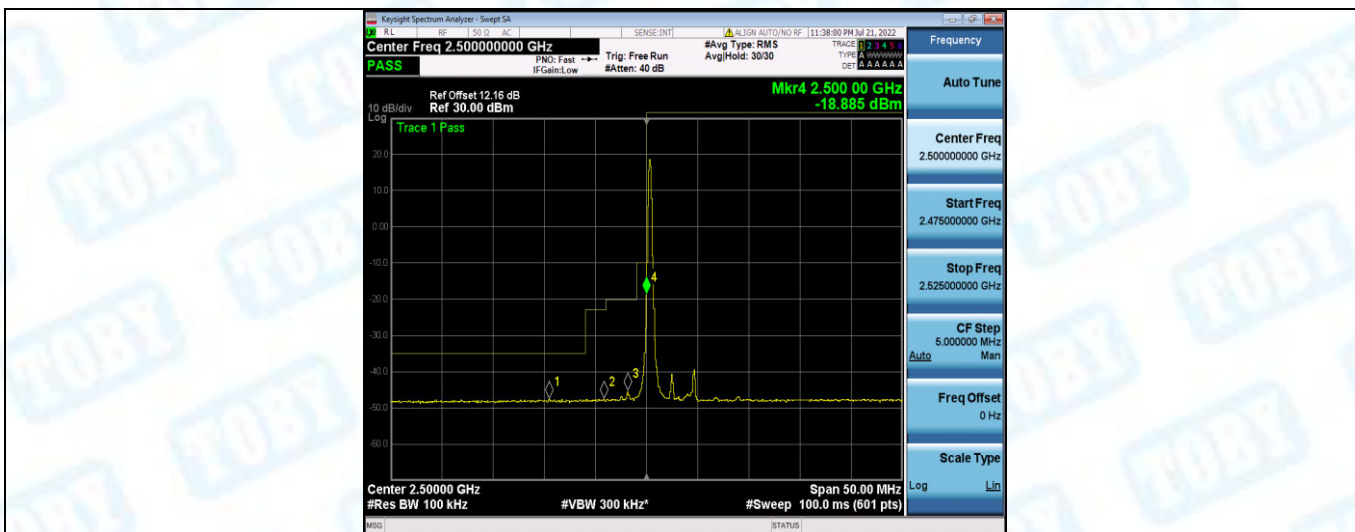
Band7-5MHz-16QAM-20775-1RB#24
