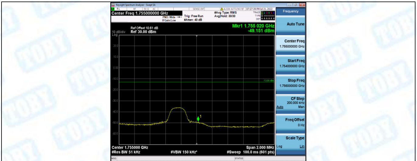
Band4-3MHz-QPSK-20385-1RB#14
