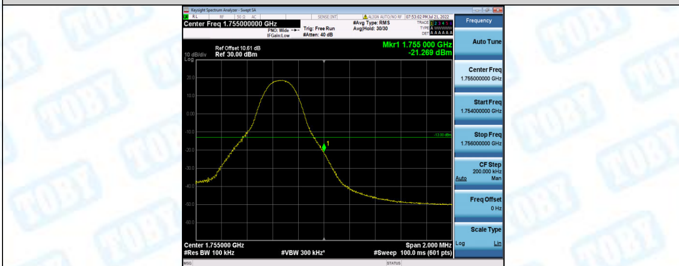
Band4-5MHz-16QAM-20375-25RB#0
