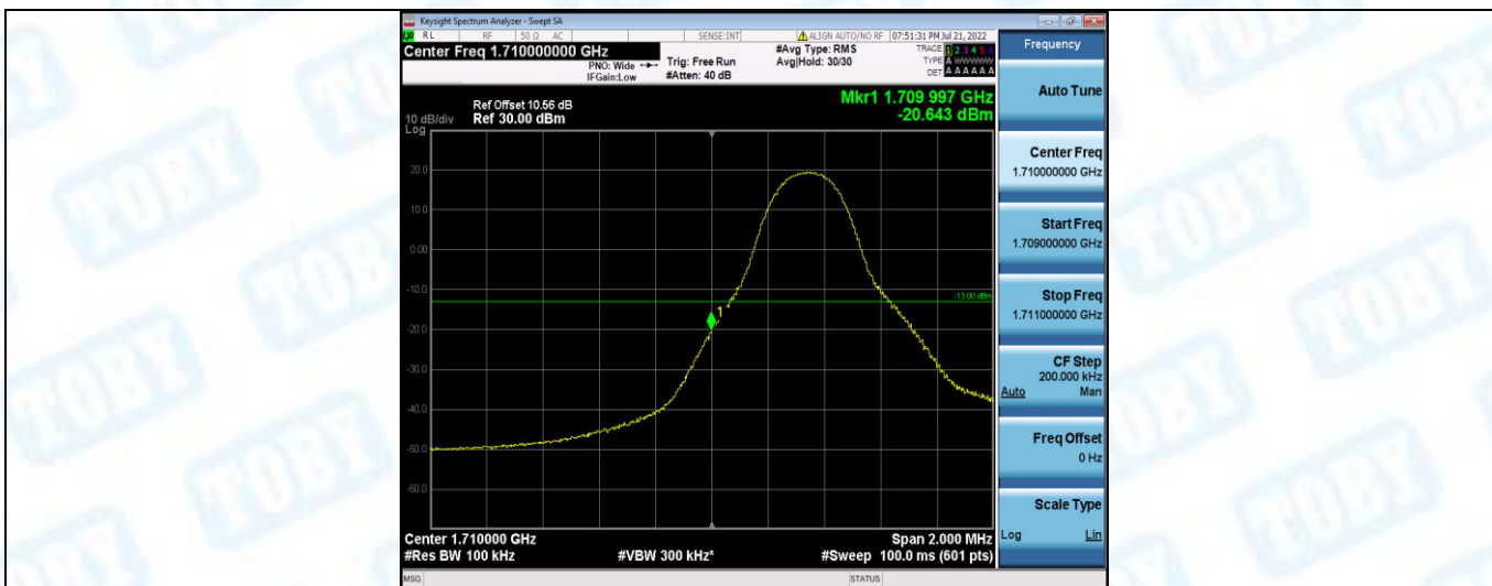
Band4-5MHz-16QAM-19975-1RB#24
