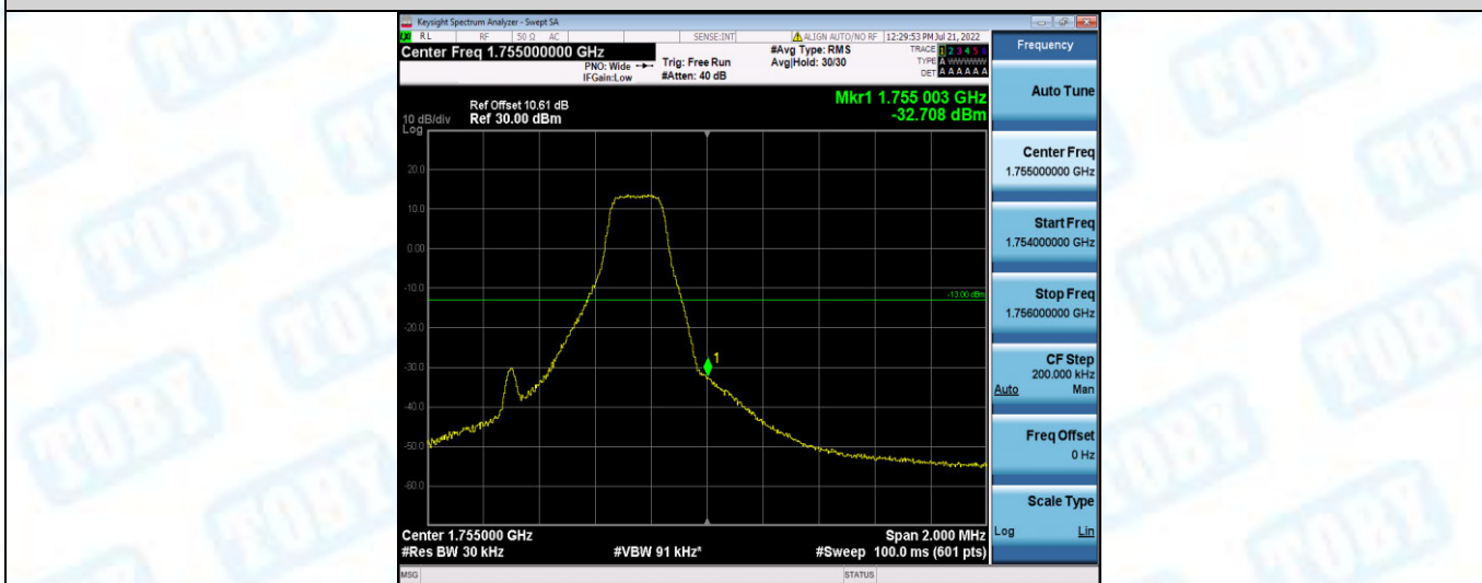
Band4-1.4MHz-16QAM-20393-6RB#0
