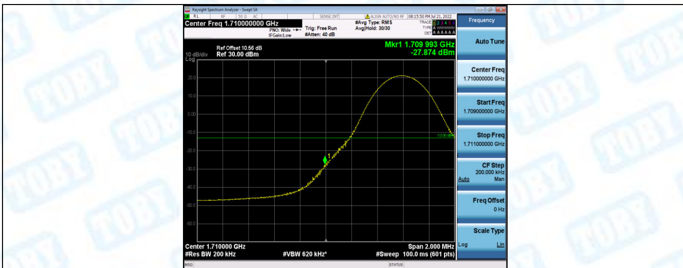
Band4-10MHz-16QAM-20000-1RB#49
