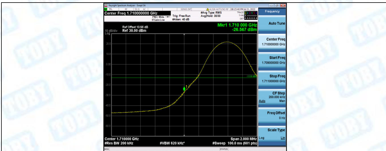
Band4-10MHz-QPSK-20000-1RB#49
