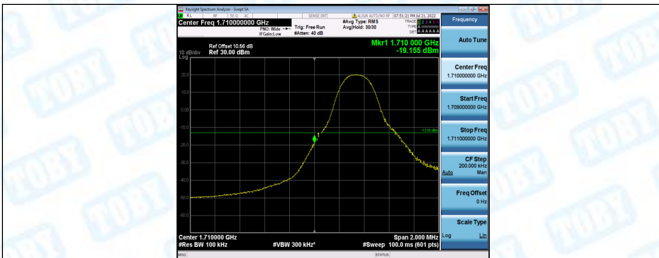
Band4-5MHz-QPSK-19975-1RB#24
