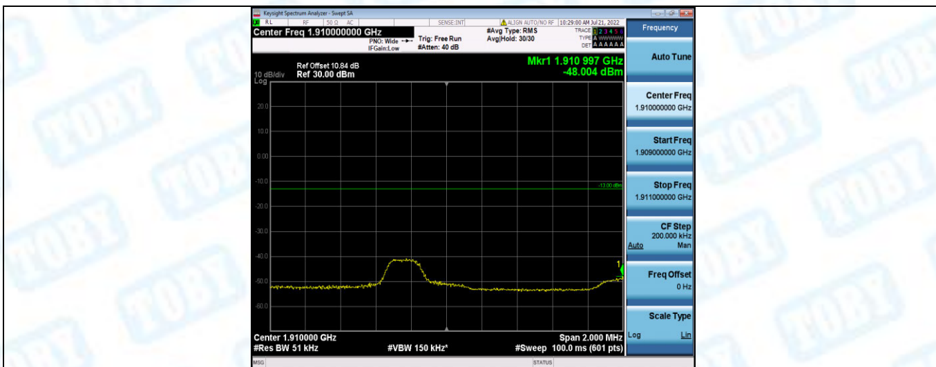
Band2-3MHz-16QAM-19185-1RB#14
