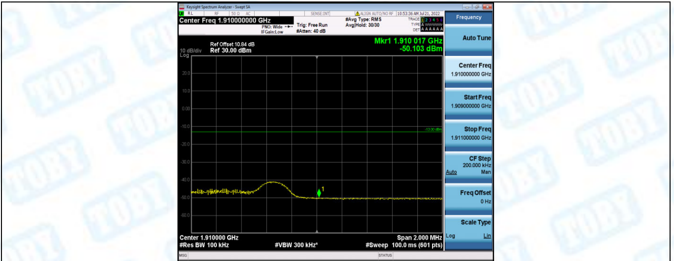
Band2-5MHz-16QAM-19175-1RB#24
