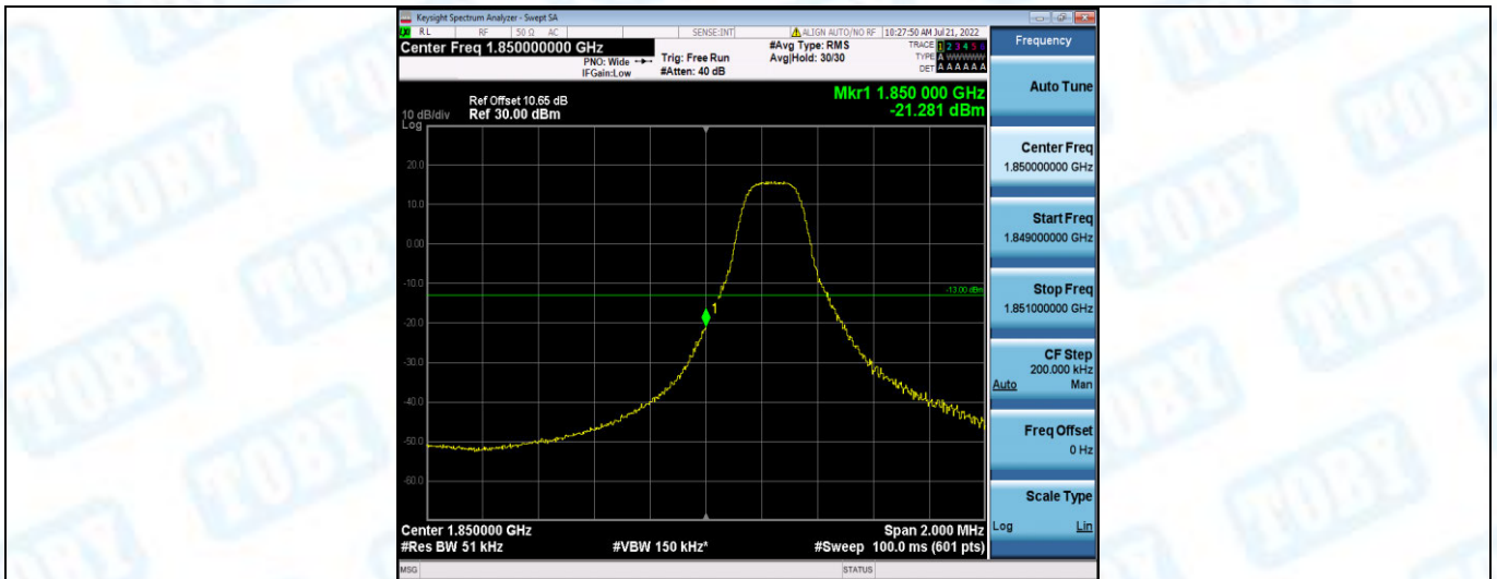
Band2-3MHz-16QAM-18615-1RB#14
