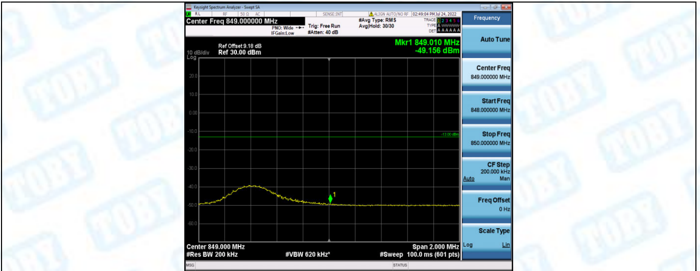
Band26-10MHz-16QAM-26990-1RB#49
