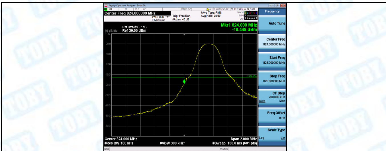
Band26-5MHz-QPSK-26815-1RB#24
