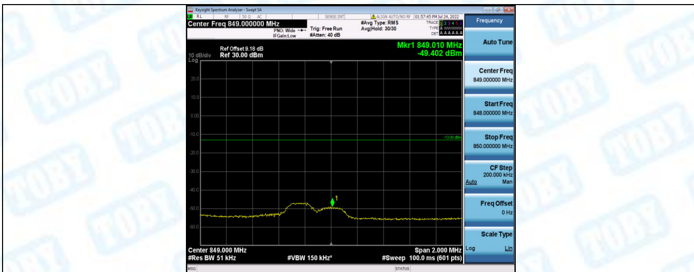
Band26-3MHz-QPSK-27025-1RB#14
