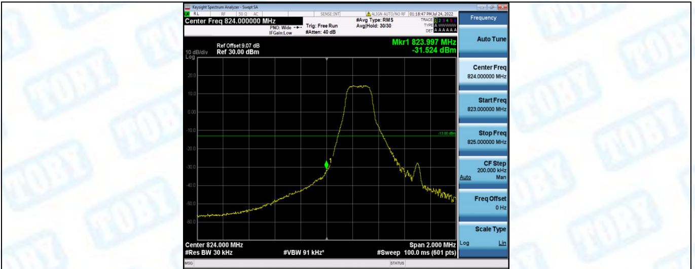
Band26-1.4MHz-16QAM-26797-1RB#5
