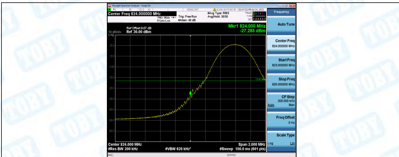
Band26-10MHz-16QAM-26840-1RB#49
