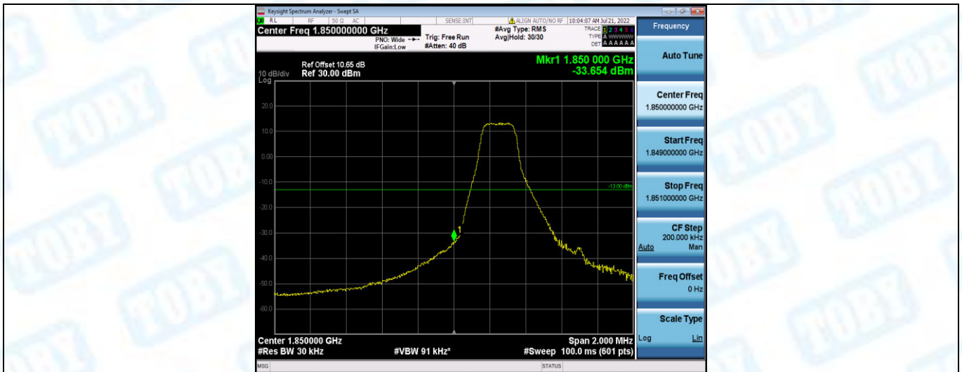
Band2-1.4MHz-16QAM-18607-1RB#5
