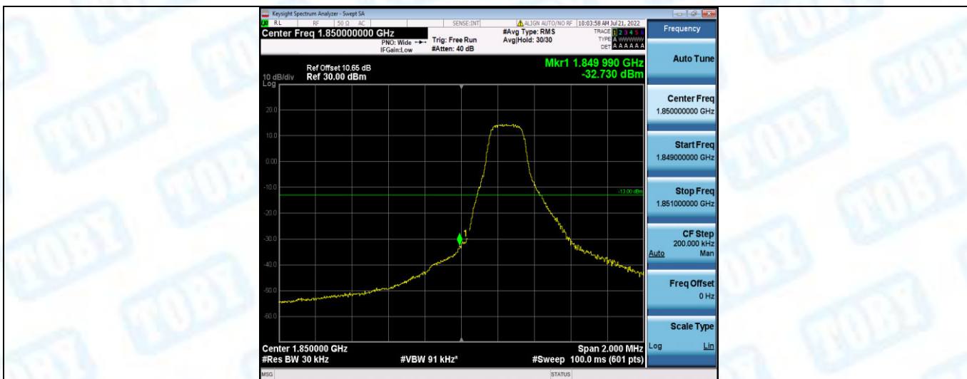
Band2-1.4MHz-QPSK-18607-1RB#5
