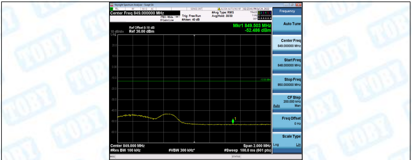
Band26-5MHz-QPSK-27015-1RB#24
