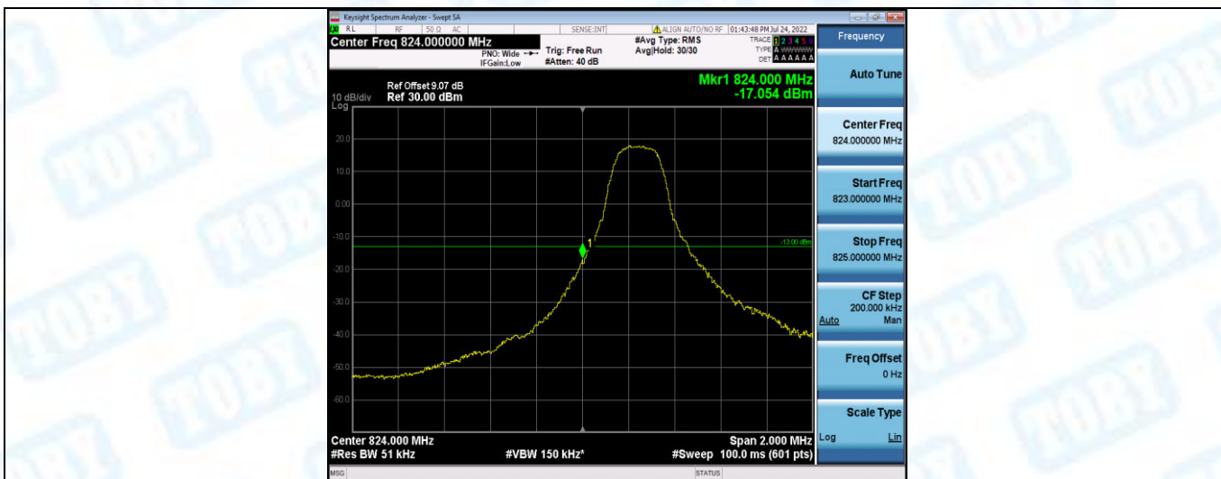
Band26-3MHz-QPSK-26805-1RB#14
