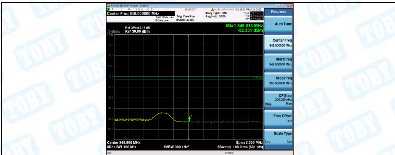
Band26-5MHz-16QAM-27015-1RB#24
