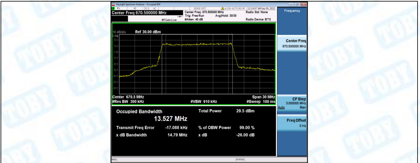
Band71-15MHz-16QAM-133297-75RB#0
