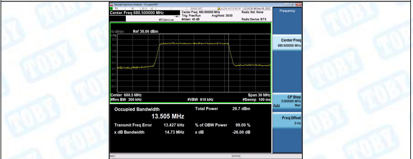
Band71-15MHz-16QAM-133397-75RB#0
