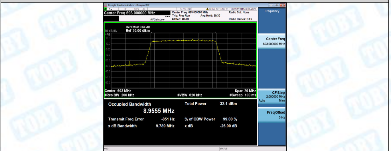
Band71-10MHz-16QAM-133172-50RB#0
