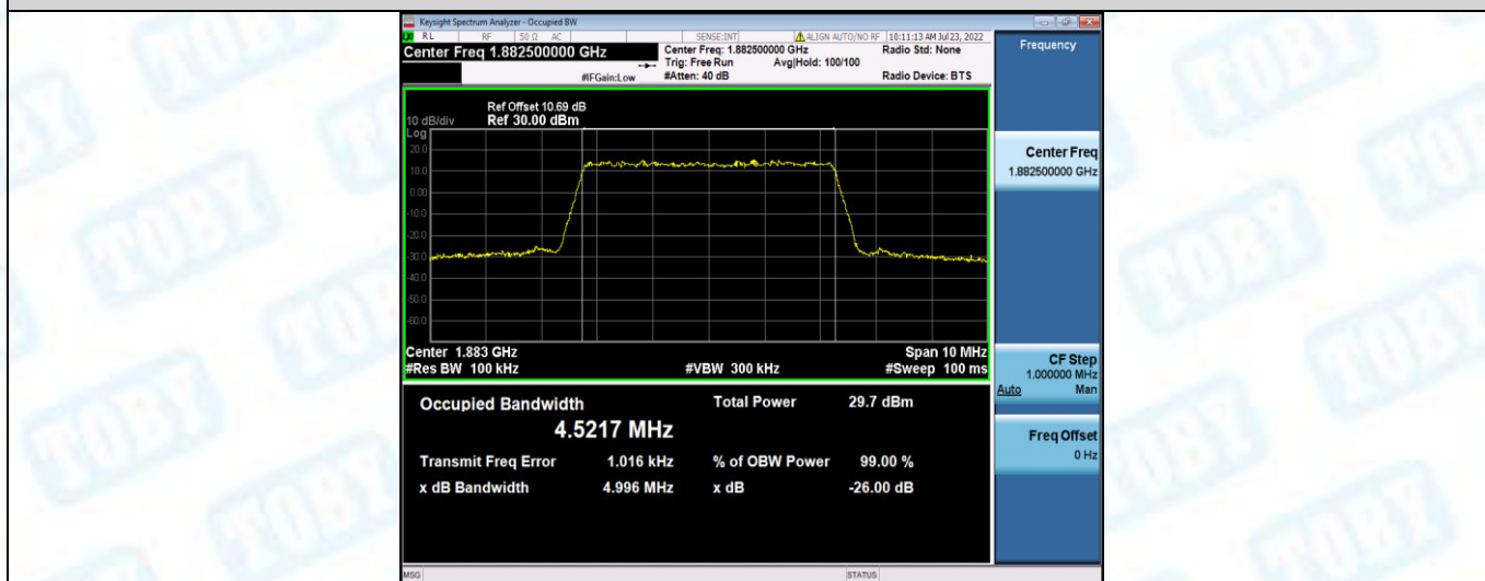
Band25-5MHz-QPSK-26665-25RB#0
