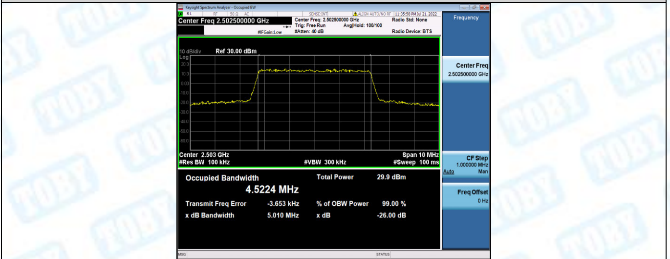
Band7-5MHz-QPSK-21100-25RB#0
