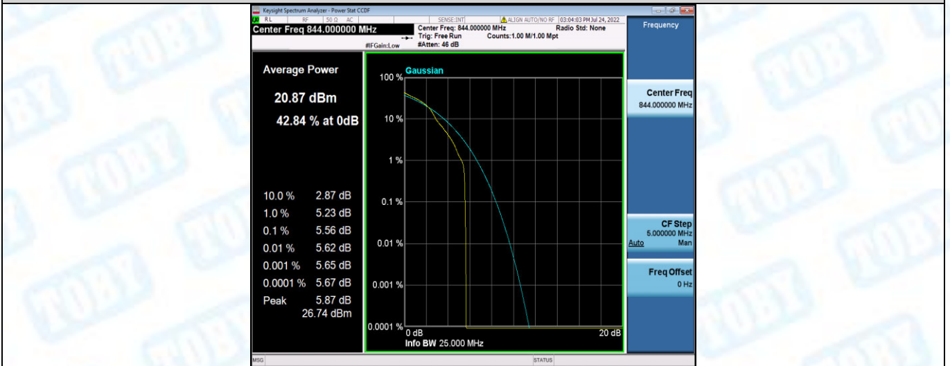
Band26-10MHz-16QAM-26990-50RB#0
