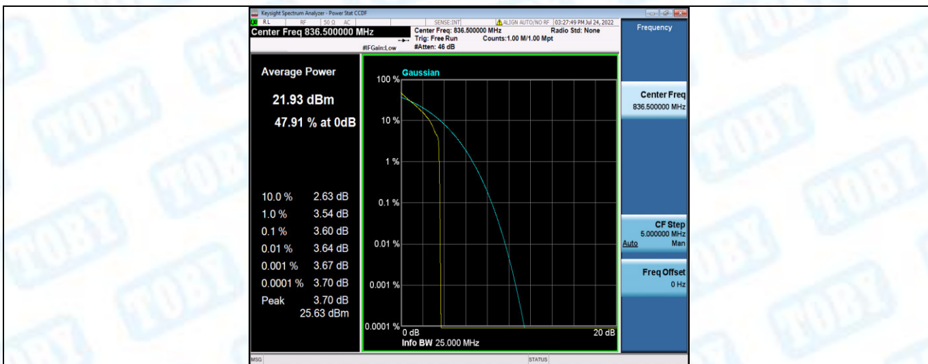
Band26-15MHz-QPSK-26915-75RB#0
