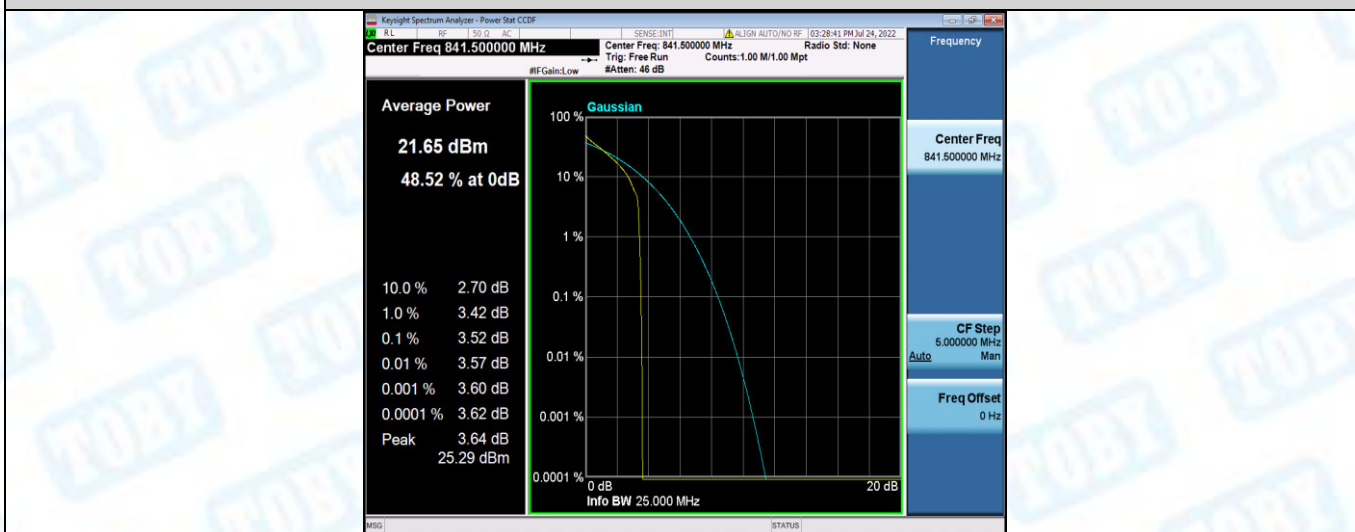
Band26-15MHz-QPSK-26965-75RB#0
