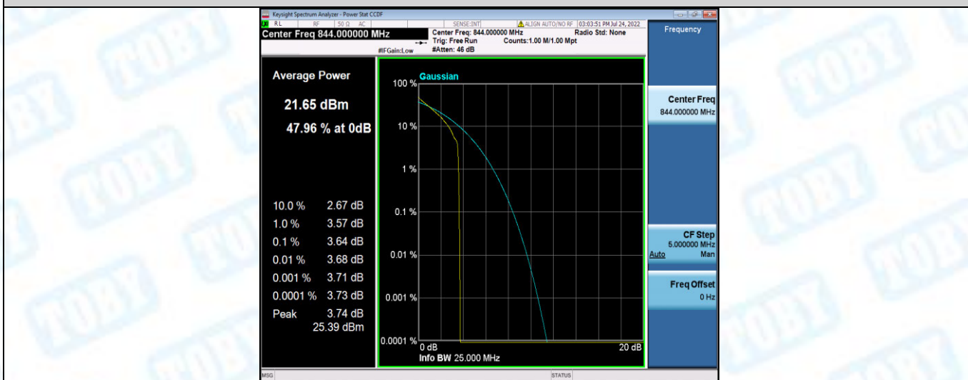
Band26-10MHz-QPSK-26990-50RB#0
