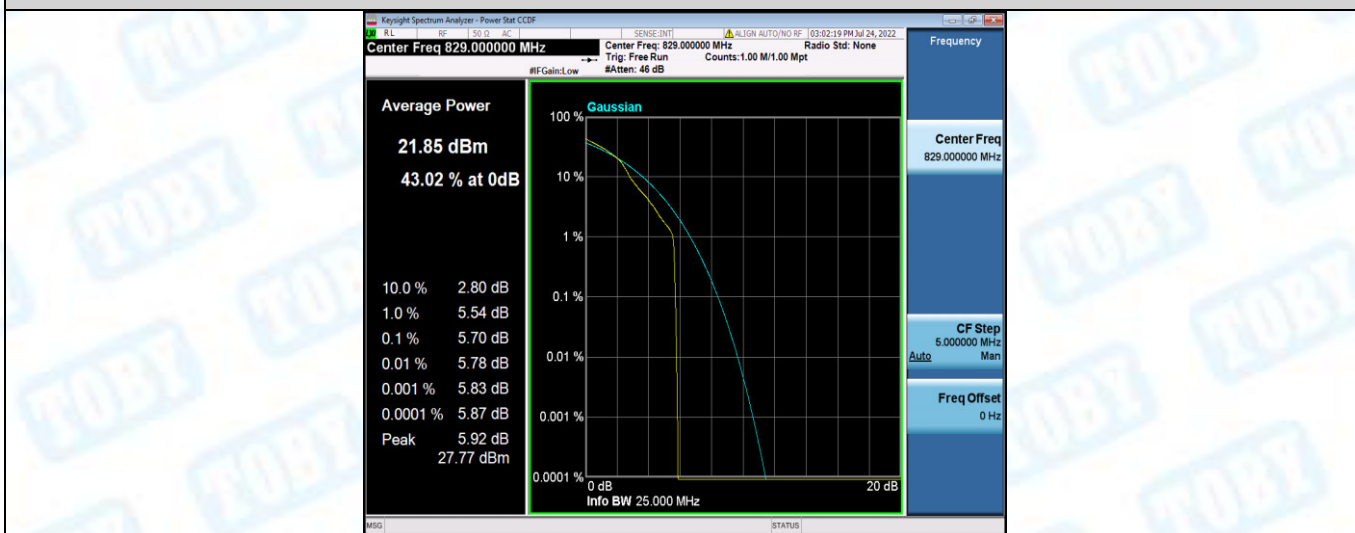
Band26-10MHz-16QAM-26840-50RB#0
