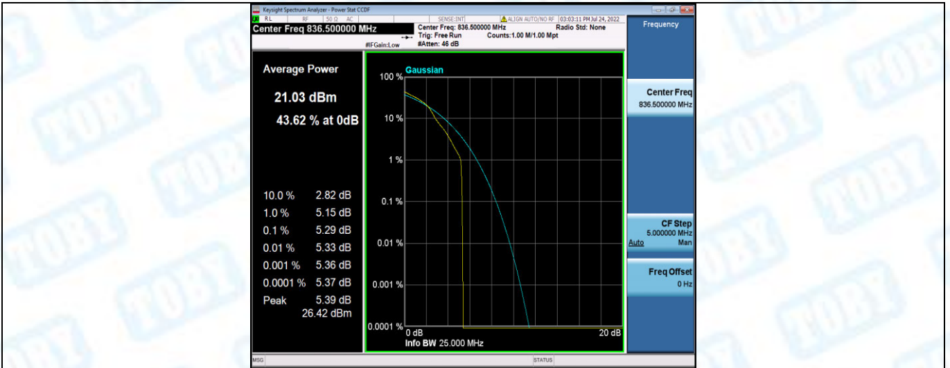
Band26-10MHz-16QAM-26915-50RB#0
