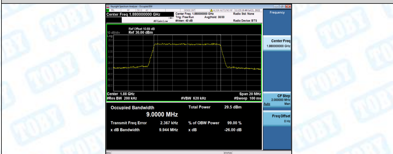
Band2-10MHz-QPSK-19150-50RB#0
