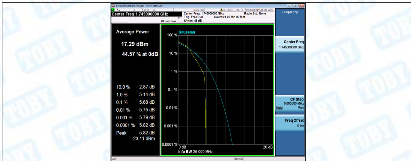
Band66-3MHz-16QAM-132322-15RB#0
