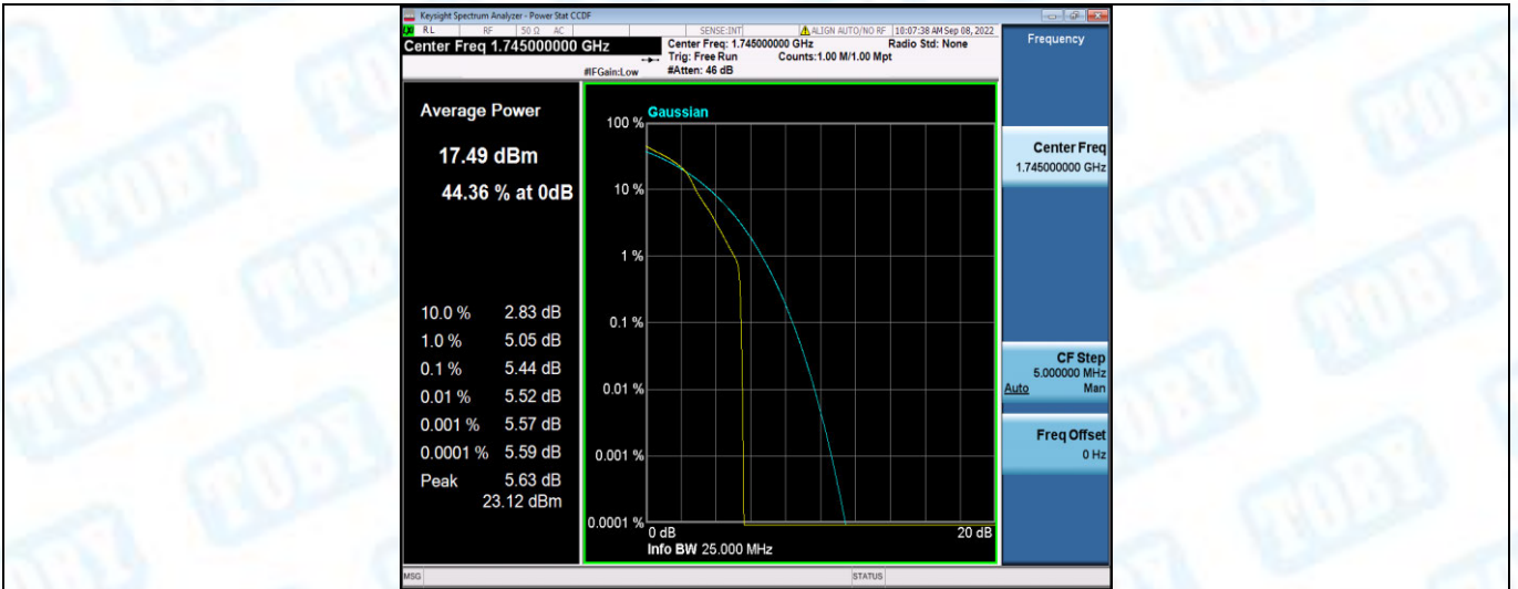
Band66-10MHz-16QAM-132322-50RB#0
