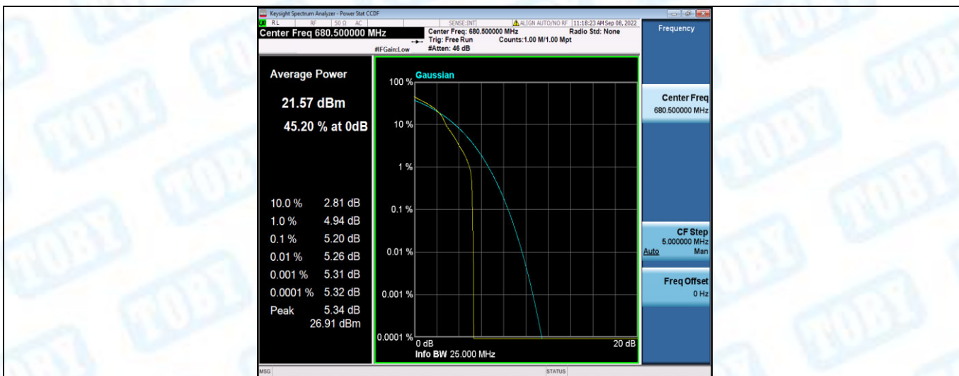
Band71-5MHz-16QAM-133297-25RB#0
