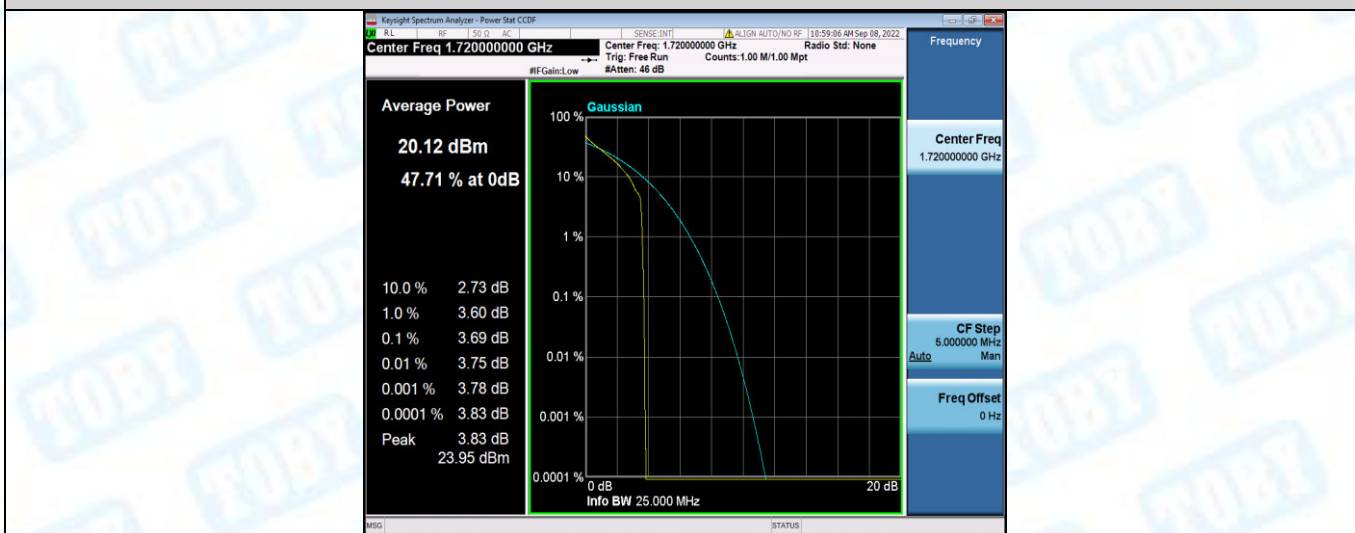
Band66-20MHz-QPSK-132072-100RB#0
