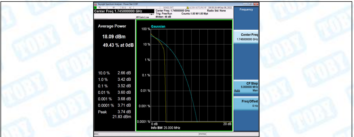
Band66-5MHz-QPSK-132322-25RB#0
