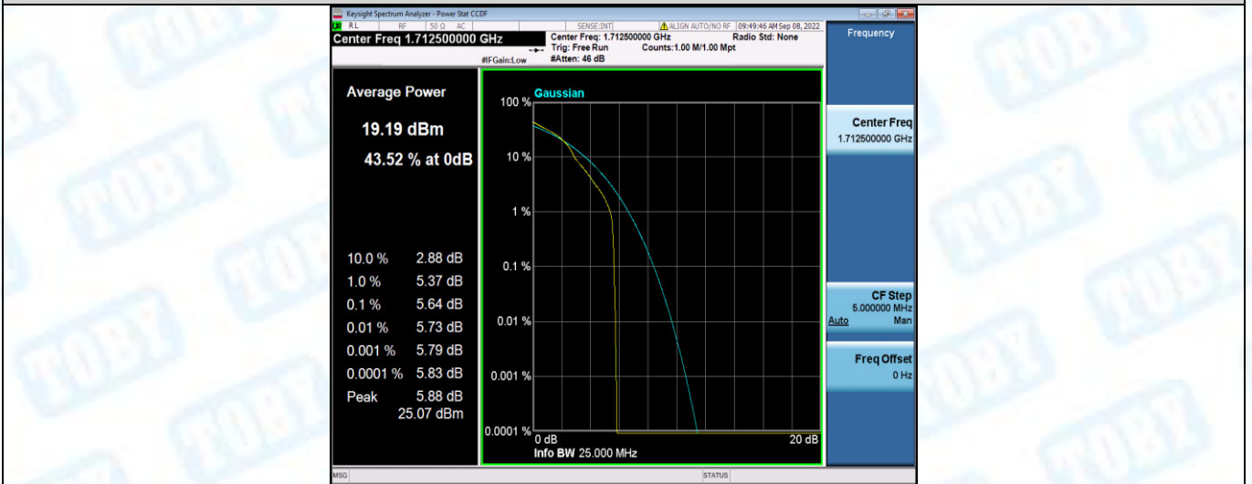
Band66-5MHz-16QAM-131997-25RB#0
