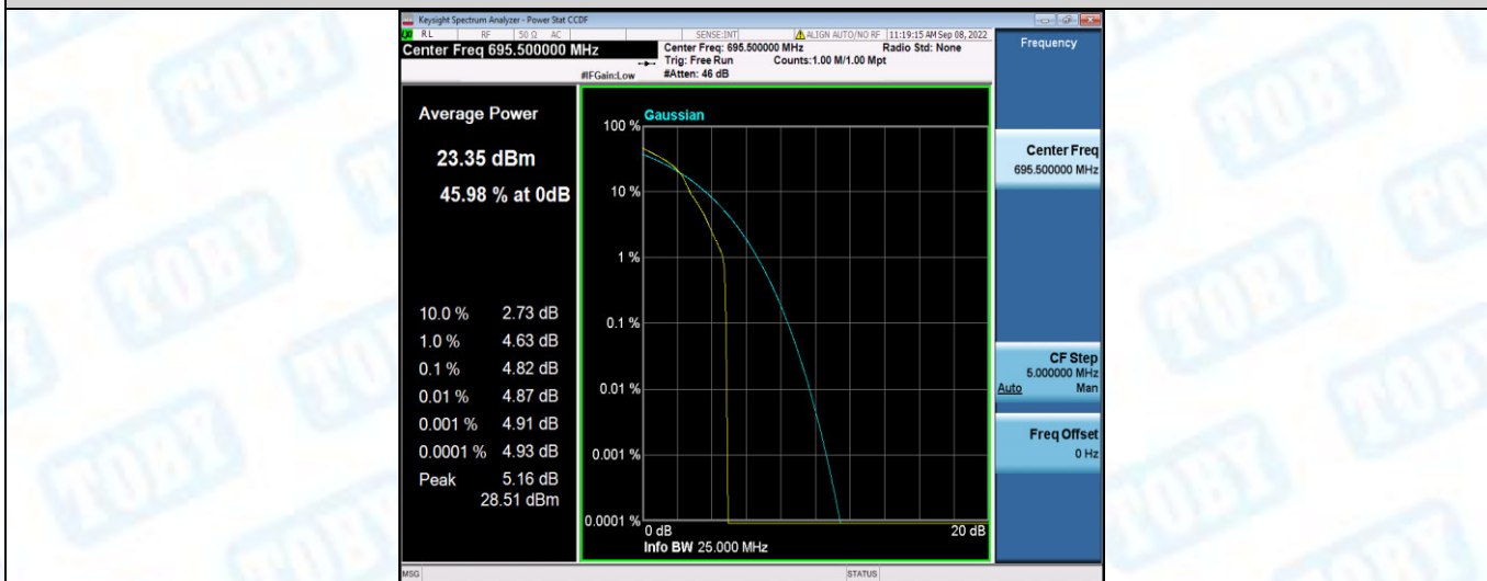
Band71-5MHz-16QAM-133447-25RB#0
