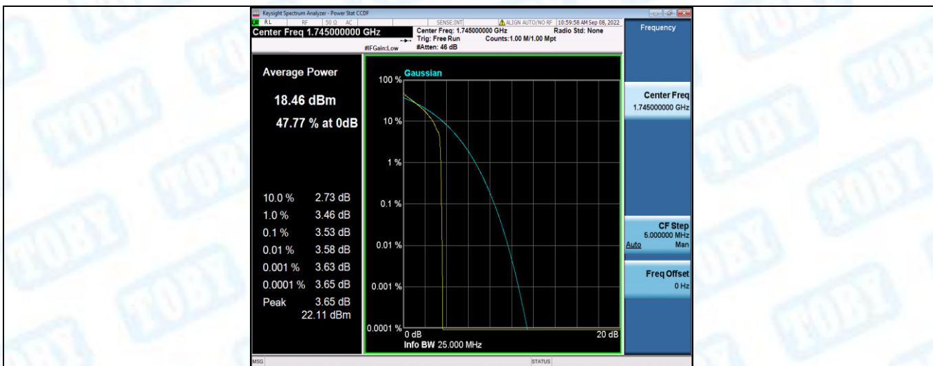
Band66-20MHz-QPSK-132322-100RB#0
