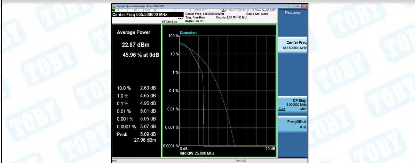
Band71-5MHz-16QAM-133147-25RB#0
