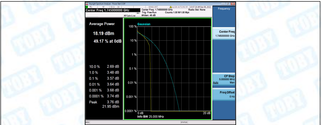
Band66-10MHz-QPSK-132322-50RB#0
