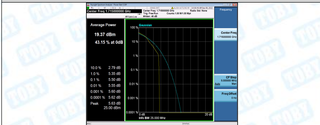
Band66-10MHz-16QAM-132022-50RB#0
