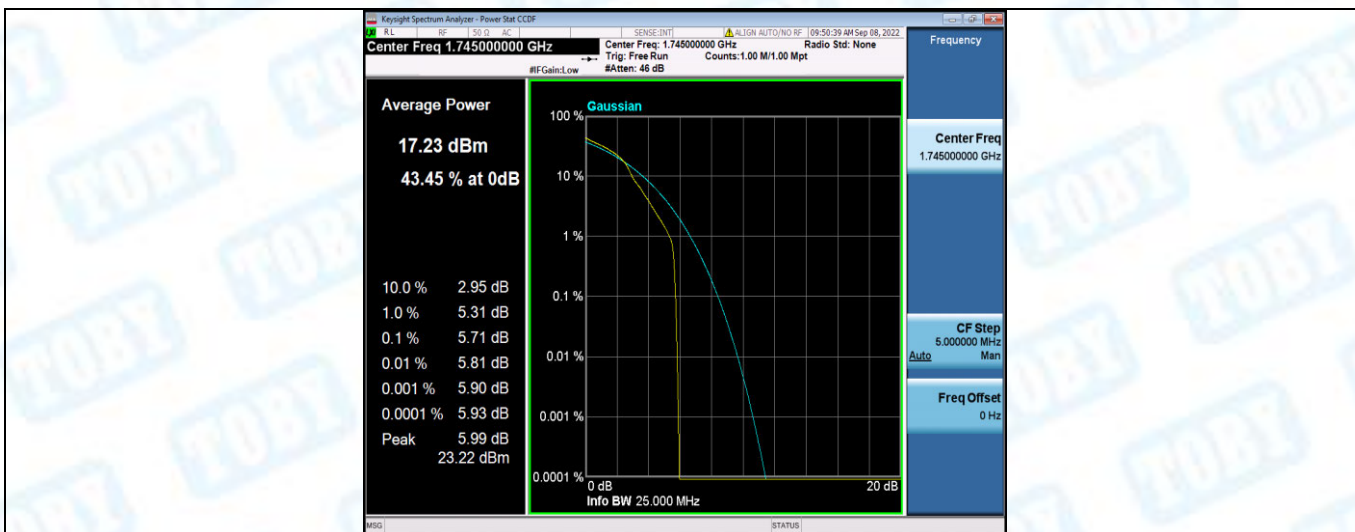
Band66-5MHz-16QAM-132322-25RB#0
