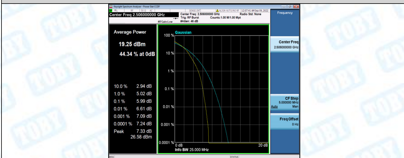
Band41-20MHz-16QAM-40620-1RB#0
