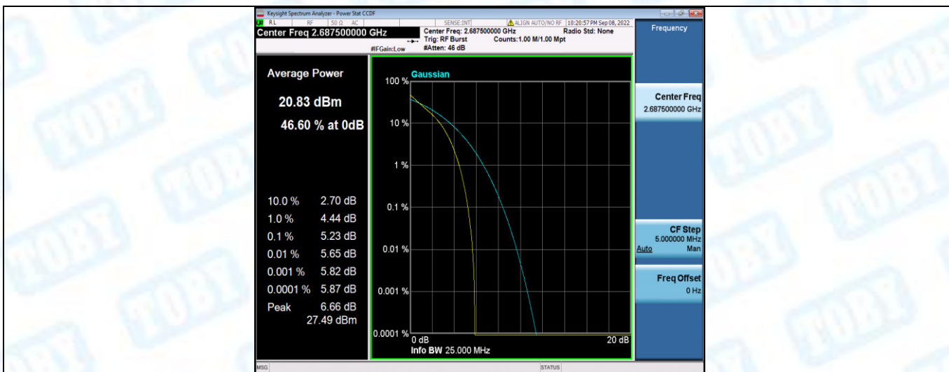
Band41-5MHz-16QAM-39675-1RB#0
