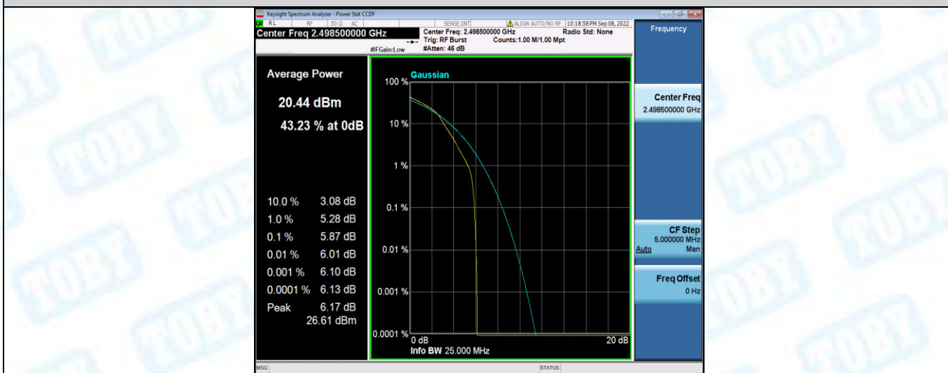
Band41-5MHz-16QAM-39675-25RB#0
