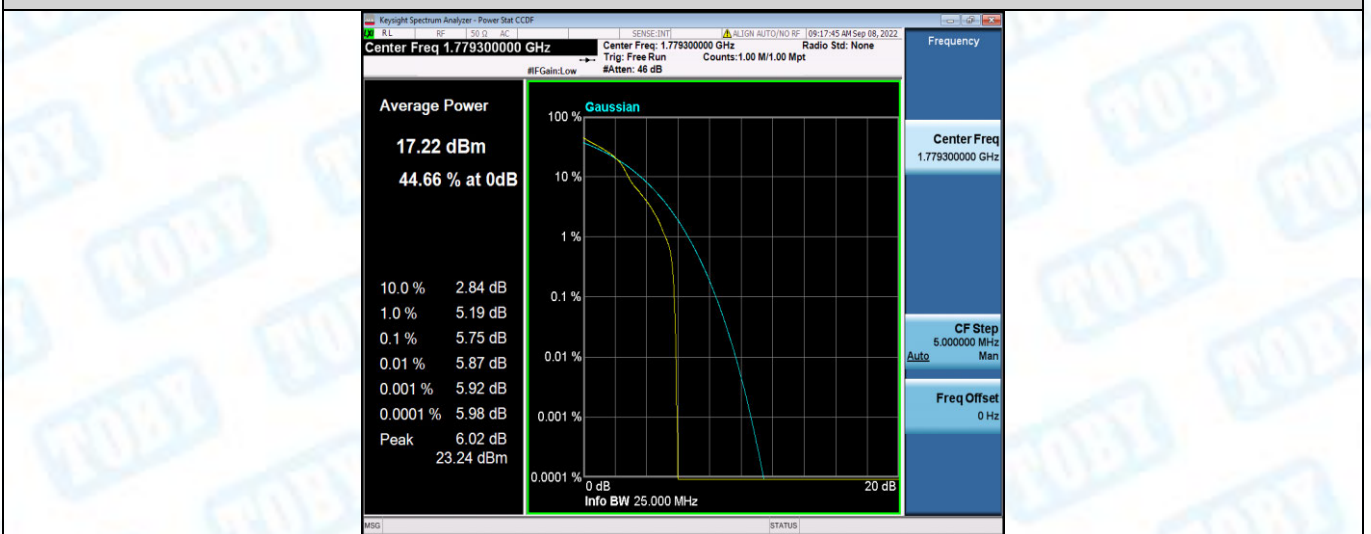
Band66-1.4MHz-16QAM-132665-6RB#0
