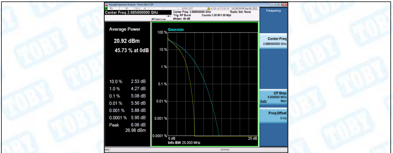
Band41-10MHz-16QAM-39700-1RB#0
