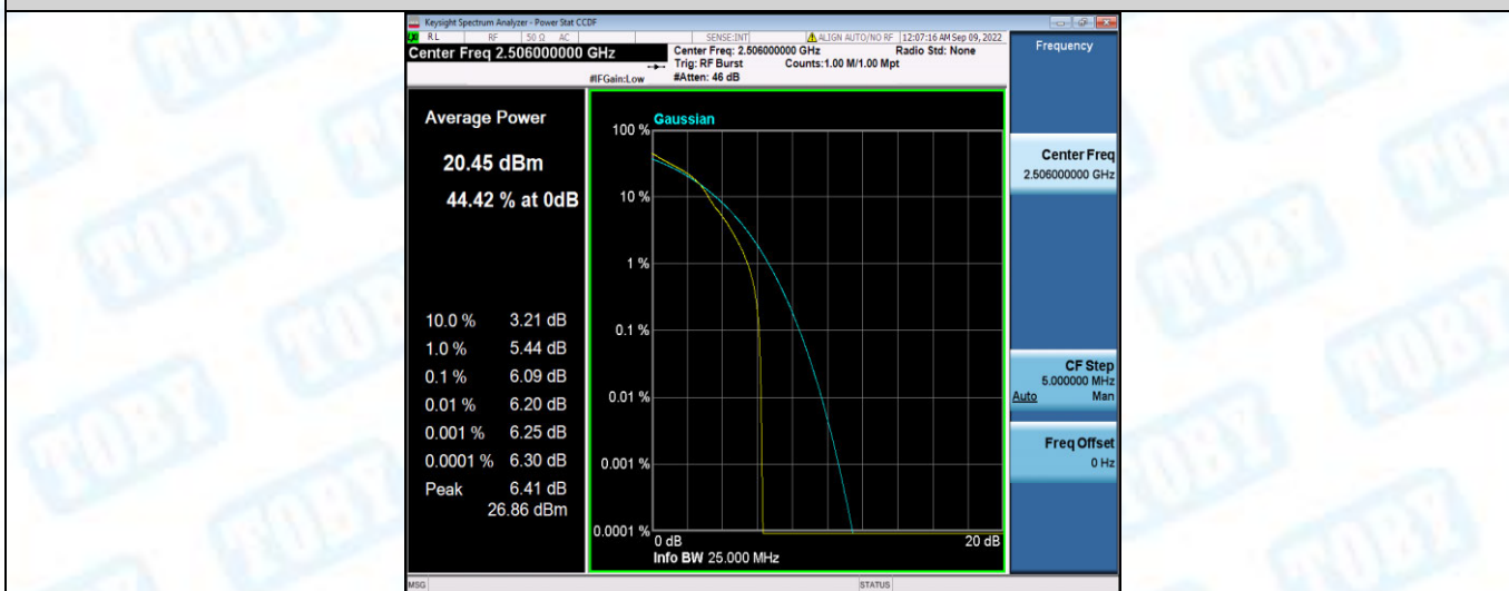
Band41-20MHz-16QAM-39750-100RB#0
