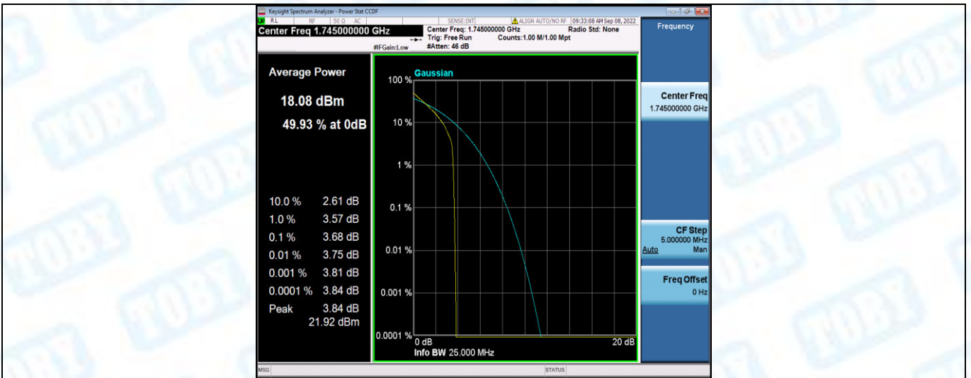
Band66-3MHz-QPSK-132322-15RB#0
