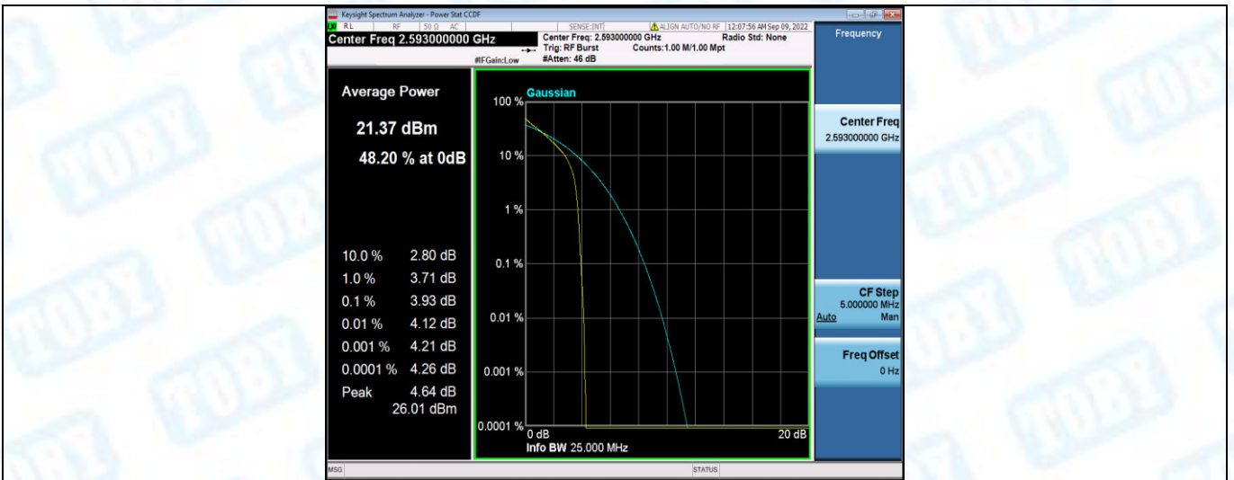
Band41-20MHz-QPSK-40620-100RB#0
