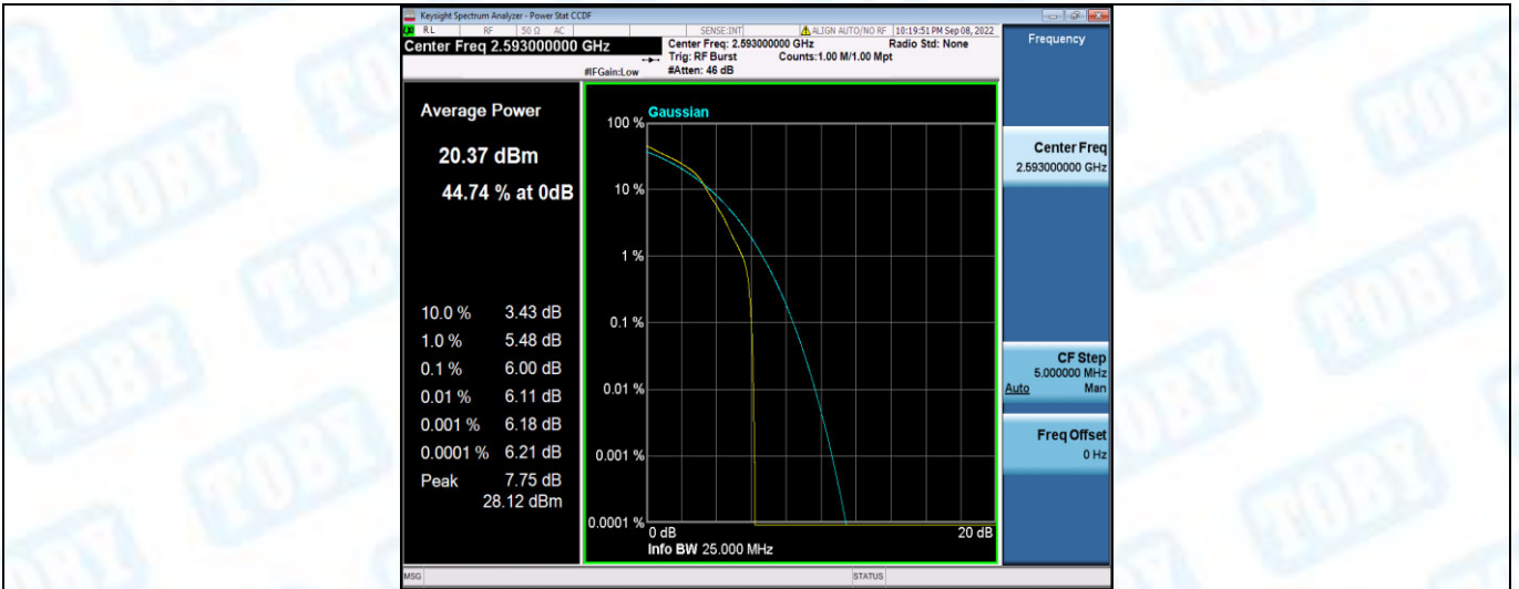
Band41-5MHz-16QAM-40620-25RB#0
