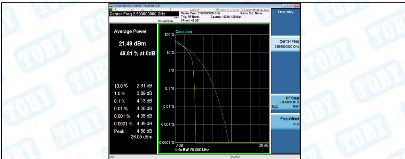
Band41-5MHz-QPSK-40620-25RB#0
