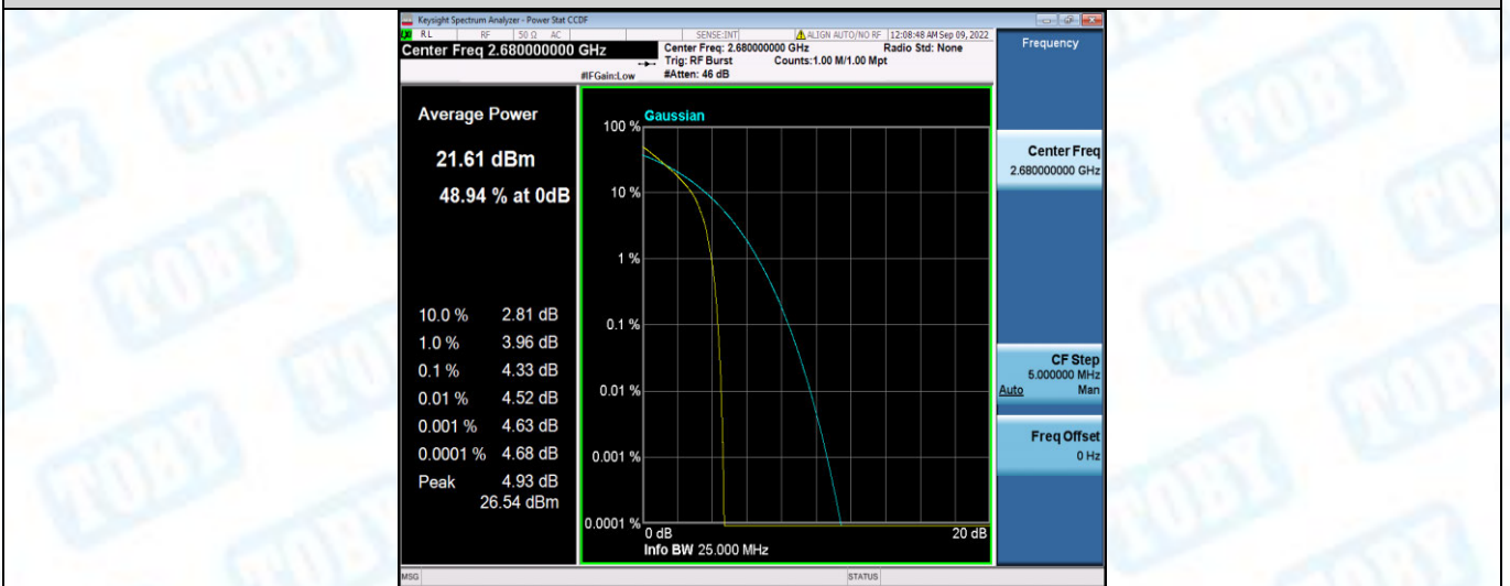
Band41-20MHz-QPSK-41490-100RB#0
