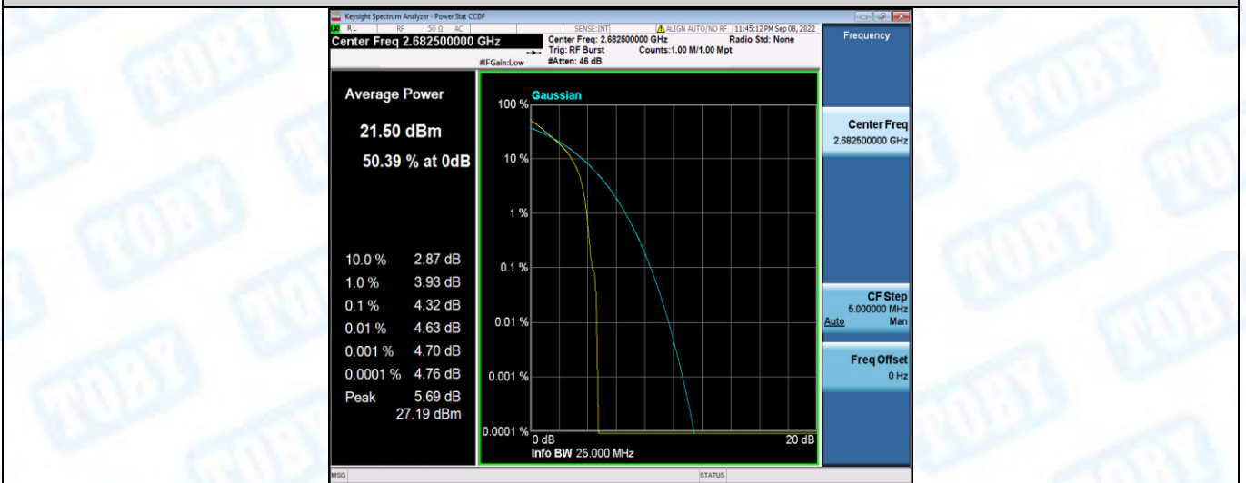
Band41-15MHz-QPSK-41515-75RB#0
