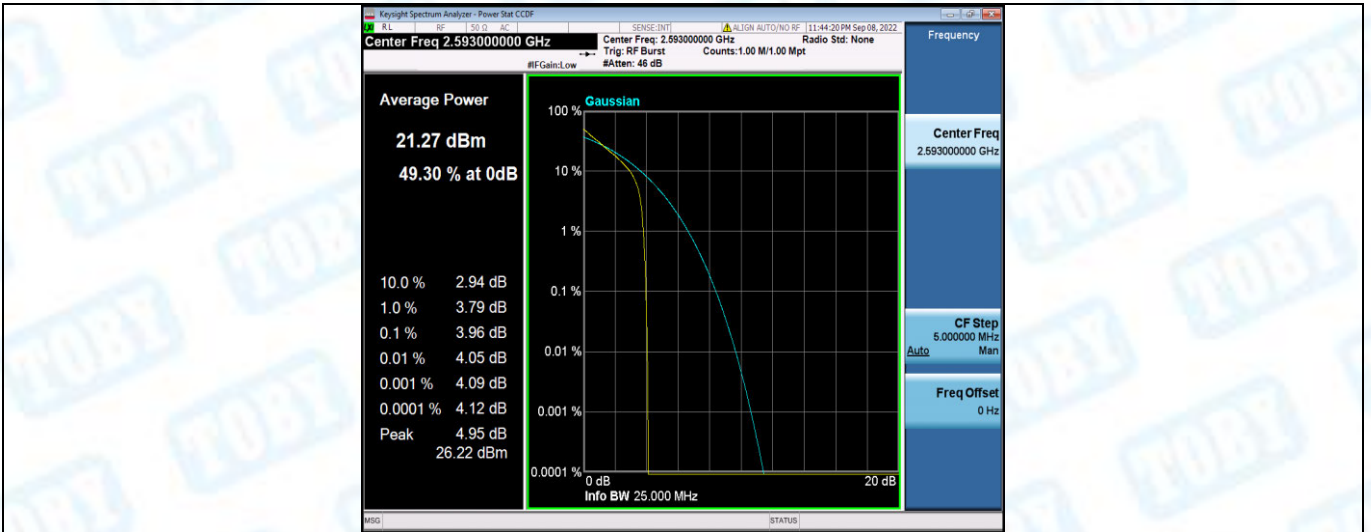
Band41-15MHz-QPSK-40620-75RB#0
