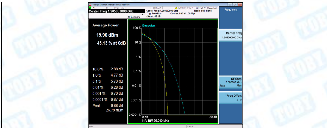
Band41-5MHz-QPSK-39675-1RB#0
