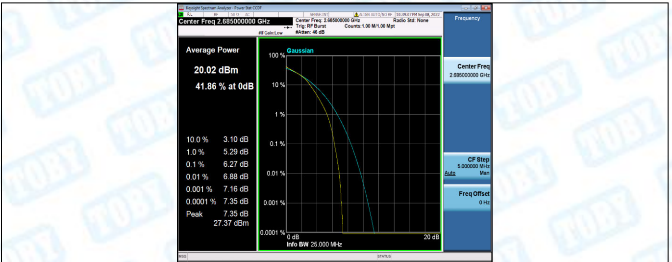
Band41-15MHz-QPSK-39725-1RB#0
