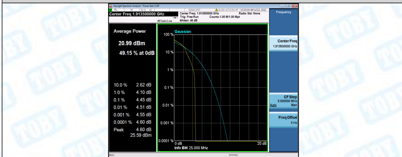
Band25-3MHz-16QAM-26675-15RB#0
