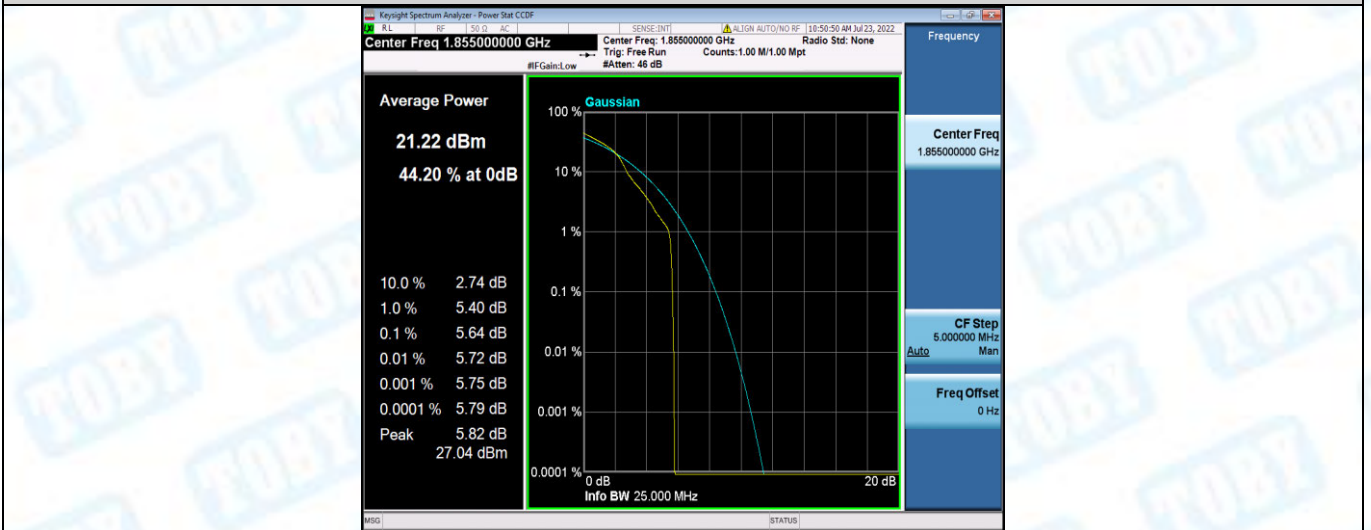
Band25-10MHz-16QAM-26090-50RB#0
