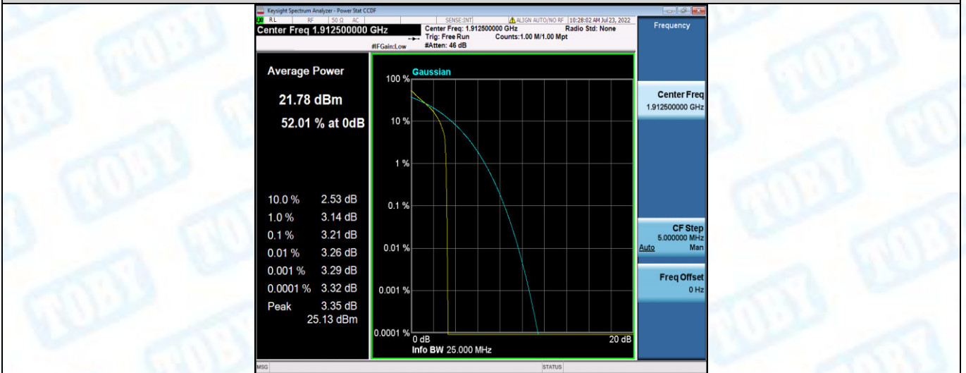
Band25-5MHz-QPSK-26665-25RB#0
