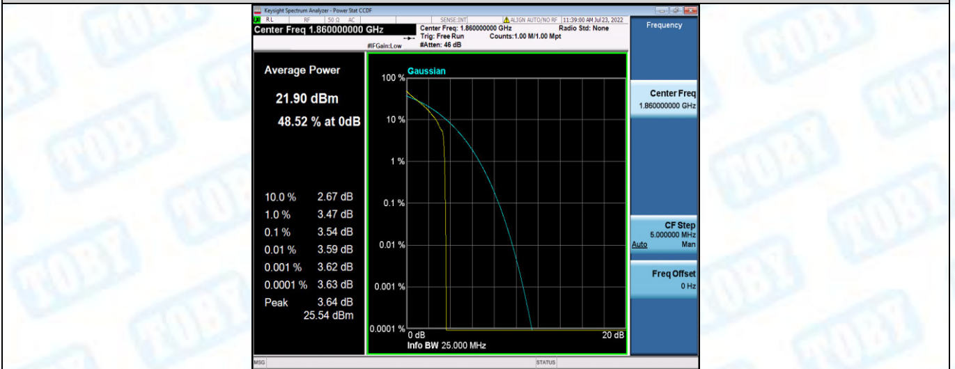
Band25-20MHz-QPSK-26140-100RB#0
