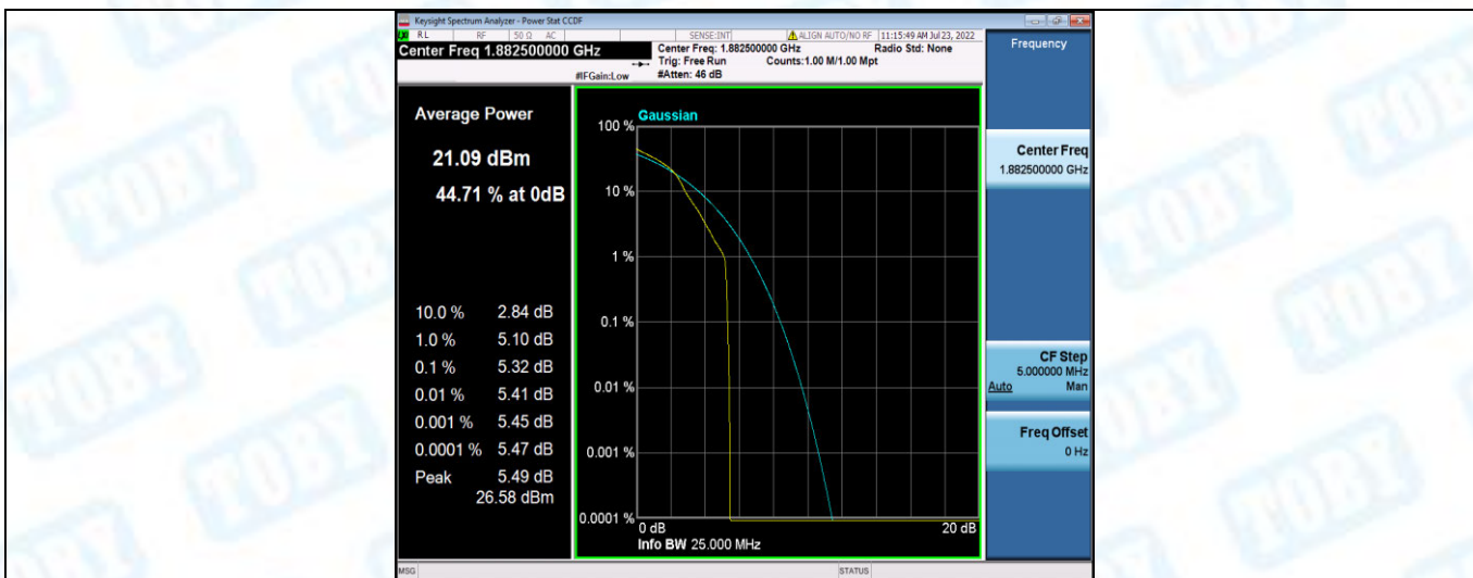
Band25-15MHz-16QAM-26365-75RB#0
