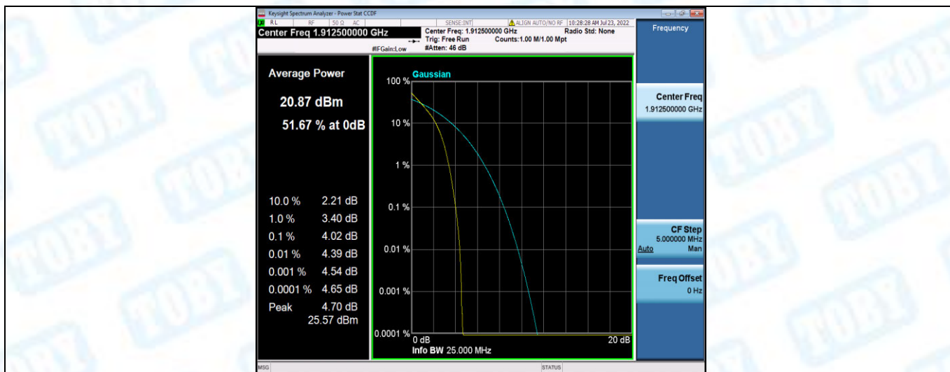
Band25-5MHz-16QAM-26065-1RB#0
