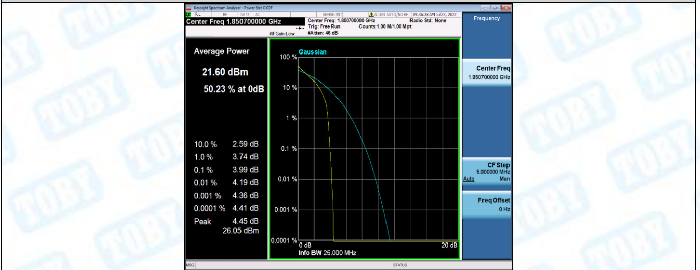
Band25-1.4MHz-QPSK-26047-6RB#0
