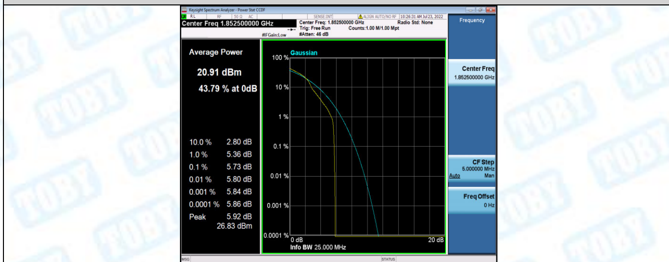
Band25-5MHz-16QAM-26065-25RB#0
