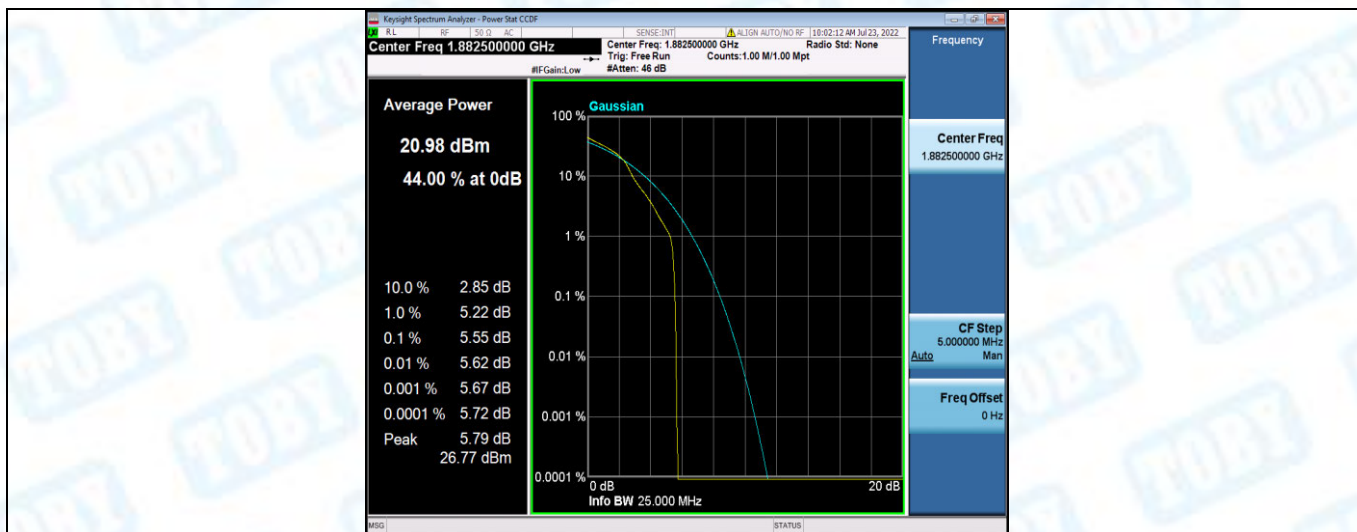
Band25-3MHz-16QAM-26365-15RB#0
