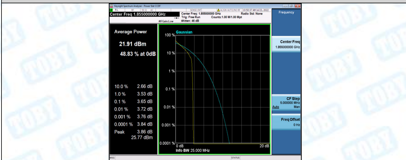
Band25-10MHz-QPSK-26090-50RB#0
