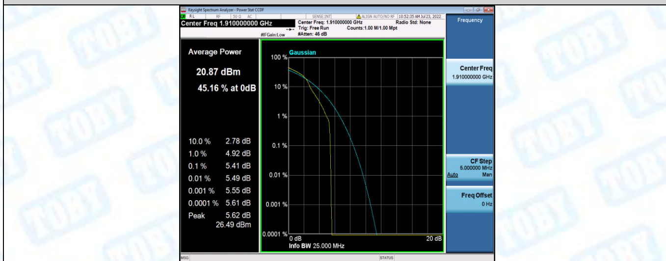
Band25-10MHz-16QAM-26640-50RB#0
