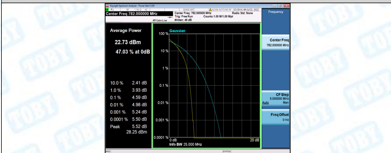
Band13-10MHz-16QAM-23230-1RB#0
