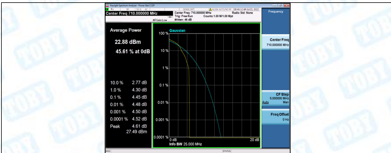
Band17-5MHz-16QAM-23790-25RB#0
