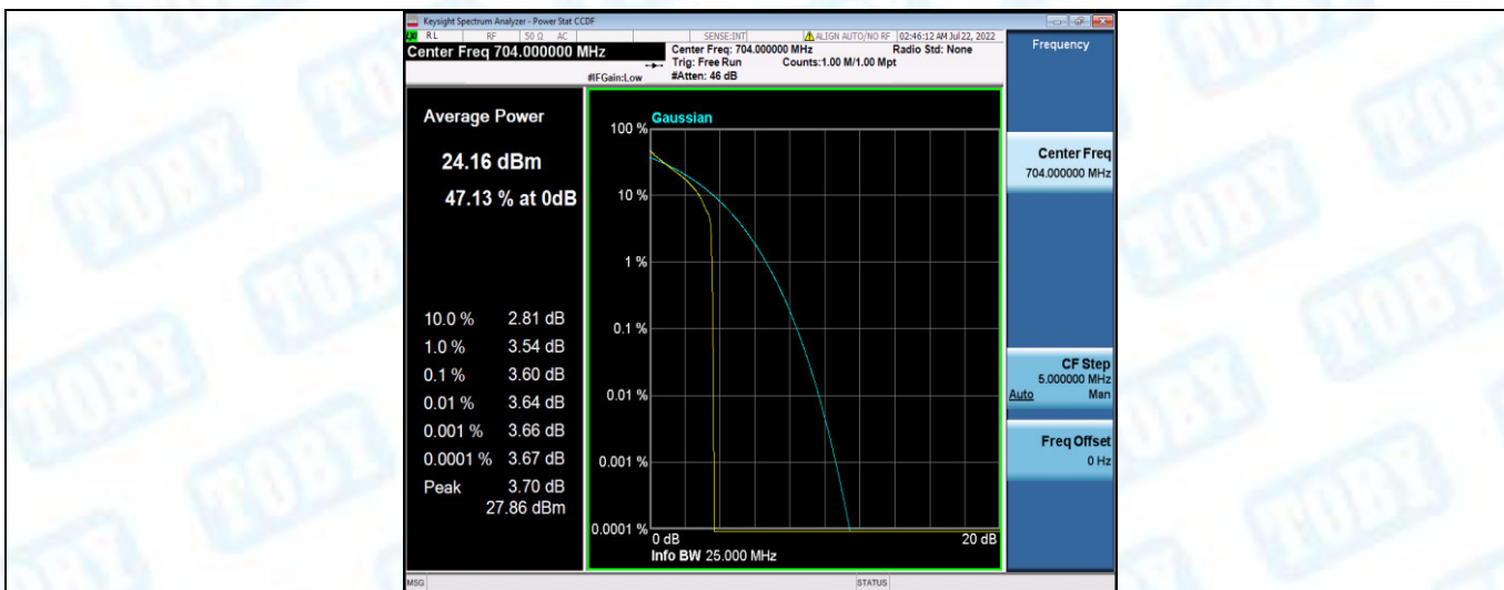
Band12-10MHz-QPSK-23060-50RB#0
