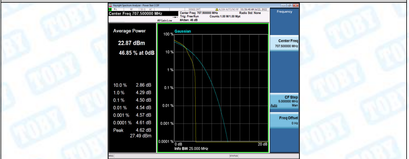
Band12-3MHz-16QAM-23095-15RB#0
