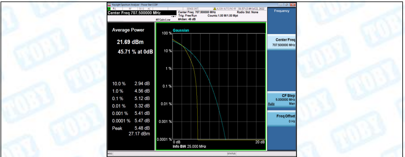
Band12-3MHz-16QAM-23165-1RB#0
