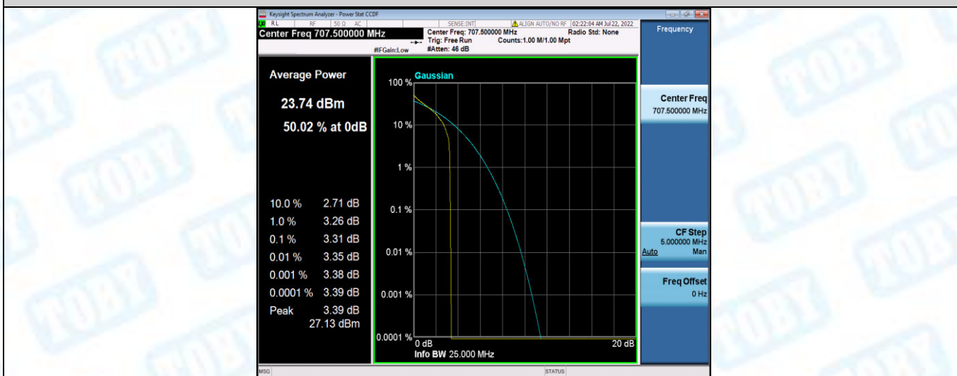
Band12-5MHz-QPSK-23095-25RB#0
