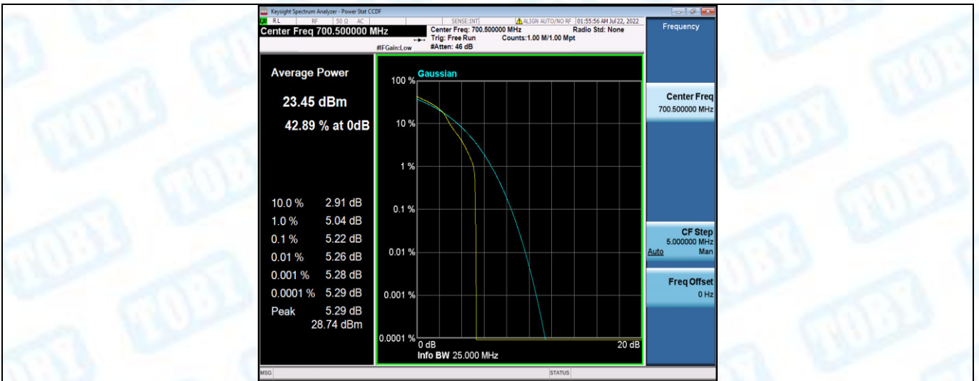
Band12-3MHz-16QAM-23025-15RB#0
