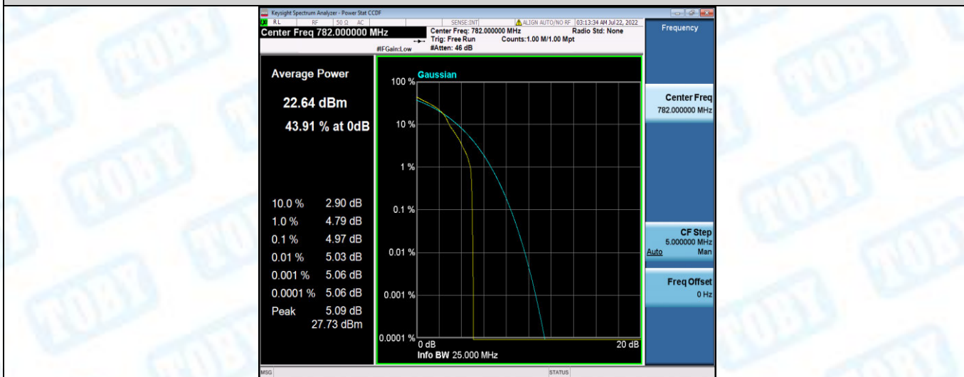
Band13-5MHz-16QAM-23230-25RB#0
