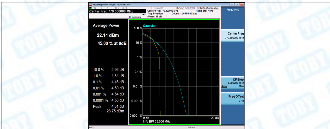
Band13-5MHz-16QAM-23205-25RB#0
