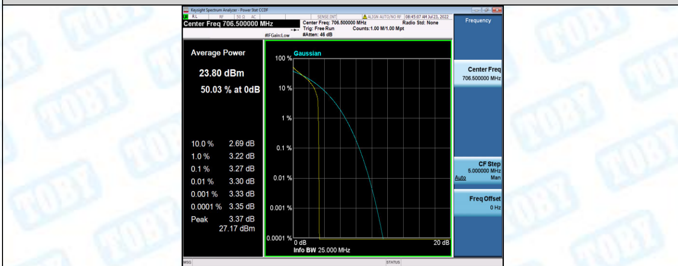
Band17-5MHz-QPSK-23755-25RB#0
