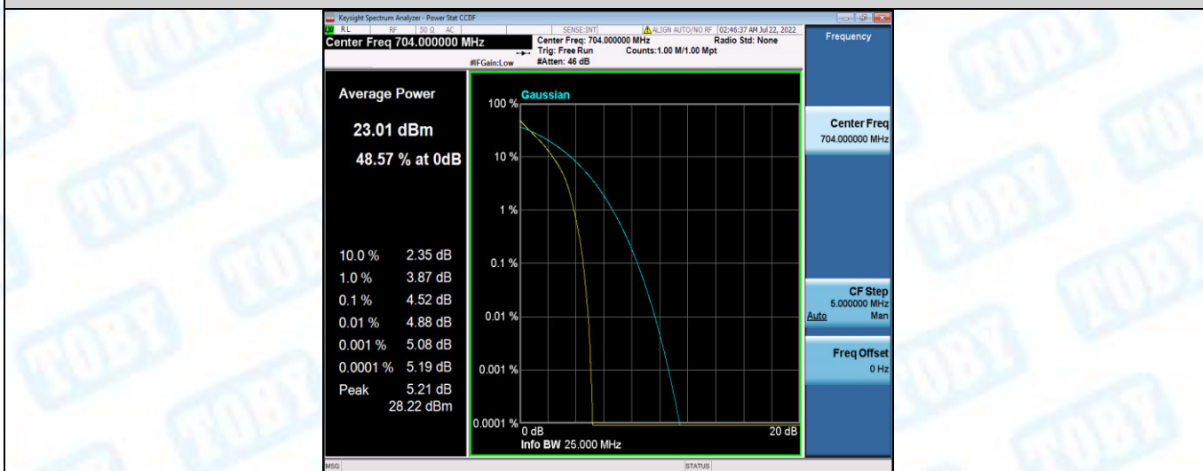
Band12-10MHz-QPSK-23095-1RB#0
