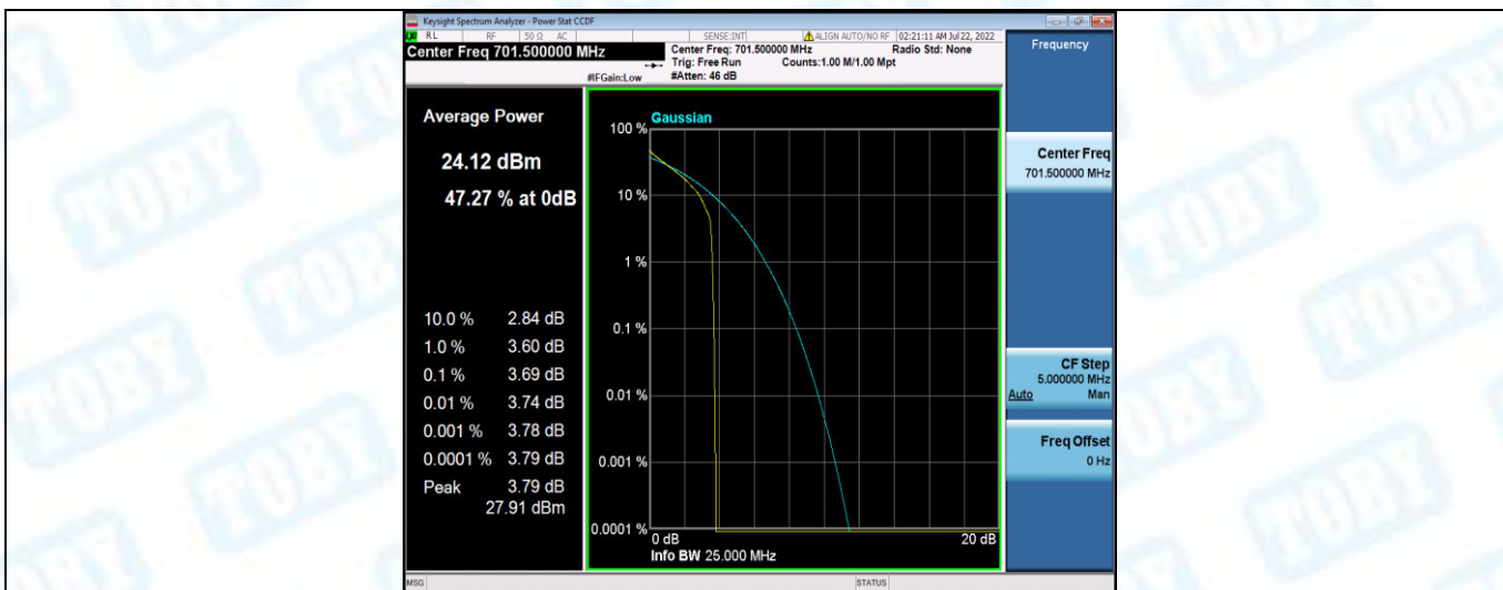
Band12-5MHz-QPSK-23035-25RB#0
