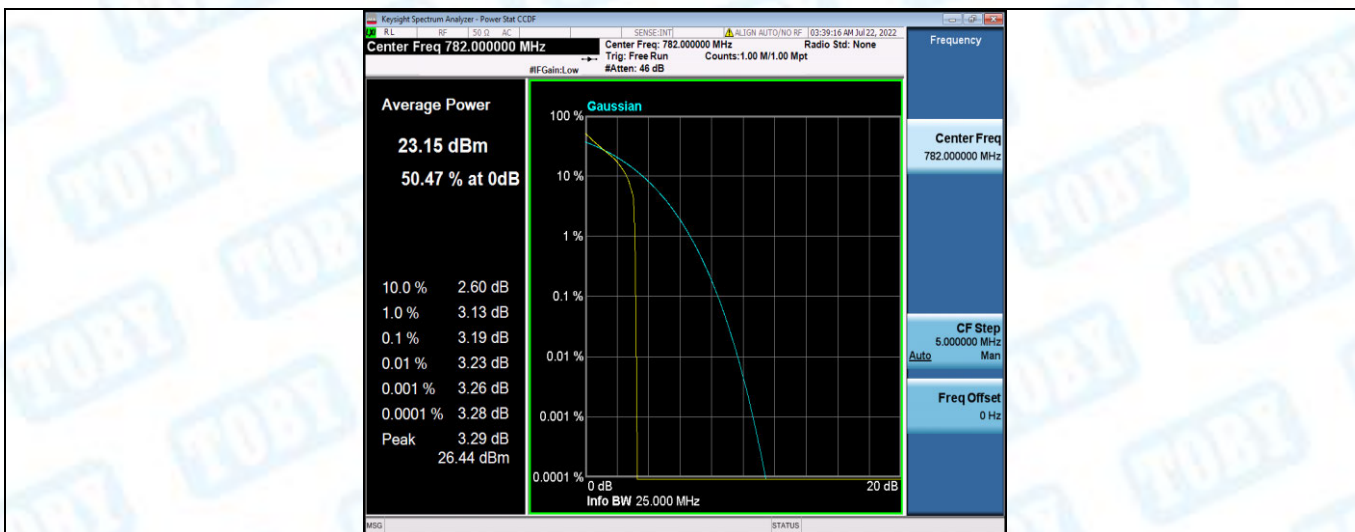
Band13-10MHz-QPSK-23230-50RB#0
