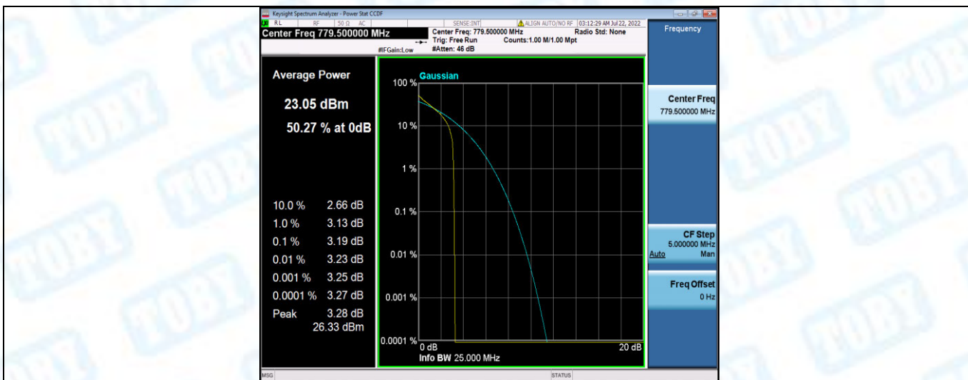
Band13-5MHz-QPSK-23205-25RB#0
