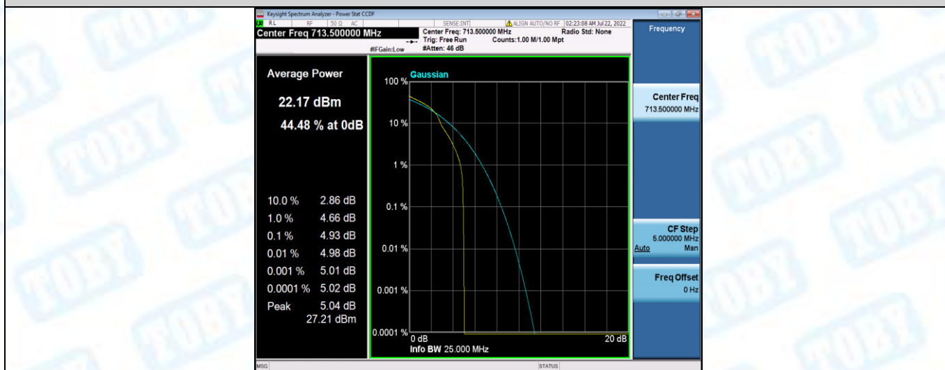
Band12-5MHz-16QAM-23155-25RB#0
