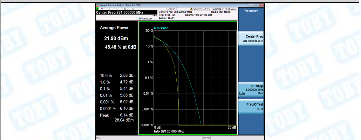
Band13-10MHz-QPSK-23230-1RB#0
